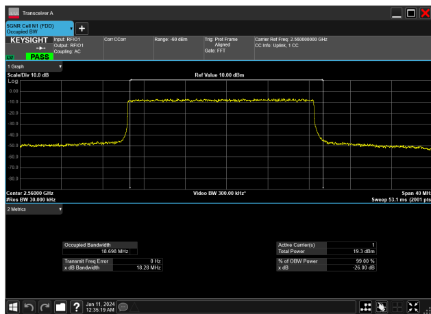
20MHz_15kHz_2560MHz_DFT-s-OFDM 256 QAM_RB100@0&amp;18.698 MHz
