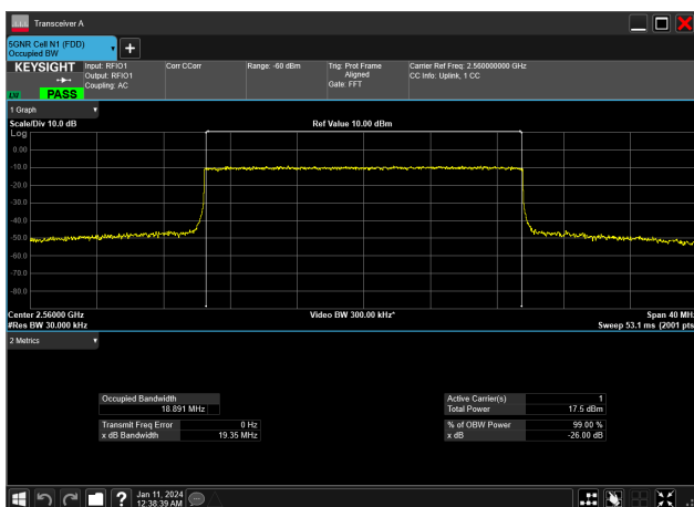
20MHz_15kHz_2560MHz_CP-OFDM 256 QAM_RB106@0&amp;18.891 MHz
