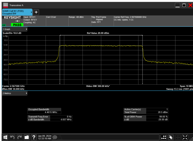
5MHz_15kHz_2567.5MHz_CP-OFDM 16 QAM_RB25@0&amp;4.461 MHz
