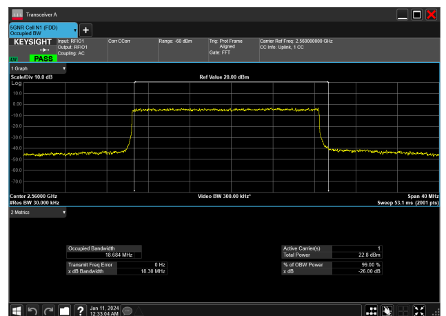
20MHz_15kHz_2560MHz_DFT-s-OFDM QPSK_RB100@0&amp;18.684 MHz
