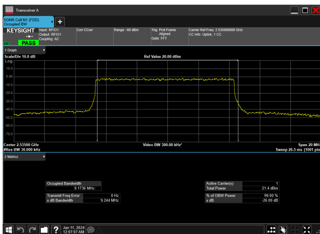
10MHz_15kHz_2535MHz_DFT-s-OFDM 16 QAM_RB50@0&amp;9.174 MHz
