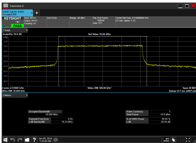
20MHz_15kHz_2510MHz_DFT-s-OFDM 256 QAM_RB100@0&amp;18.688 MHz
