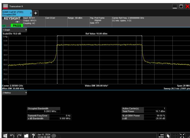
10MHz_15kHz_2505MHz_CP-OFDM 256 QAM_RB52@0&amp;9.280 MHz
