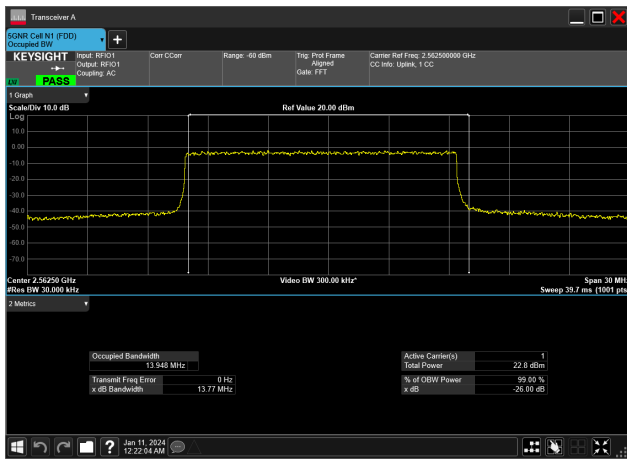
15MHz_15kHz_2562.5MHz_DFT-s-OFDM QPSK_RB75@0&13.948 MHz
