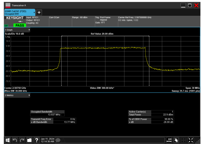
15MHz_15kHz_2507.5MHz_DFT-s-OFDM PI/2 BPSK_RB75@0&13.937 MHz
