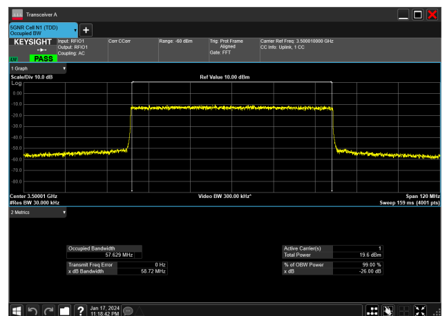
60MHz_30kHz_3500MHz_DFT-s-OFDM 256 QAM_RB162@0&amp;57.629 MHz
