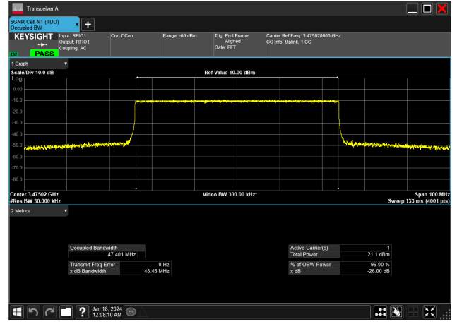
50MHz_30kHz_3475MHz_CP-OFDM QPSK_RB133@0&amp;47.401 MHz
