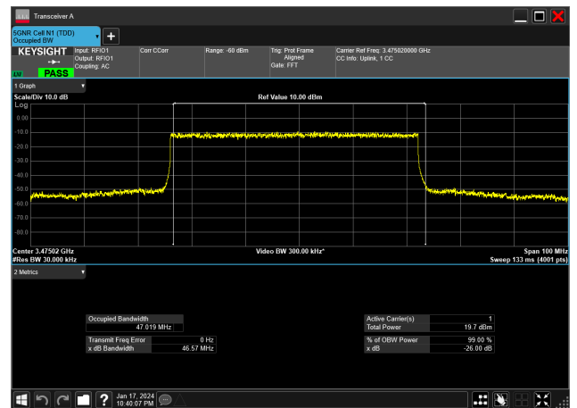
50MHz_30kHz_3475MHz_DFT-s-OFDM 256 QAM_RB128@0&amp;47.019 MHz
