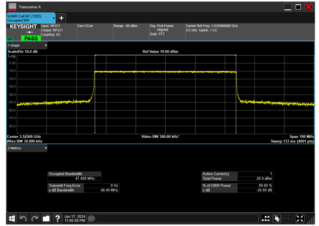
50MHz_30kHz_3525MHz_CP-OFDM QPSK_RB133@0&amp;47.408 MHz
