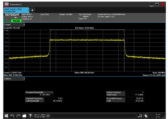
50MHz_30kHz_3525MHz_CP-OFDM 256 QAM_RB133@0&amp;47.362 MHz
