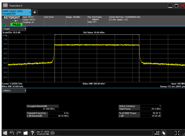
50MHz_30kHz_3525MHz_CP-OFDM 64 QAM_RB133@0&amp;47.408 MHz
