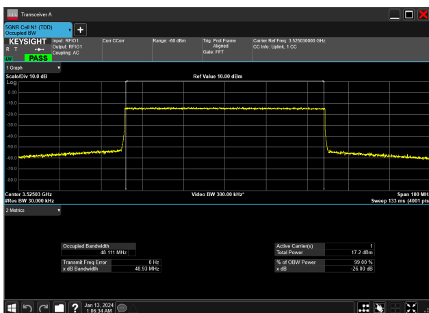
50MHz_15kHz_3525MHz_CP-OFDM 256 QAM_RB270@0&amp;48.111 MHz
