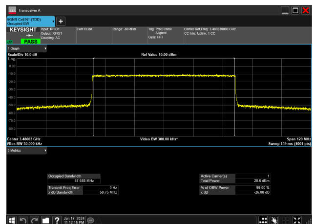
60MHz_30kHz_3480MHz_CP-OFDM 64 QAM_RB162@0&amp;57.688 MHz
