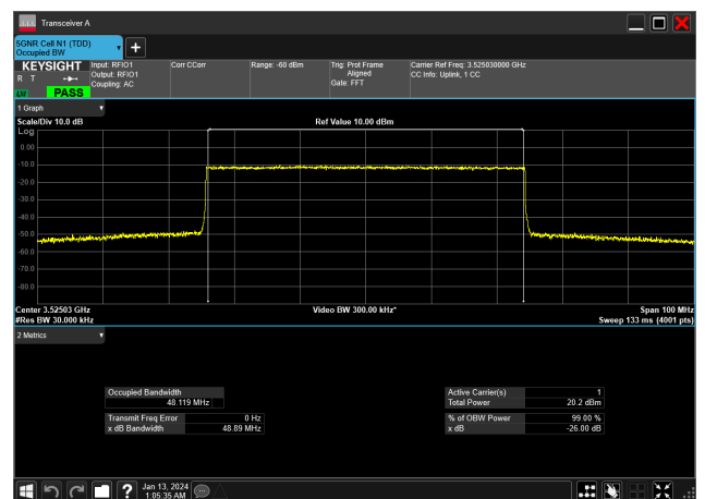
50MHz_15kHz_3525MHz_CP-OFDM 64 QAM_RB270@0&amp;48.119 MHz
