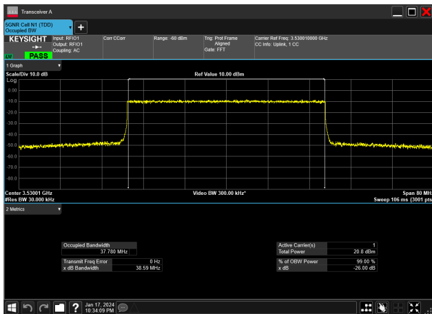
40MHz_30kHz_3530MHz_CP-OFDM 16 QAM_RB106@0&amp;37.780 MHz
