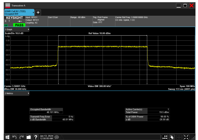
50MHz_15kHz_3500MHz_DFT-s-OFDM 256 QAM_RB270@0&amp;48.101 MHz
