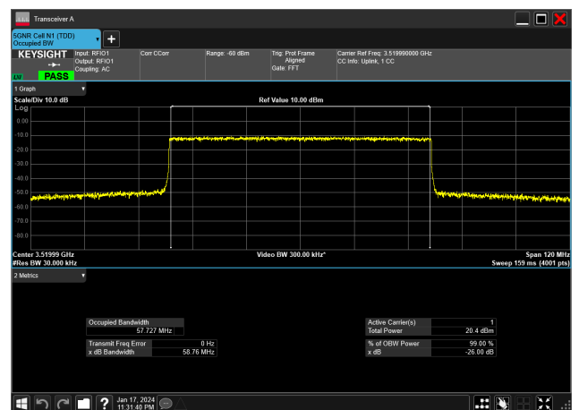
60MHz_30kHz_3520MHz_CP-OFDM 64 QAM_RB162@0&amp;57.727 MHz
