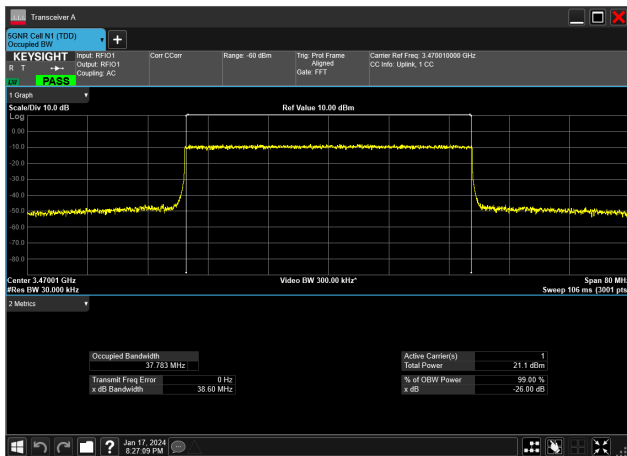
40MHz_30kHz_3470MHz_CP-OFDM 16 QAM_RB106@0&amp;37.783 MHz
