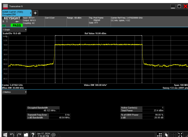
50MHz_15kHz_3475MHz_DFT-s-OFDM PI/2 BPSK_RB270@0&amp;48.123 MHz
