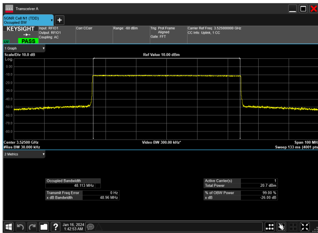
50MHz_15kHz_3525MHz_CP-OFDM QPSK_RB270@0&amp;48.113 MHz
