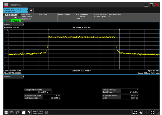
40MHz_30kHz_3500MHz_DFT-s-OFDM 64 QAM_RB100@0&amp;37.554 MHz
