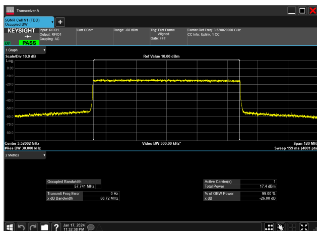
60MHz_30kHz_3520MHz_CP-OFDM 256 QAM_RB162@0&amp;57.741 MHz
