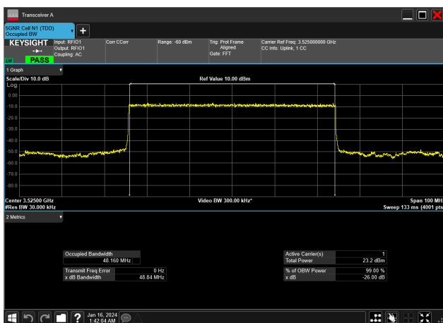
50MHz_15kHz_3525MHz_DFT-s-OFDM PI/2 BPSK_RB270@0&amp;48.160 MHz
