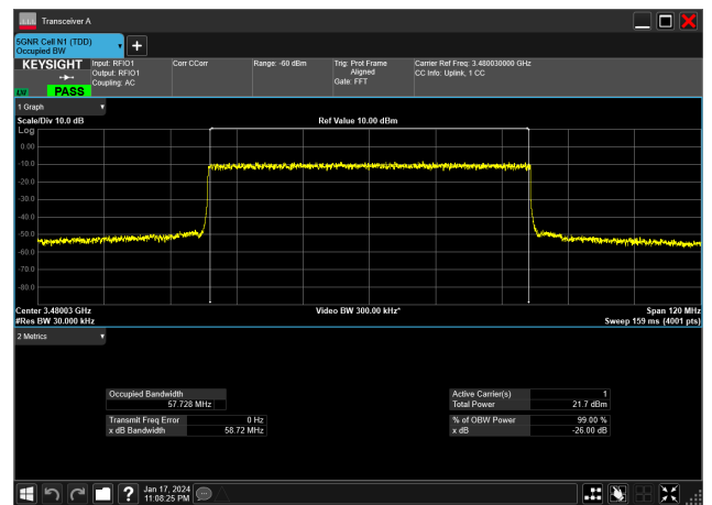
60MHz_30kHz_3480MHz_DFT-s-OFDM 64 QAM_RB162@0&amp;57.728 MHz
