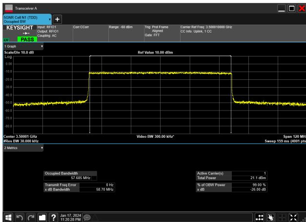
60MHz_30kHz_3500MHz_CP-OFDM 16 QAM_RB162@0&amp;57.685 MHz
