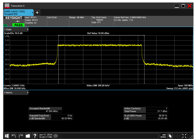
50MHz_30kHz_3500MHz_DFT-s-OFDM 64 QAM_RB128@0&amp;47.005 MHz
