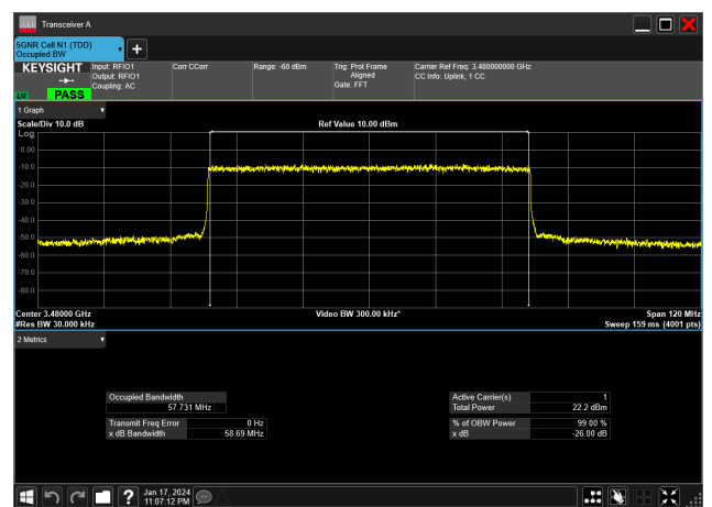
60MHz_30kHz_3480MHz_DFT-s-OFDM 16 QAM_RB162@0&amp;57.731 MHz
