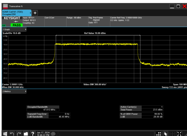
50MHz_30kHz_3500MHz_DFT-s-OFDM PI/2 BPSK_RB128@0&amp;47.013 MHz
