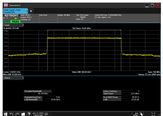
50MHz_15kHz_3525MHz_DFT-s-OFDM QPSK_RB270@0&amp;48.158 MHz
