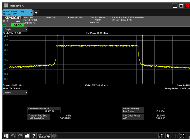
40MHz_30kHz_3500MHz_DFT-s-OFDM 256 QAM_RB100@0&amp;37.463 MHz
