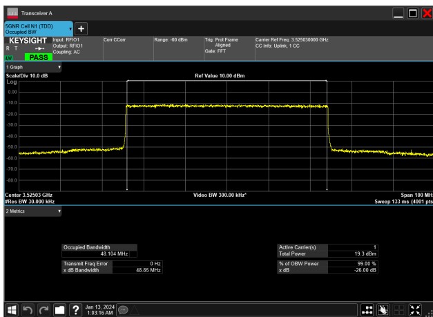
50MHz_15kHz_3525MHz_DFT-s-OFDM 256 QAM_RB270@0&amp;48.104 MHz
