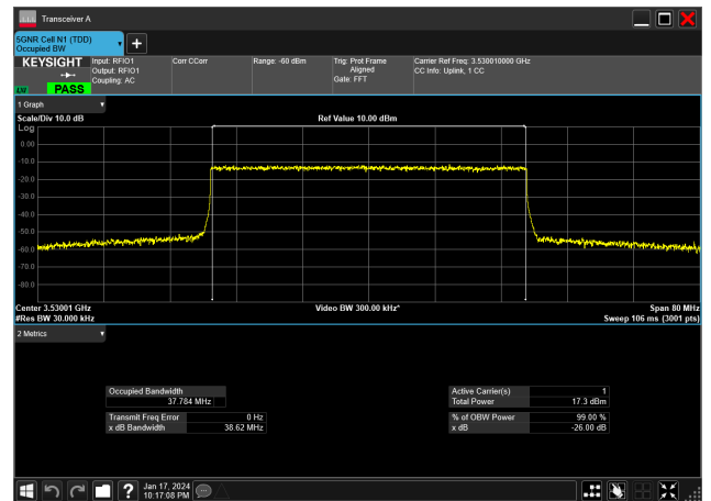
40MHz_30kHz_3530MHz_CP-OFDM 256 QAM_RB106@0&amp;37.784 MHz
