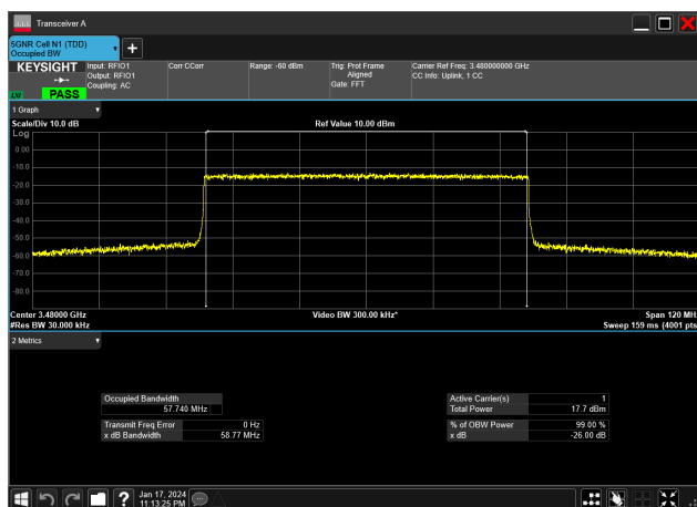
60MHz_30kHz_3480MHz_CP-OFDM 256 QAM_RB162@0&amp;57.740 MHz
