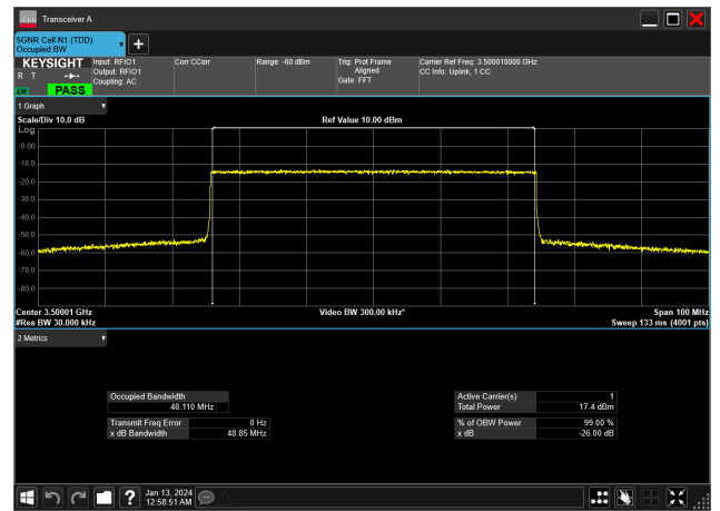
50MHz_15kHz_3500MHz_CP-OFDM 256 QAM_RB270@0&amp;48.110 MHz
