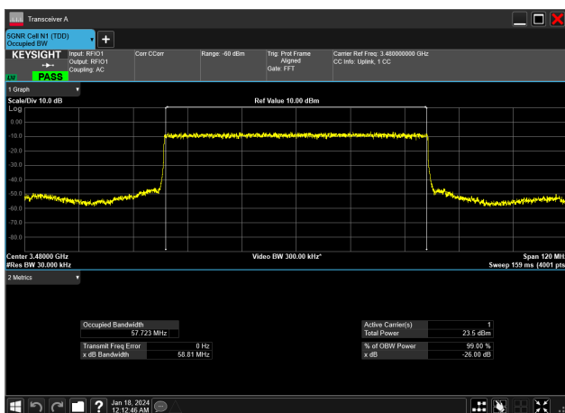
60MHz_30kHz_3480MHz_DFT-s-OFDM PI/2 BPSK_RB162@0&amp;57.723 MHz
