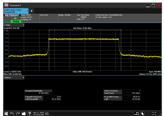
50MHz_30kHz_3525MHz_DFT-s-OFDM 256 QAM_RB128@0&amp;47.065 MHz
