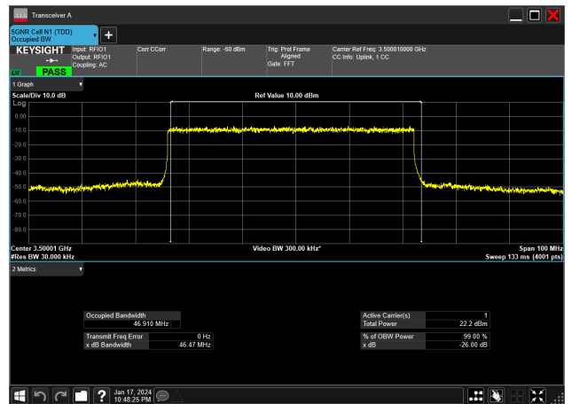
50MHz_30kHz_3500MHz_DFT-s-OFDM 16 QAM_RB128@0&amp;46.910 MHz
