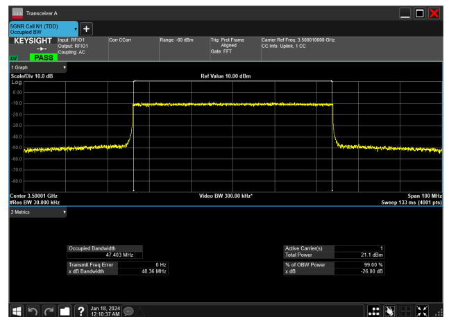
50MHz_30kHz_3500MHz_CP-OFDM 16 QAM_RB133@0&amp;47.403 MHz
