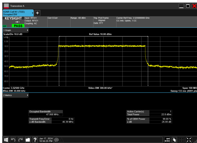
50MHz_30kHz_3525MHz_DFT-s-OFDM QPSK_RB128@0&amp;47.068 MHz
