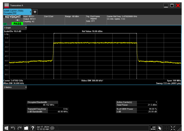
50MHz_15kHz_3475MHz_DFT-s-OFDM 64 QAM_RB270@0&amp;48.152 MHz
