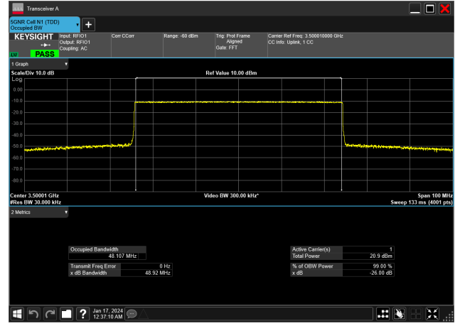
50MHz_15kHz_3500MHz_CP-OFDM QPSK_RB270@0&amp;48.107 MHz
