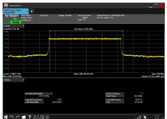
50MHz_30kHz_3500MHz_DFT-s-OFDM QPSK_RB128@0&amp;47.014 MHz
