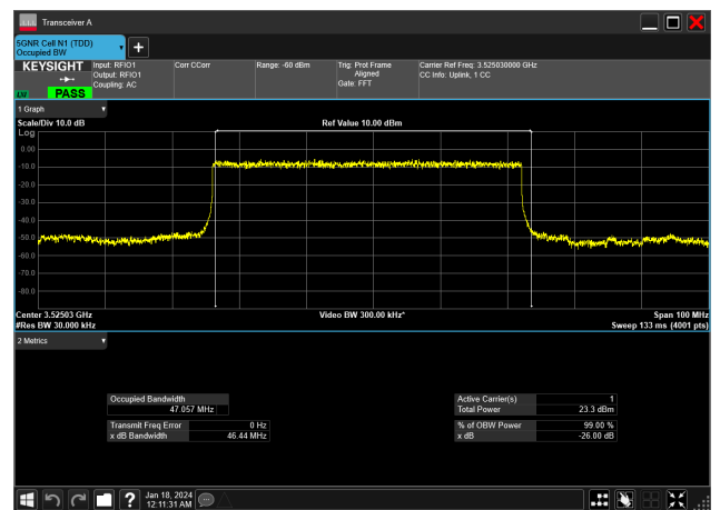
50MHz_30kHz_3525MHz_DFT-s-OFDM PI/2 BPSK_RB128@0&amp;47.057 MHz
