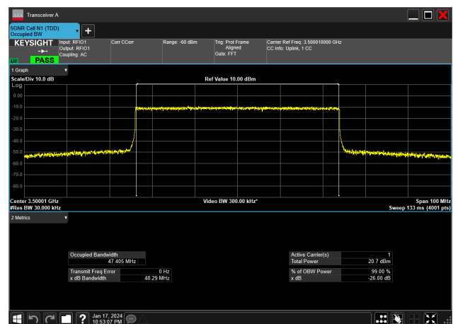
50MHz_30kHz_3500MHz_CP-OFDM 64 QAM_RB133@0&amp;47.405 MHz
