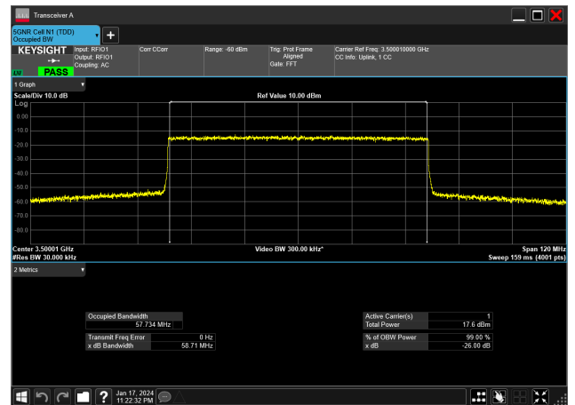
60MHz_30kHz_3500MHz_CP-OFDM 256 QAM_RB162@0&amp;57.734 MHz
