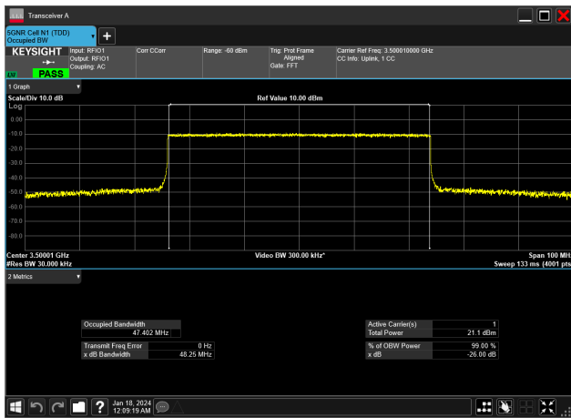
50MHz_30kHz_3500MHz_CP-OFDM QPSK_RB133@0&amp;47.402 MHz
