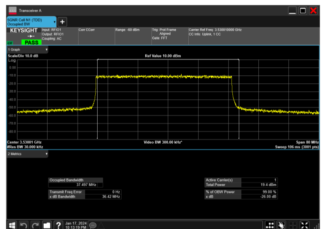
40MHz_30kHz_3530MHz_DFT-s-OFDM 256 QAM_RB100@0&amp;37.497 MHz
