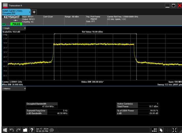
50MHz_30kHz_3500MHz_DFT-s-OFDM 256 QAM_RB128@0&amp;47.054 MHz
