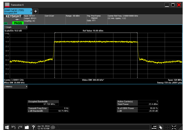
60MHz_30kHz_3500MHz_DFT-s-OFDM PI/2 BPSK_RB162@0&amp;57.720 MHz
