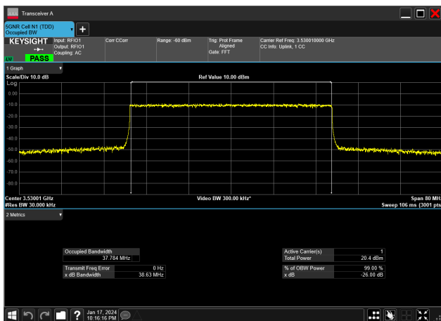
40MHz_30kHz_3530MHz_CP-OFDM 64 QAM_RB106@0&amp;37.784 MHz
