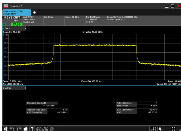
50MHz_30kHz_3500MHz_CP-OFDM 256 QAM_RB133@0&amp;47.352 MHz
