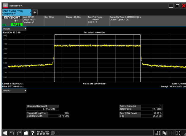
60MHz_30kHz_3480MHz_DFT-s-OFDM 256 QAM_RB162@0&amp;57.665 MHz
