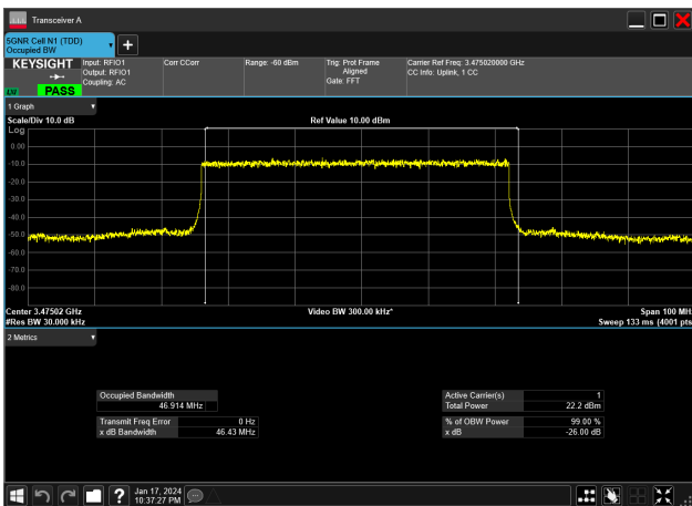
50MHz_30kHz_3475MHz_DFT-s-OFDM 16 QAM_RB128@0&amp;46.914 MHz
