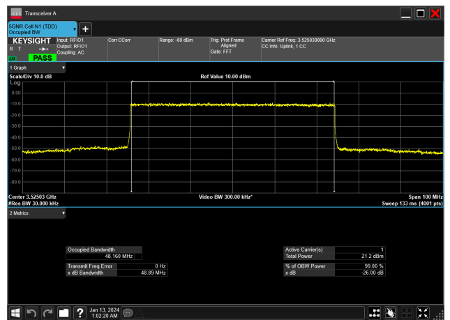
50MHz_15kHz_3525MHz_DFT-s-OFDM 64 QAM_RB270@0&amp;48.160 MHz
