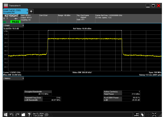
50MHz_15kHz_3525MHz_DFT-s-OFDM 16 QAM_RB270@0&amp;48.113 MHz
