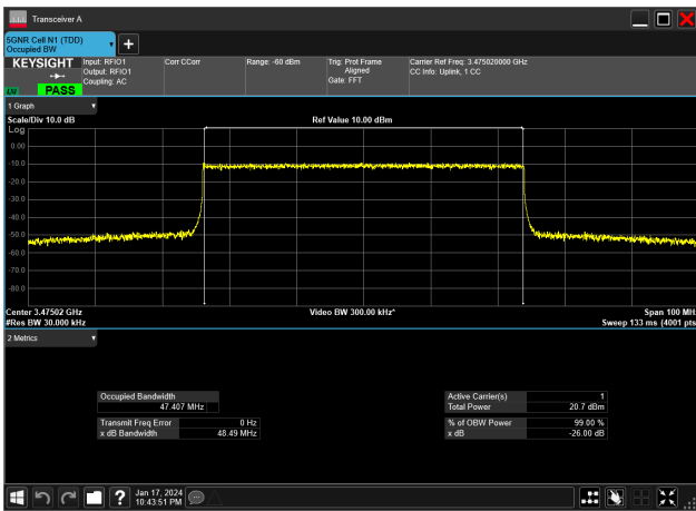
50MHz_30kHz_3475MHz_CP-OFDM 64 QAM_RB133@0&amp;47.407 MHz
