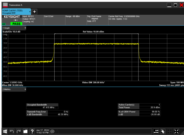
50MHz_30kHz_3525MHz_CP-OFDM 16 QAM_RB133@0&amp;47.415 MHz
