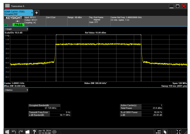
60MHz_30kHz_3480MHz_DFT-s-OFDM QPSK_RB162@0&amp;57.729 MHz
