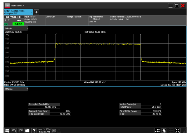
50MHz_15kHz_3525MHz_CP-OFDM 16 QAM_RB270@0&amp;48.117 MHz
