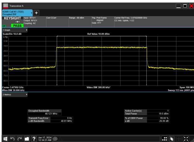
50MHz_15kHz_3475MHz_DFT-s-OFDM 256 QAM_RB270@0&amp;48.121 MHz
