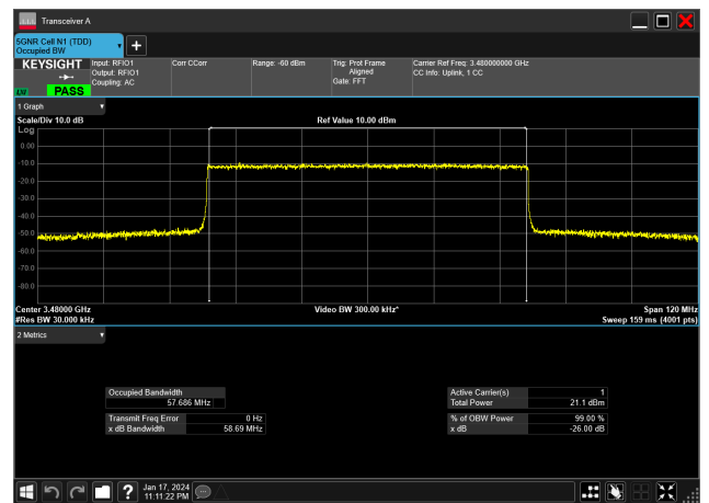
60MHz_30kHz_3480MHz_CP-OFDM 16 QAM_RB162@0&amp;57.686 MHz
