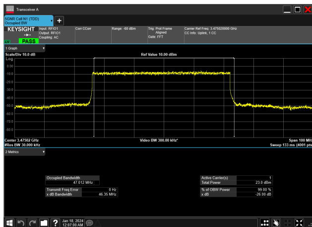
50MHz_30kHz_3475MHz_DFT-s-OFDM QPSK_RB128@0&amp;47.012 MHz
