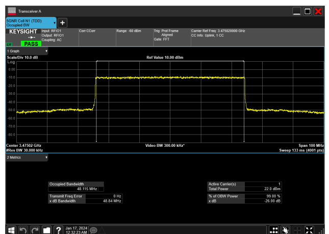
50MHz_15kHz_3475MHz_DFT-s-OFDM 16 QAM_RB270@0&amp;48.115 MHz
