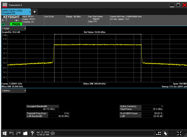
50MHz_15kHz_3500MHz_CP-OFDM 64 QAM_RB270@0&amp;48.115 MHz
