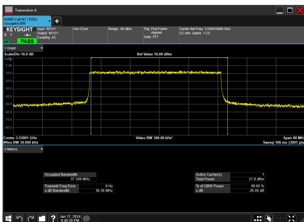
40MHz_30kHz_3530MHz_DFT-s-OFDM 16 QAM_RB100@0&amp;37.349 MHz
