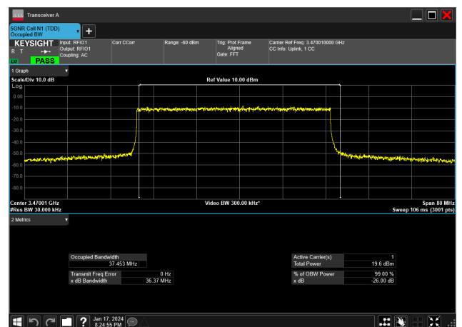
40MHz_30kHz_3470MHz_DFT-s-OFDM 256 QAM_RB100@0&amp;37.453 MHz
