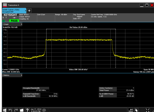
40MHz_30kHz_3500MHz_DFT-s-OFDM PI/2 BPSK_RB100@0&amp;37.563 MHz
