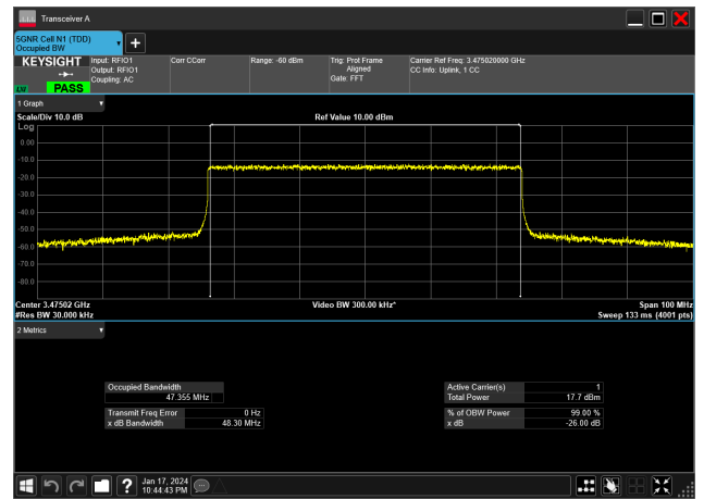
50MHz_30kHz_3475MHz_CP-OFDM 256 QAM_RB133@0&amp;47.355 MHz
