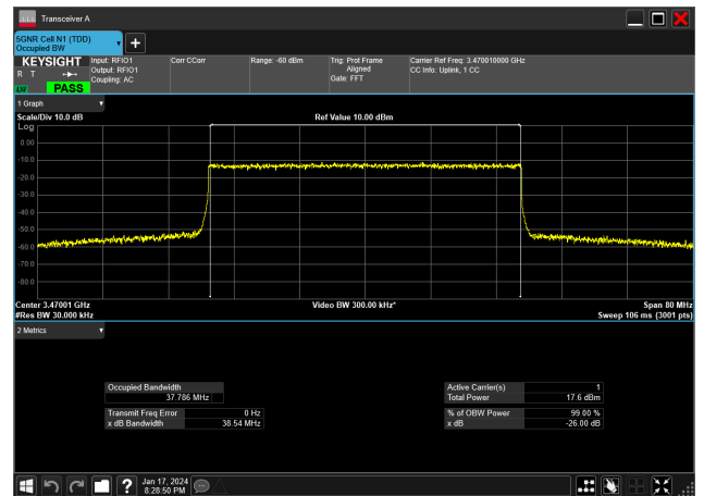
40MHz_30kHz_3470MHz_CP-OFDM 256 QAM_RB106@0&amp;37.786 MHz
