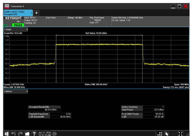
50MHz_15kHz_3475MHz_DFT-s-OFDM QPSK_RB270@0&amp;48.074 MHz
