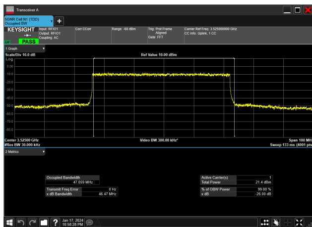
50MHz_30kHz_3525MHz_DFT-s-OFDM 64 QAM_RB128@0&amp;47.059 MHz
