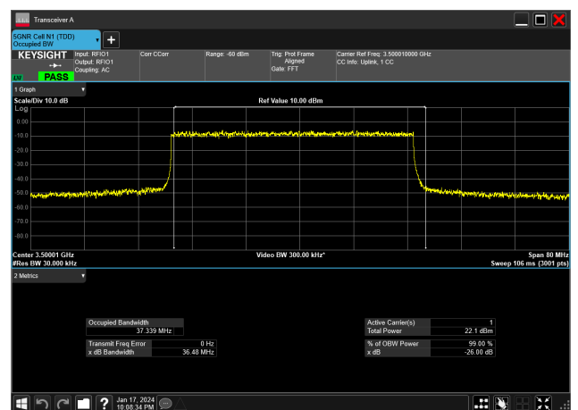
40MHz_30kHz_3500MHz_DFT-s-OFDM 16 QAM_RB100@0&amp;37.339 MHz
