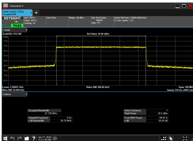
60MHz_30kHz_3500MHz_CP-OFDM 64 QAM_RB162@0&amp;57.720 MHz
