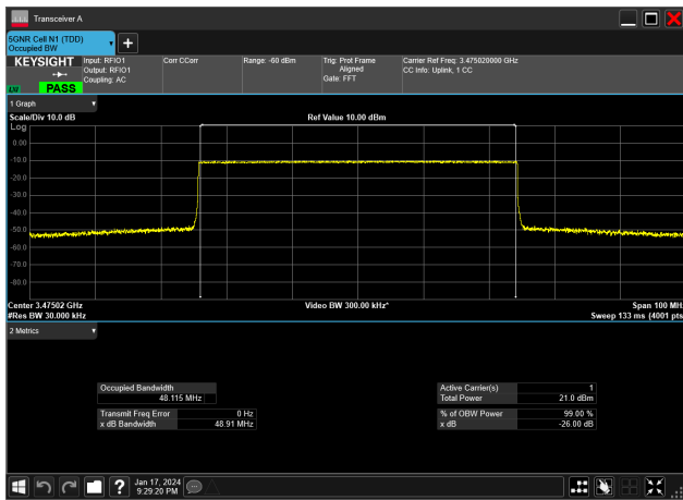
50MHz_15kHz_3475MHz_CP-OFDM QPSK_RB270@0&amp;48.115 MHz
