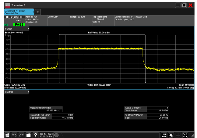
50MHz_30kHz_3475MHz_DFT-s-OFDM PI/2 BPSK_RB128@0&amp;47.020 MHz
