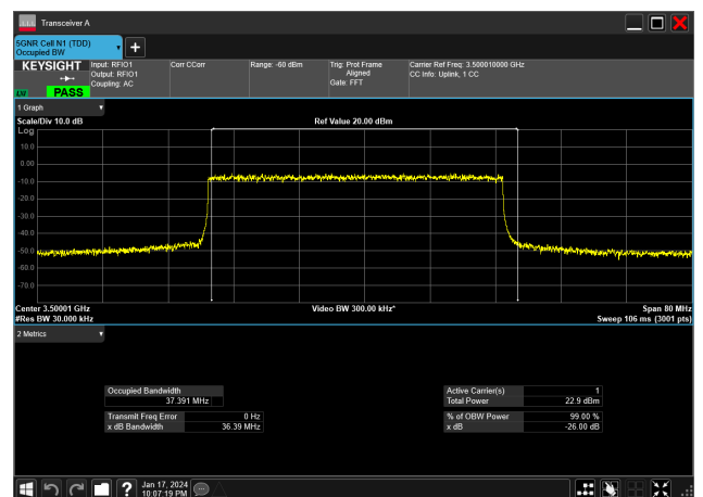
40MHz_30kHz_3500MHz_DFT-s-OFDM QPSK_RB100@0&amp;37.391 MHz
