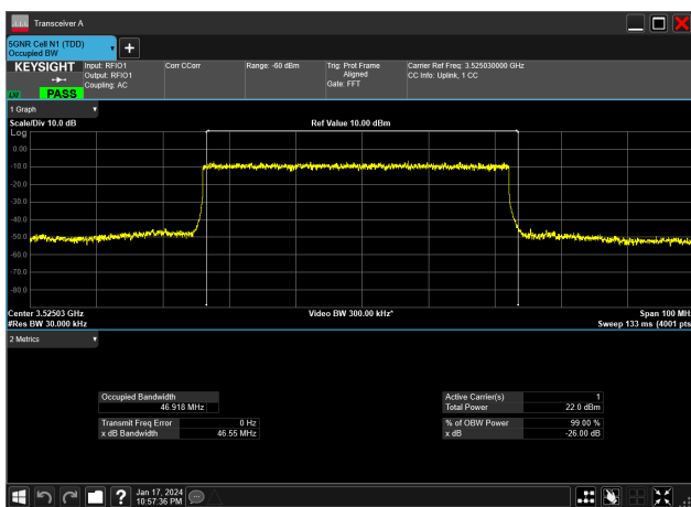
50MHz_30kHz_3525MHz_DFT-s-OFDM 16 QAM_RB128@0&amp;46.918 MHz
