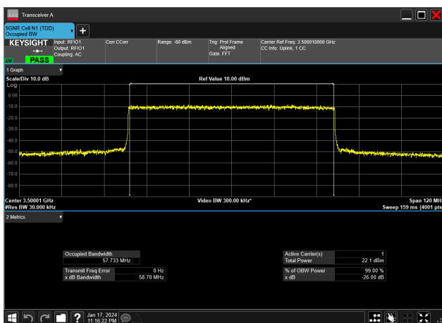
60MHz_30kHz_3500MHz_DFT-s-OFDM 16 QAM_RB162@0&amp;57.733 MHz
