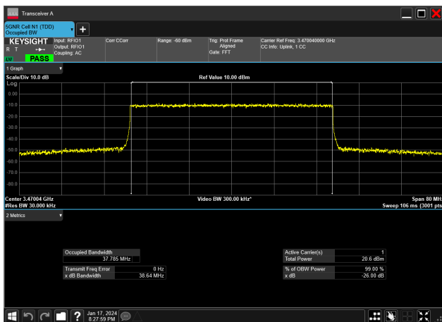
40MHz_30kHz_3470MHz_CP-OFDM 64 QAM_RB106@0&amp;37.785 MHz
