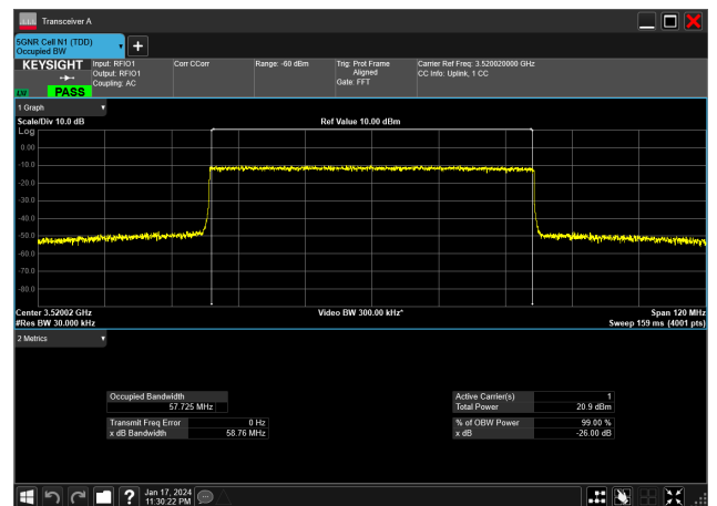
60MHz_30kHz_3520MHz_CP-OFDM 16 QAM_RB162@0&amp;57.725 MHz
