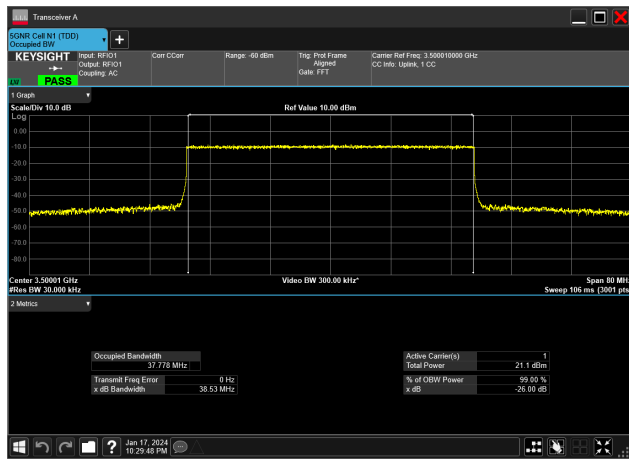
40MHz_30kHz_3500MHz_CP-OFDM QPSK_RB106@0&amp;37.778 MHz
