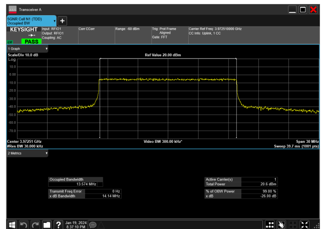
15MHz_30kHz_3972.5MHz_CP-OFDM 16 QAM_RB38@0&amp;13.574 MHz
