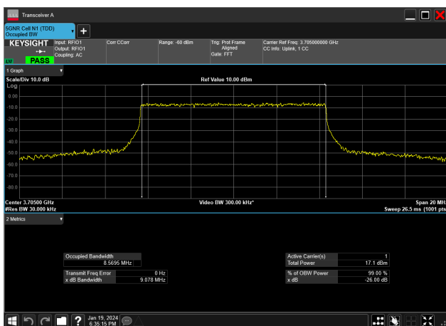
10MHz_30kHz_3705MHz_CP-OFDM 256 QAM_RB24@0&amp;8.570 MHz
