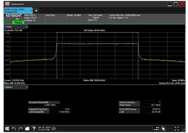
10MHz_15kHz_3840MHz_CP-OFDM 16 QAM_RB52@0&amp;9.286 MHz
