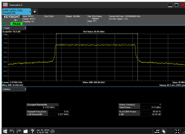
10MHz_15kHz_3975MHz_DFT-s-OFDM 64 QAM_RB50@0&amp;9.178 MHz
