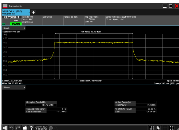
15MHz_30kHz_3972.5MHz_CP-OFDM 256 QAM_RB38@0&amp;13.575 MHz
