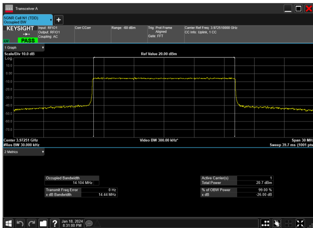
15MHz_15kHz_3972.5MHz_CP-OFDM 16 QAM_RB79@0&amp;14.104 MHz
