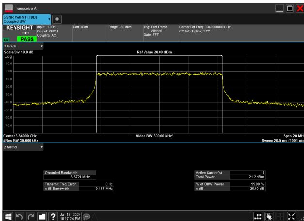
10MHz_30kHz_3840MHz_DFT-s-OFDM 64 QAM_RB24@0&amp;8.572 MHz
