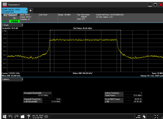
15MHz_30kHz_3972.5MHz_DFT-s-OFDM PI/2 BPSK_RB36@0&amp;13.511 MHz
