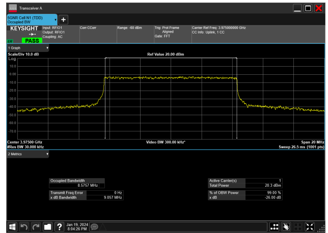
10MHz_30kHz_3975MHz_CP-OFDM 64 QAM_RB24@0&amp;8.576 MHz
