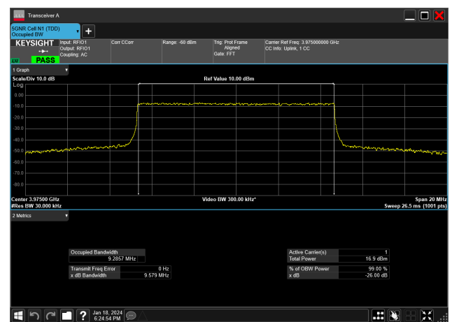
10MHz_15kHz_3975MHz_CP-OFDM 256 QAM_RB52@0&amp;9.286 MHz
