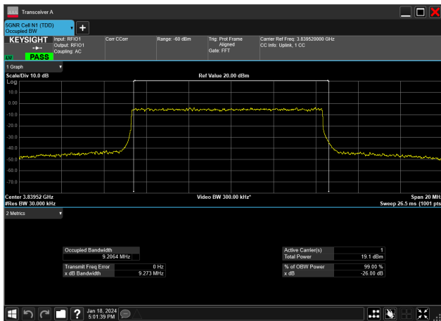
10MHz_15kHz_3840MHz_DFT-s-OFDM 256 QAM_RB50@0&amp;9.206 MHz
