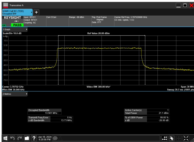
15MHz_15kHz_3707.5MHz_DFT-s-OFDM 64 QAM_RB75@0&13.981 MHz
