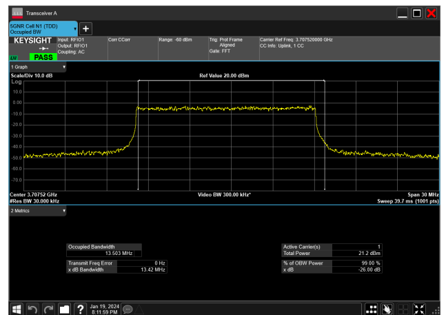
15MHz_30kHz_3707.5MHz_DFT-s-OFDM 64 QAM_RB36@0&amp;13.503 MHz
