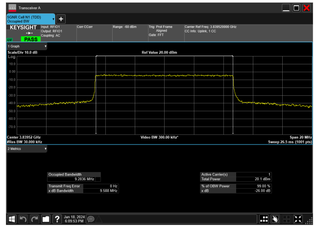
10MHz_15kHz_3840MHz_CP-OFDM 64 QAM_RB52@0&amp;9.284 MHz
