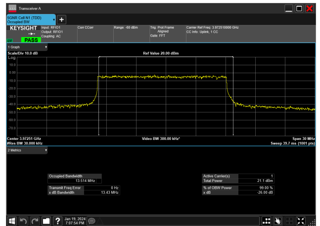
15MHz_30kHz_3972.5MHz_DFT-s-OFDM 64 QAM_RB36@0&amp;13.514 MHz
