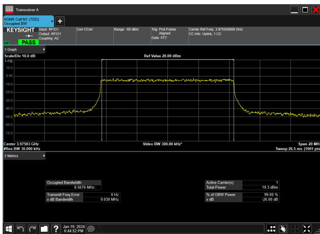
10MHz_30kHz_3975MHz_DFT-s-OFDM 256 QAM_RB24@0&amp;8.568 MHz
