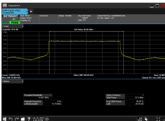
15MHz_15kHz_3840MHz_DFT-s-OFDM PI/2 BPSK_RB75@0&amp;14.001 MHz
