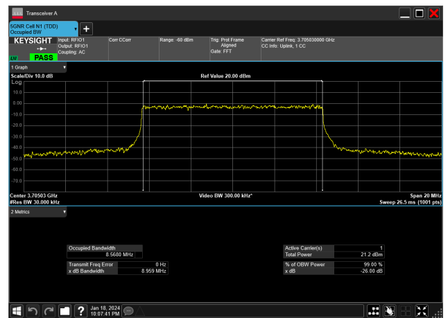
10MHz_30kHz_3705MHz_DFT-s-OFDM 64 QAM_RB24@0&amp;8.568 MHz
