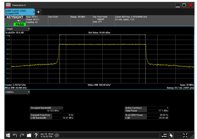
15MHz_15kHz_3707.5MHz_CP-OFDM 256 QAM_RB79@0&amp;14.103 MHz
