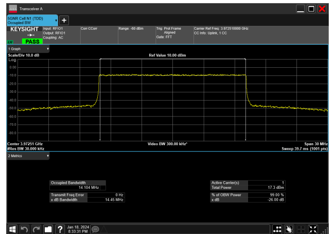
15MHz_15kHz_3972.5MHz_CP-OFDM 256 QAM_RB79@0&amp;14.104 MHz
