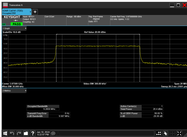
10MHz_15kHz_3975MHz_CP-OFDM 16 QAM_RB52@0&amp;9.286 MHz
