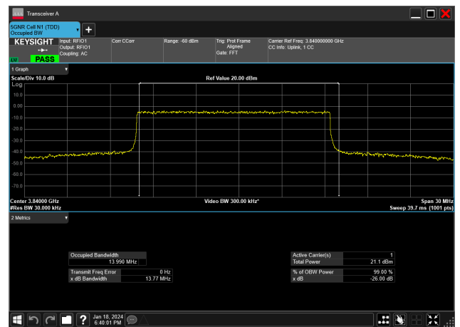
15MHz_15kHz_3840MHz_DFT-s-OFDM 64 QAM_RB75@0&amp;13.990 MHz
