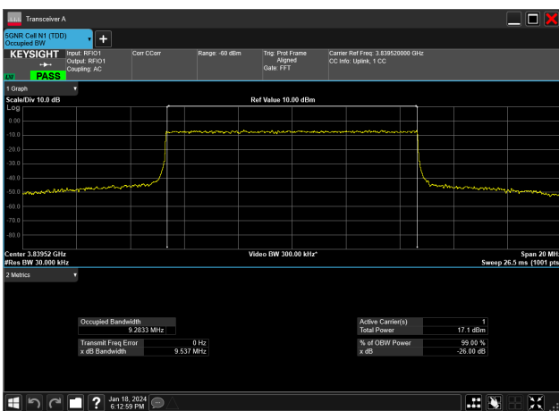
10MHz_15kHz_3840MHz_CP-OFDM 256 QAM_RB52@0&amp;9.283 MHz
