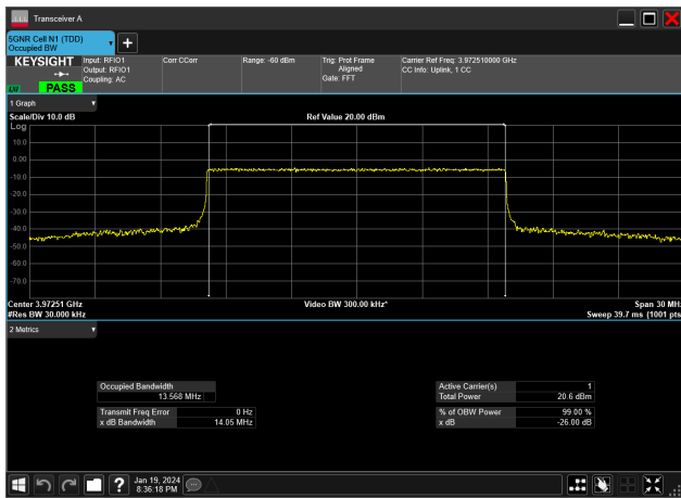
15MHz_30kHz_3972.5MHz_CP-OFDM QPSK_RB38@0&amp;13.568 MHz
