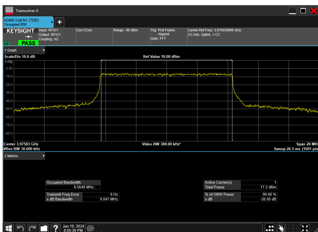
10MHz_30kHz_3975MHz_CP-OFDM 256 QAM_RB24@0&amp;8.565 MHz
