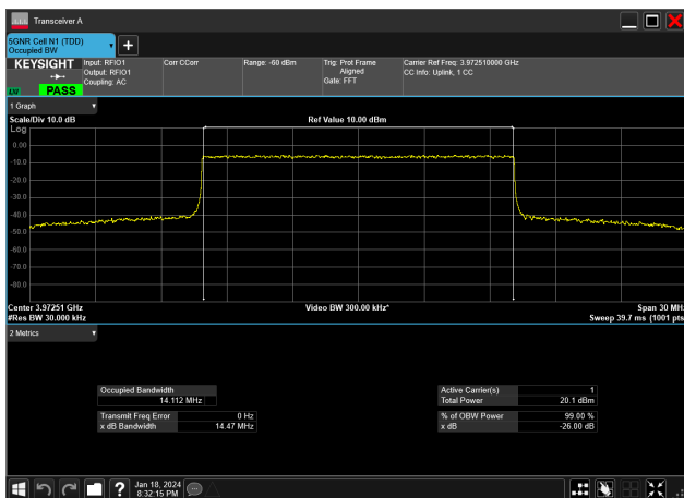
15MHz_15kHz_3972.5MHz_CP-OFDM 64 QAM_RB79@0&amp;14.112 MHz
