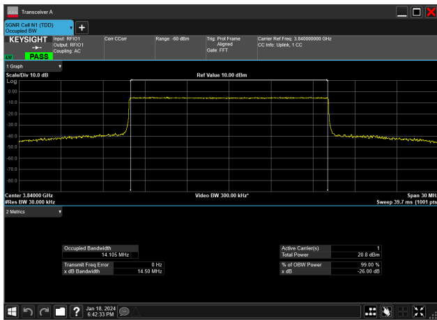
15MHz_15kHz_3840MHz_CP-OFDM QPSK_RB79@0&amp;14.105 MHz
