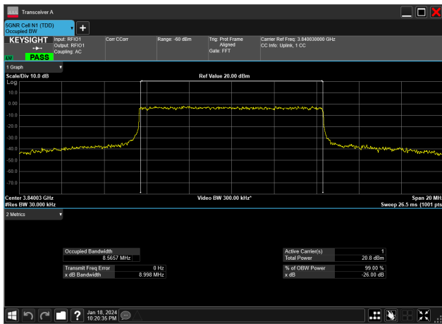
10MHz_30kHz_3840MHz_CP-OFDM 16 QAM_RB24@0&amp;8.566 MHz
