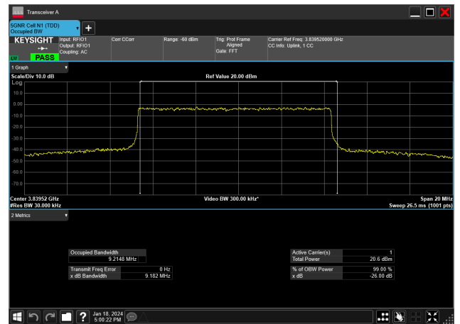
10MHz_15kHz_3840MHz_DFT-s-OFDM 64 QAM_RB50@0&amp;9.215 MHz
