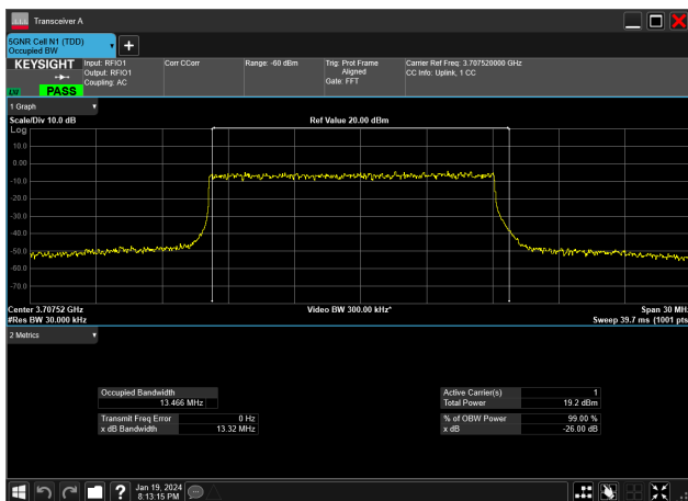
15MHz_30kHz_3707.5MHz_DFT-s-OFDM 256 QAM_RB36@0&amp;13.466 MHz
