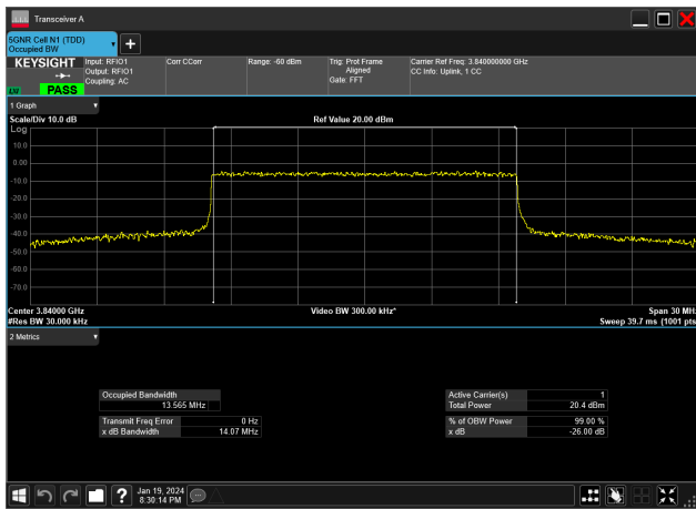
15MHz_30kHz_3840MHz_CP-OFDM 64 QAM_RB38@0&amp;13.565 MHz
