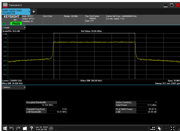
15MHz_15kHz_3840MHz_CP-OFDM 256 QAM_RB79@0&14.104 MHz
