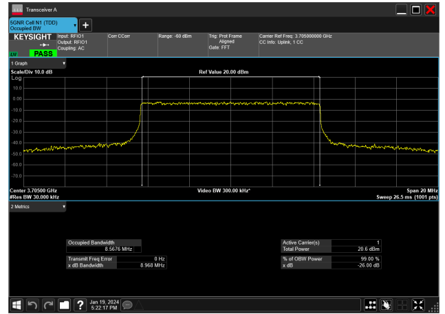
10MHz_30kHz_3705MHz_CP-OFDM 16 QAM_RB24@0&amp;8.568 MHz
