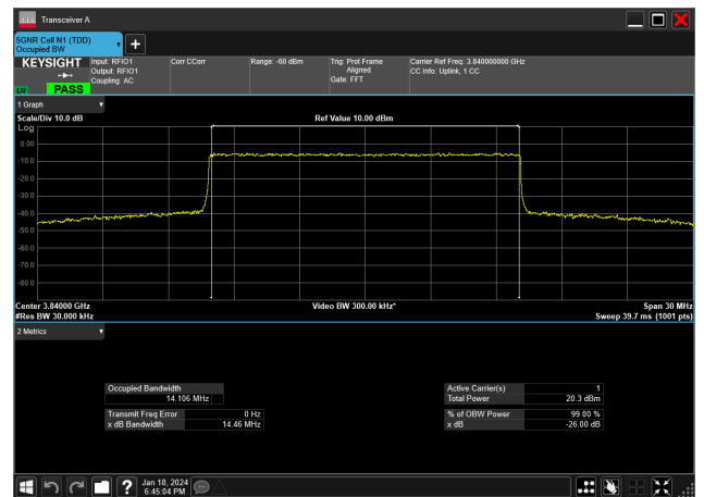
15MHz_15kHz_3840MHz_CP-OFDM 64 QAM_RB79@0&14.106 MHz
