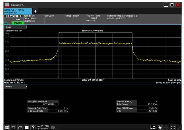
10MHz_30kHz_3975MHz_DFT-s-OFDM 16 QAM_RB24@0&amp;8.574 MHz
