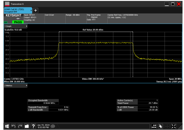
10MHz_30kHz_3975MHz_CP-OFDM 16 QAM_RB24@0&amp;8.564 MHz
