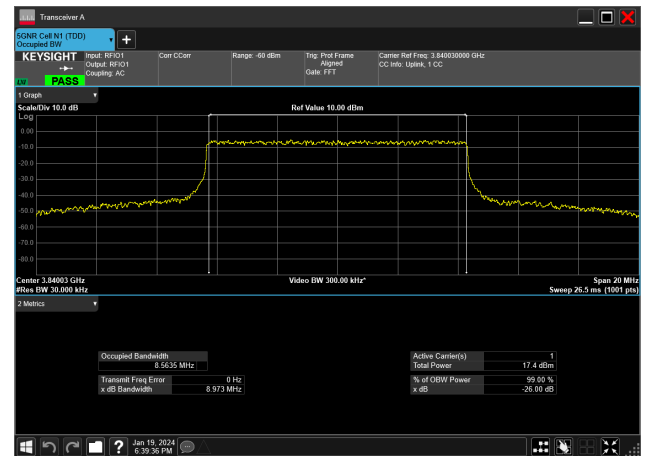
10MHz_30kHz_3840MHz_CP-OFDM 256 QAM_RB24@0&amp;8.564 MHz
