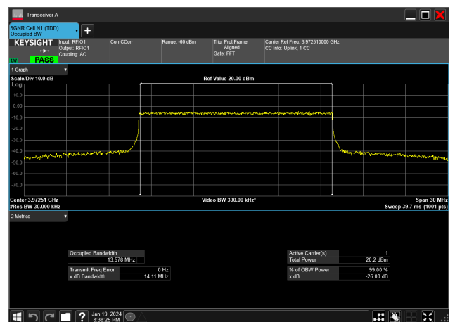
15MHz_30kHz_3972.5MHz_CP-OFDM 64 QAM_RB38@0&amp;13.578 MHz
