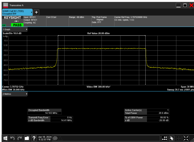
15MHz_15kHz_3707.5MHz_CP-OFDM 16 QAM_RB79@0&amp;14.103 MHz
