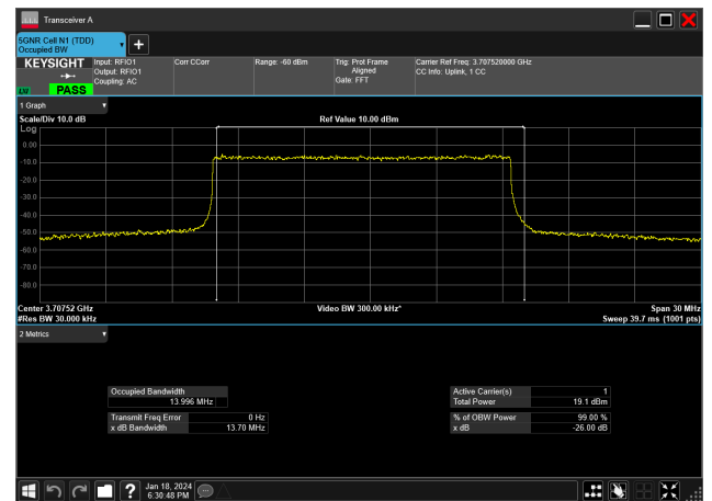
15MHz_15kHz_3707.5MHz_DFT-s-OFDM 256 QAM_RB75@0&amp;13.996 MHz
