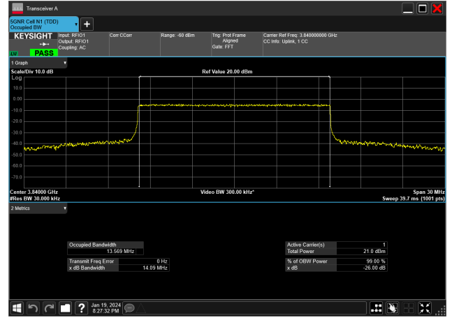
15MHz_30kHz_3840MHz_CP-OFDM QPSK_RB38@0&amp;13.569 MHz
