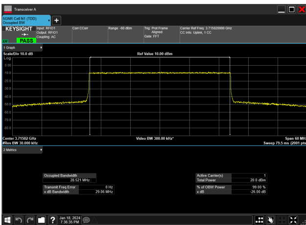
30MHz_15kHz_3715MHz_CP-OFDM 64 QAM_RB160@0&amp;28.521 MHz
