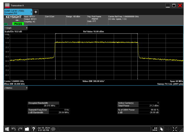
30MHz_15kHz_3840MHz_DFT-s-OFDM 64 QAM_RB160@0&amp;28.515 MHz
