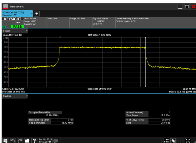
20MHz_30kHz_3970MHz_CP-OFDM 256 QAM_RB51@0&amp;18.174 MHz
