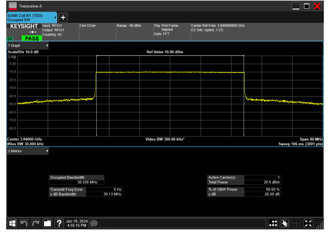
40MHz_15kHz_3840MHz_CP-OFDM QPSK_RB216@0&amp;38.508 MHz
