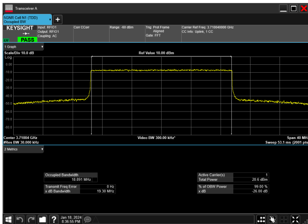
20MHz_15kHz_3710MHz_CP-OFDM 16 QAM_RB106@0&amp;18.891 MHz
