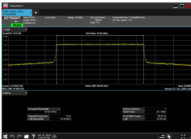
20MHz_15kHz_3710MHz_CP-OFDM 64 QAM_RB106@0&amp;18.921 MHz
