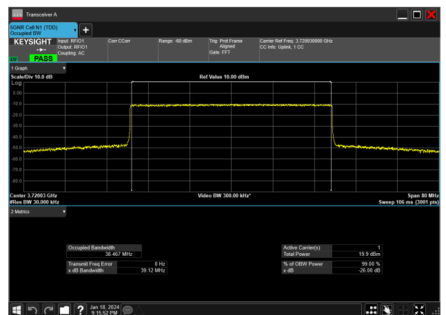
40MHz_15kHz_3720MHz_CP-OFDM 64 QAM_RB216@0&amp;38.467 MHz
