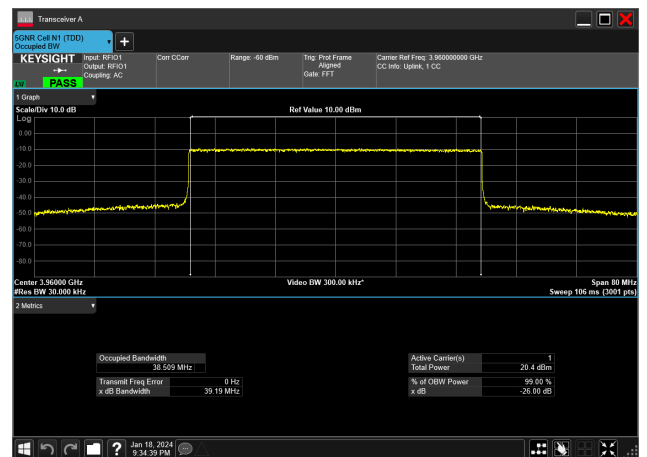
40MHz_15kHz_3960MHz_CP-OFDM 16 QAM_RB216@0&amp;38.509 MHz
