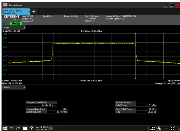
30MHz_15kHz_3840MHz_CP-OFDM 256 QAM_RB160@0&amp;28.517 MHz
