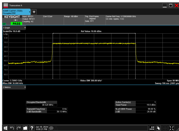
40MHz_15kHz_3720MHz_DFT-s-OFDM 256 QAM_RB216@0&amp;38.520 MHz
