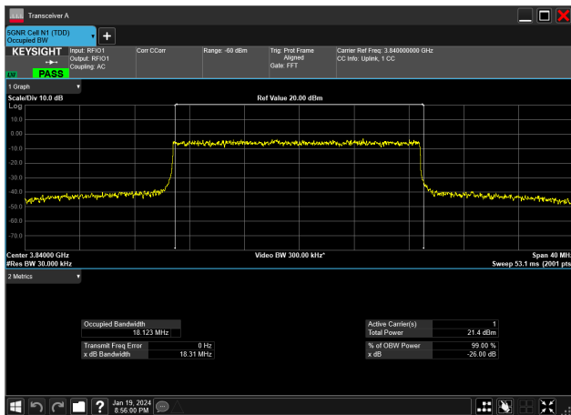
20MHz_30kHz_3840MHz_DFT-s-OFDM 64 QAM_RB50@0&amp;18.123 MHz
