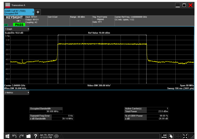
40MHz_15kHz_3840MHz_DFT-s-OFDM PI/2 BPSK_RB216@0&amp;38.508 MHz
