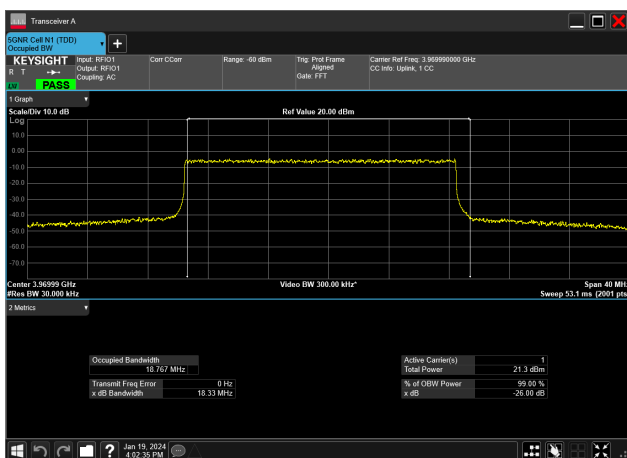
20MHz_15kHz_3970MHz_DFT-s-OFDM 16 QAM_RB100@0&amp;18.767 MHz
