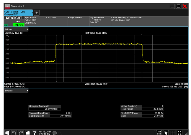
40MHz_15kHz_3720MHz_DFT-s-OFDM QPSK_RB216@0&amp;38.509 MHz
