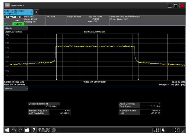
20MHz_15kHz_3840MHz_DFT-s-OFDM 64 QAM_RB100@0&amp;18.740 MHz
