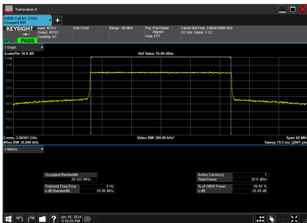
30MHz_15kHz_3965MHz_CP-OFDM 64 QAM_RB160@0&amp;28.522 MHz
