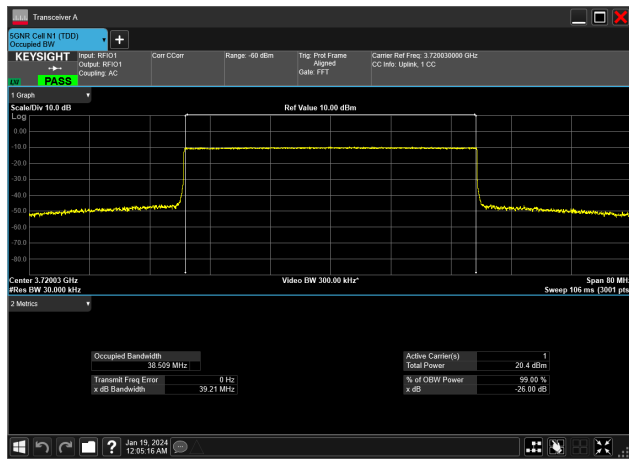
40MHz_15kHz_3720MHz_CP-OFDM QPSK_RB216@0&amp;38.509 MHz
