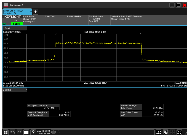
30MHz_15kHz_3965MHz_DFT-s-OFDM 64 QAM_RB160@0&amp;28.521 MHz
