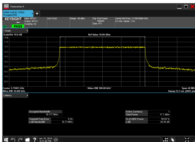
20MHz_30kHz_3710MHz_CP-OFDM 256 QAM_RB51@0&amp;18.177 MHz
