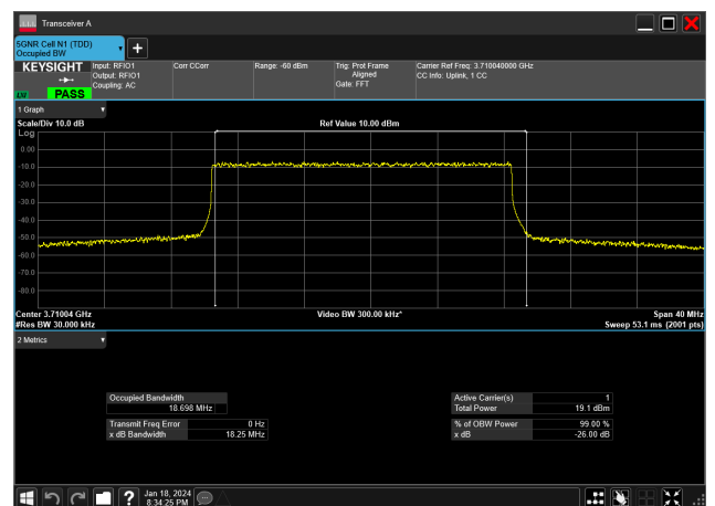
20MHz_15kHz_3710MHz_DFT-s-OFDM 256 QAM_RB100@0&amp;18.698 MHz
