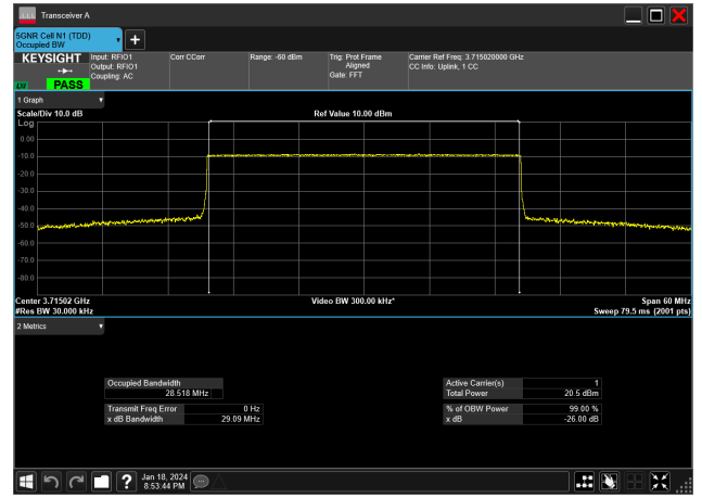
30MHz_15kHz_3715MHz_CP-OFDM QPSK_RB160@0&amp;28.518 MHz
