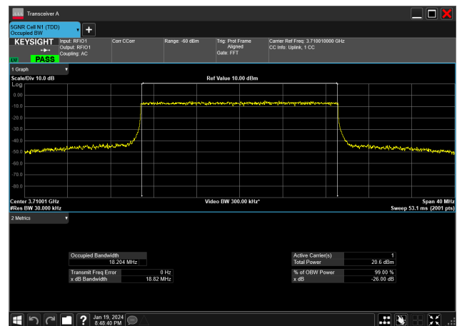
20MHz_30kHz_3710MHz_CP-OFDM 16 QAM_RB51@0&amp;18.204 MHz
