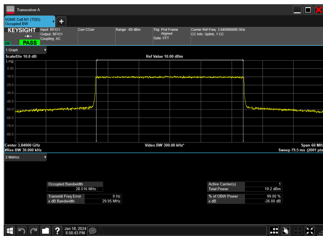
30MHz_15kHz_3840MHz_DFT-s-OFDM 256 QAM_RB160@0&amp;28.516 MHz
