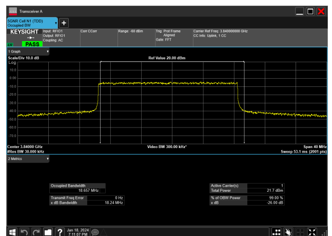
20MHz_15kHz_3840MHz_DFT-s-OFDM 16 QAM_RB100@0&amp;18.657 MHz
