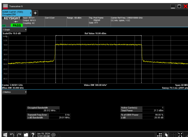
30MHz_15kHz_3965MHz_DFT-s-OFDM 16 QAM_RB160@0&amp;28.512 MHz
