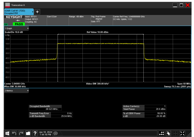
30MHz_15kHz_3840MHz_CP-OFDM 16 QAM_RB160@0&amp;28.523 MHz
