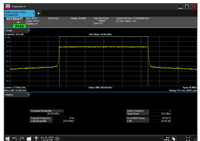
30MHz_15kHz_3715MHz_DFT-s-OFDM 256 QAM_RB160@0&amp;28.505 MHz
