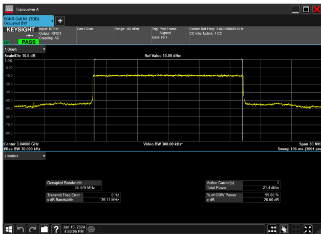
40MHz_15kHz_3840MHz_DFT-s-OFDM 16 QAM_RB216@0&amp;38.479 MHz
