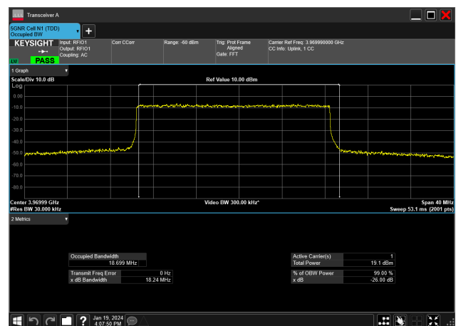
20MHz_15kHz_3970MHz_DFT-s-OFDM 256 QAM_RB100@0&amp;18.699 MHz
