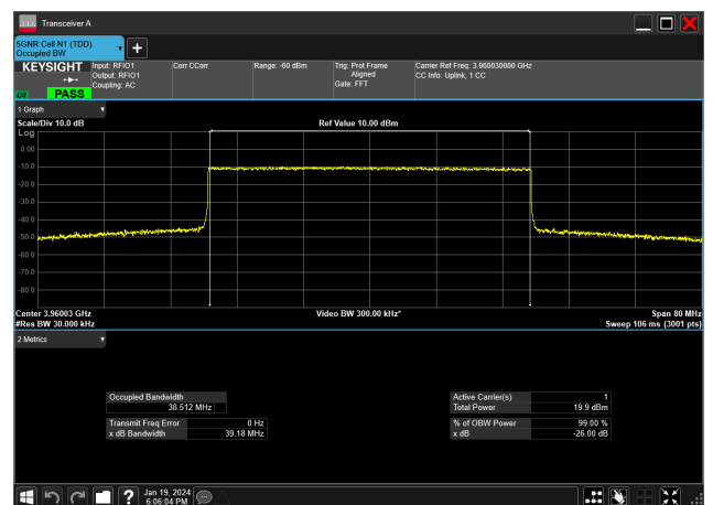
40MHz_15kHz_3960MHz_CP-OFDM 64 QAM_RB216@0&amp;38.512 MHz
