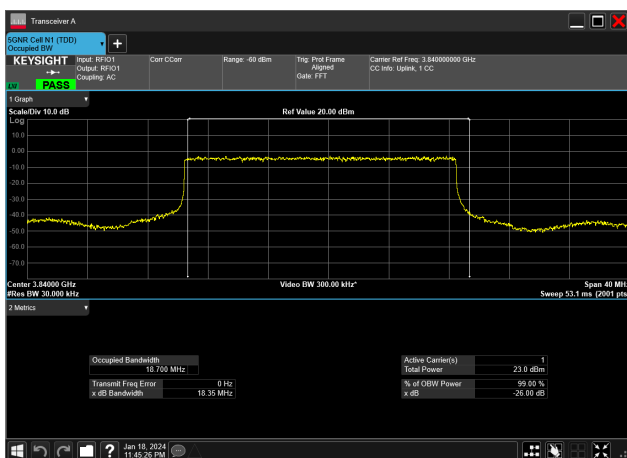
20MHz_15kHz_3840MHz_DFT-s-OFDM PI/2 BPSK_RB100@0&amp;18.700 MHz
