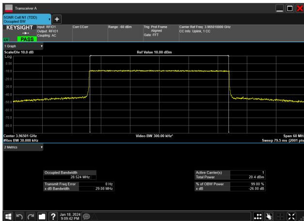
30MHz_15kHz_3965MHz_CP-OFDM 16 QAM_RB160@0&amp;28.524 MHz
