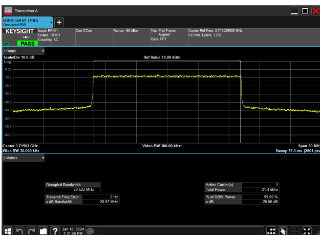
30MHz_15kHz_3715MHz_DFT-s-OFDM 16 QAM_RB160@0&amp;28.522 MHz
