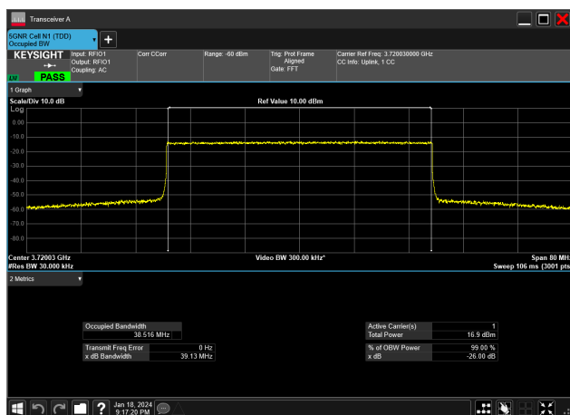
40MHz_15kHz_3720MHz_CP-OFDM 256 QAM_RB216@0&amp;38.516 MHz
