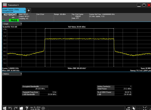
30MHz_15kHz_3840MHz_DFT-s-OFDM PI/2 BPSK_RB160@0&amp;28.525 MHz
