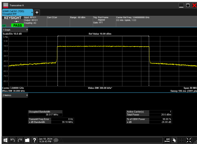
40MHz_15kHz_3840MHz_CP-OFDM 16 QAM_RB216@0&amp;38.517 MHz
