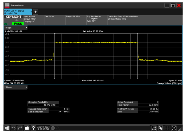
40MHz_15kHz_3720MHz_DFT-s-OFDM 64 QAM_RB216@0&amp;38.479 MHz
