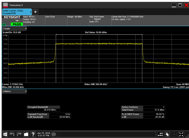
30MHz_15kHz_3715MHz_DFT-s-OFDM 64 QAM_RB160@0&amp;28.519 MHz
