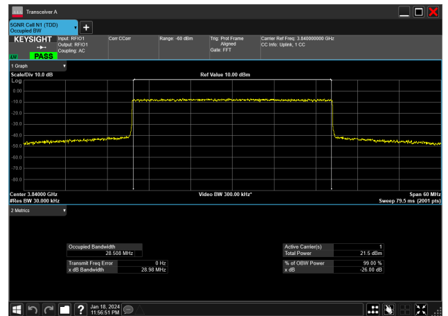
30MHz_15kHz_3840MHz_DFT-s-OFDM 16 QAM_RB160@0&amp;28.508 MHz
