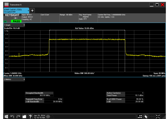
40MHz_15kHz_3840MHz_DFT-s-OFDM 256 QAM_RB216@0&amp;38.510 MHz
