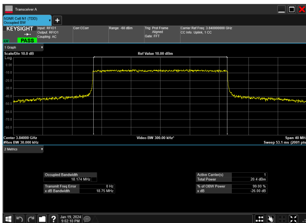
20MHz_30kHz_3840MHz_CP-OFDM 64 QAM_RB51@0&amp;18.174 MHz
