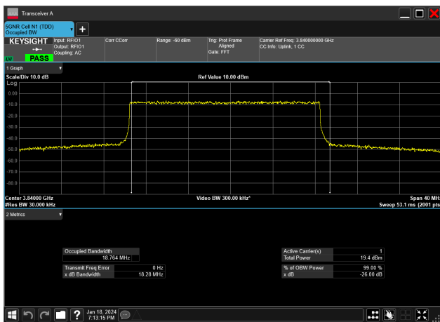
20MHz_15kHz_3840MHz_DFT-s-OFDM 256 QAM_RB100@0&amp;18.764 MHz
