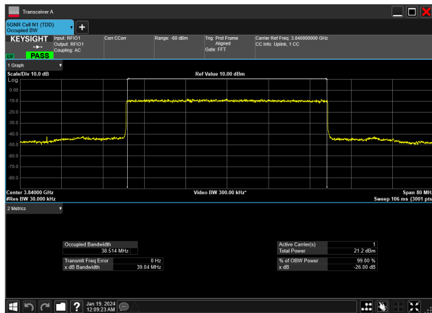
40MHz_15kHz_3840MHz_DFT-s-OFDM 64 QAM_RB216@0&amp;38.514 MHz
