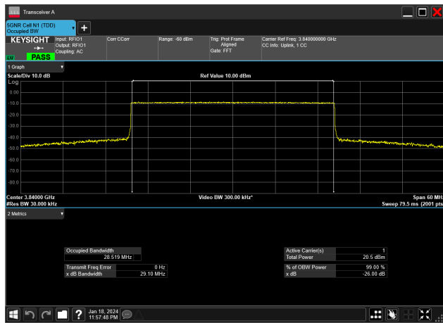
30MHz_15kHz_3840MHz_CP-OFDM QPSK_RB160@0&amp;28.519 MHz
