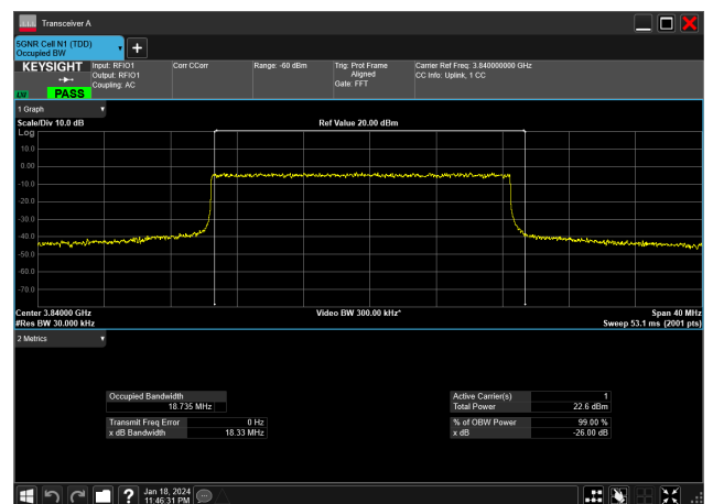
20MHz_15kHz_3840MHz_DFT-s-OFDM QPSK_RB100@0&amp;18.735 MHz
