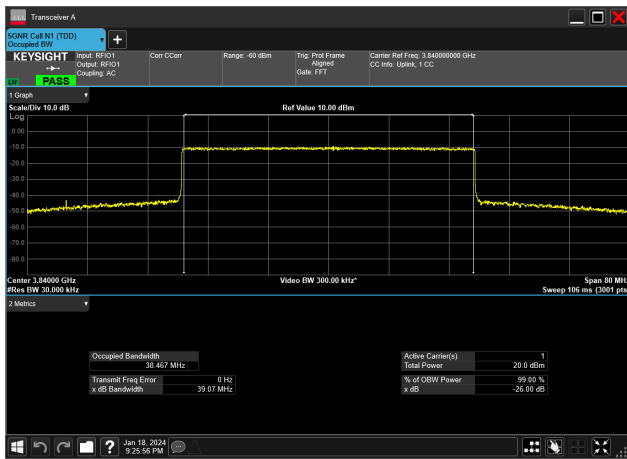
40MHz_15kHz_3840MHz_CP-OFDM 64 QAM_RB216@0&amp;38.467 MHz
