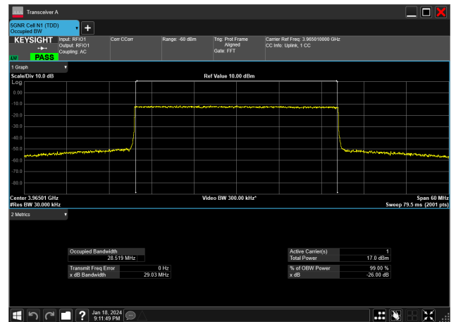
30MHz_15kHz_3965MHz_CP-OFDM 256 QAM_RB160@0&amp;28.519 MHz
