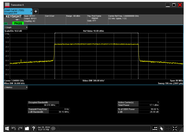
40MHz_15kHz_3840MHz_CP-OFDM 256 QAM_RB216@0&amp;38.515 MHz
