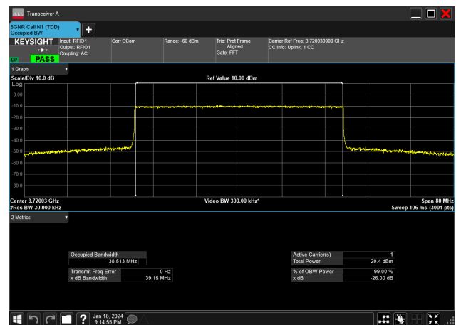
40MHz_15kHz_3720MHz_CP-OFDM 16 QAM_RB216@0&amp;38.513 MHz
