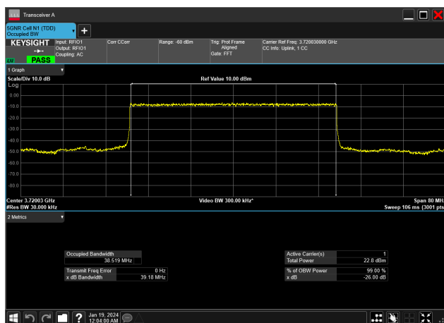
40MHz_15kHz_3720MHz_DFT-s-OFDM PI/2 BPSK_RB216@0&amp;38.519 MHz
