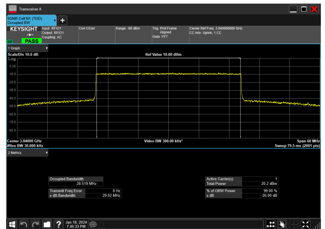
30MHz_15kHz_3840MHz_CP-OFDM 64 QAM_RB160@0&amp;28.519 MHz
