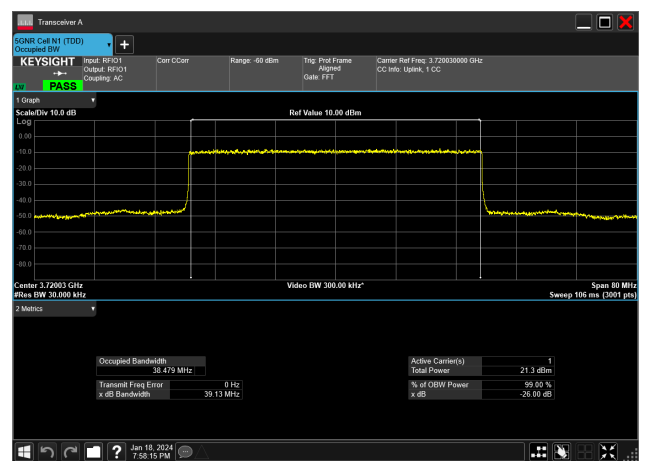
40MHz_15kHz_3720MHz_DFT-s-OFDM 16 QAM_RB216@0&amp;38.479 MHz
