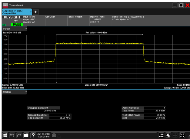
30MHz_15kHz_3715MHz_DFT-s-OFDM QPSK_RB160@0&amp;28.500 MHz
