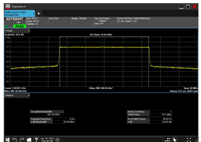
30MHz_15kHz_3965MHz_DFT-s-OFDM 256 QAM_RB160@0&amp;28.518 MHz
