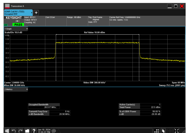
30MHz_15kHz_3840MHz_DFT-s-OFDM QPSK_RB160@0&amp;28.517 MHz
