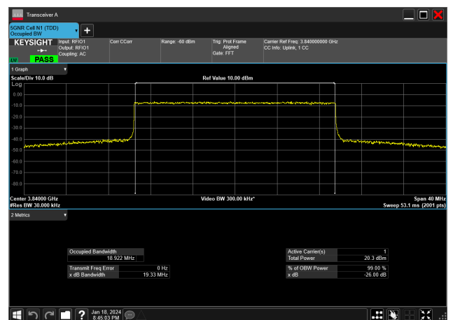
20MHz_15kHz_3840MHz_CP-OFDM 64 QAM_RB106@0&amp;18.922 MHz
