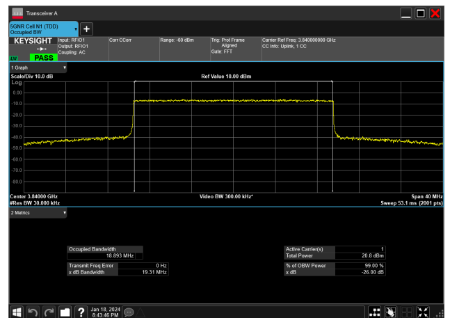
20MHz_15kHz_3840MHz_CP-OFDM 16 QAM_RB106@0&amp;18.893 MHz
