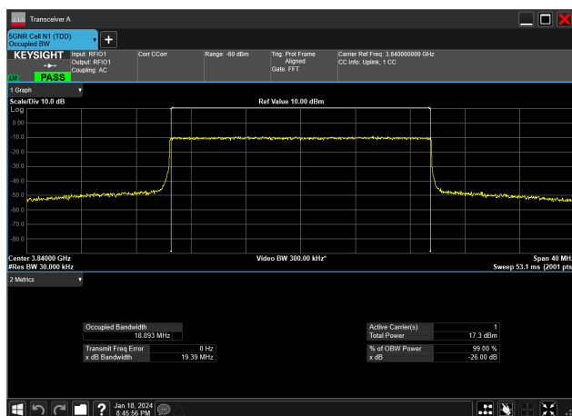
20MHz_15kHz_3840MHz_CP-OFDM 256 QAM_RB106@0&amp;18.893 MHz
