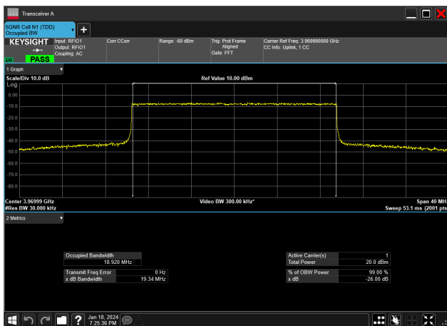
20MHz_15kHz_3970MHz_CP-OFDM 64 QAM_RB106@0&amp;18.920 MHz
