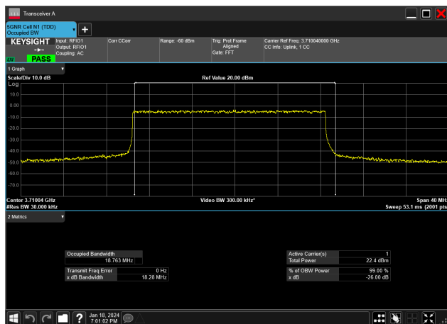
20MHz_15kHz_3710MHz_DFT-s-OFDM QPSK_RB100@0&amp;18.763 MHz
