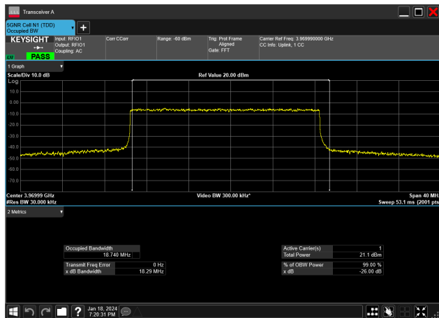
20MHz_15kHz_3970MHz_DFT-s-OFDM 64 QAM_RB100@0&amp;18.740 MHz
