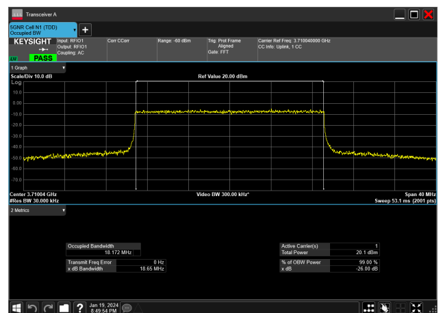
20MHz_30kHz_3710MHz_CP-OFDM 64 QAM_RB51@0&amp;18.172 MHz
