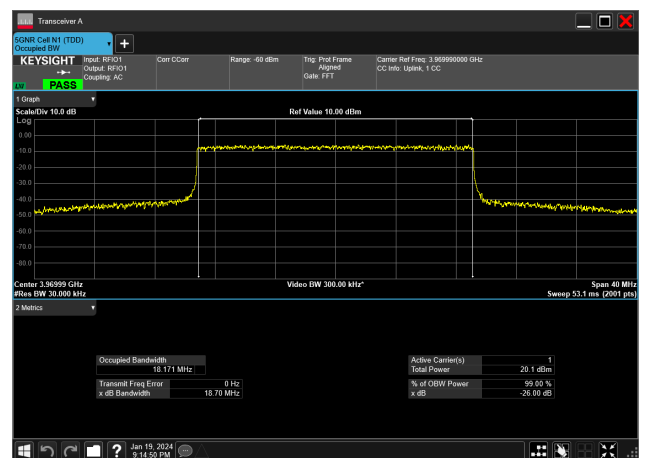
20MHz_30kHz_3970MHz_CP-OFDM 64 QAM_RB51@0&amp;18.171 MHz
