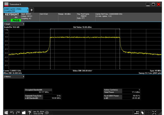
20MHz_30kHz_3840MHz_CP-OFDM 256 QAM_RB51@0&amp;18.177 MHz
