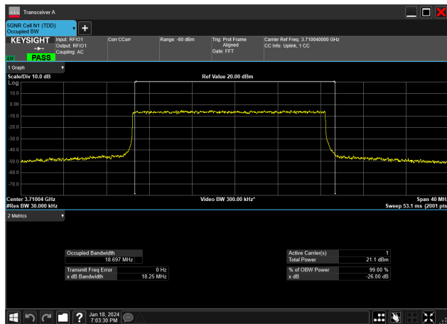
20MHz_15kHz_3710MHz_DFT-s-OFDM 64 QAM_RB100@0&amp;18.697 MHz
