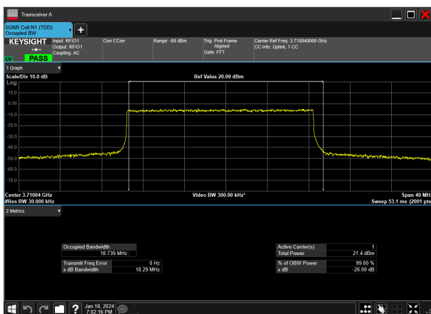
20MHz_15kHz_3710MHz_DFT-s-OFDM 16 QAM_RB100@0&amp;18.739 MHz
