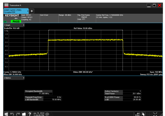
80MHz_30kHz_3740MHz_CP-OFDM 64 QAM_RB217@0&amp;77.288 MHz
