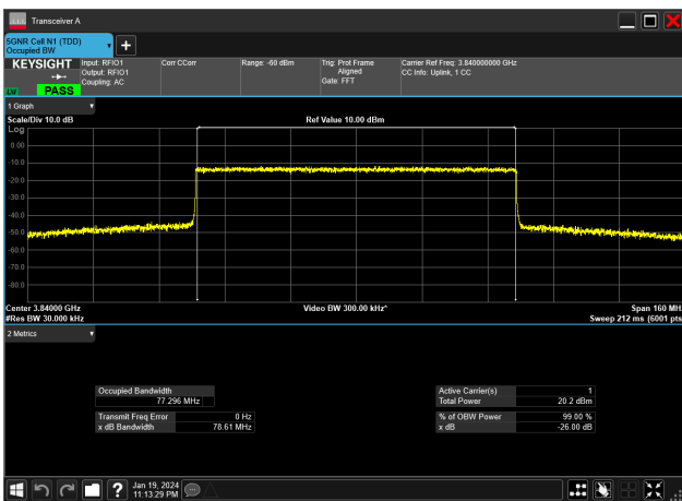
80MHz_30kHz_3840MHz_CP-OFDM 64 QAM_RB217@0&amp;77.296 MHz
