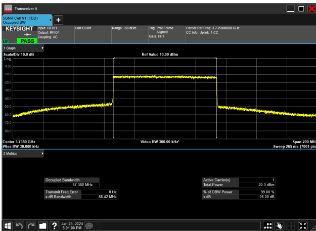
70MHz_30kHz_3735MHz_CP-OFDM 64 QAM_RB189@0&amp;67.380 MHz
