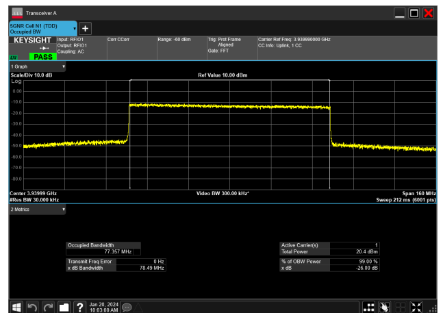
80MHz_30kHz_3940MHz_CP-OFDM 16 QAM_RB217@0&amp;77.357 MHz
