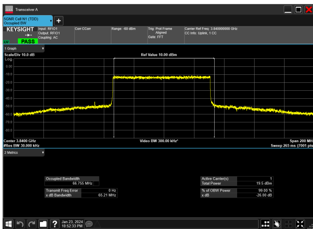
70MHz_30kHz_3840MHz_DFT-s-OFDM 256 QAM_RB180@0&amp;66.755 MHz
