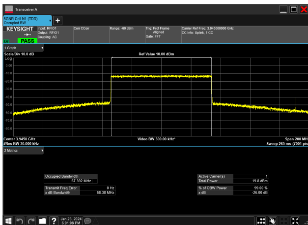
70MHz_30kHz_3945MHz_CP-OFDM 64 QAM_RB189@0&amp;67.392 MHz
