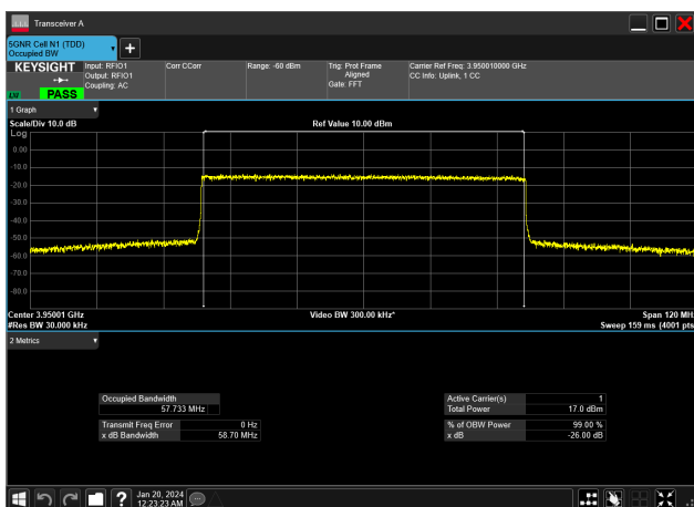
60MHz_30kHz_3950MHz_CP-OFDM 256 QAM_RB162@0&amp;57.733 MHz
