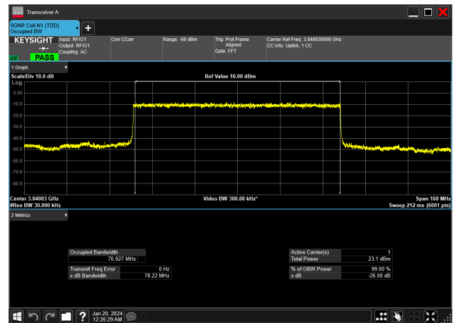
80MHz_30kHz_3840MHz_DFT-s-OFDM PI/2 BPSK_RB216@0&amp;76.927 MHz
