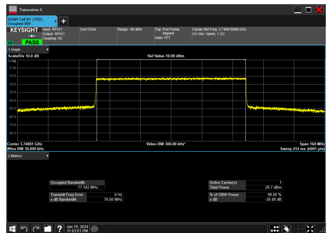
80MHz_30kHz_3740MHz_CP-OFDM 16 QAM_RB217@0&amp;77.342 MHz
