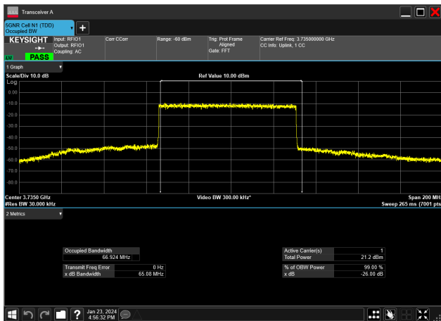
70MHz_30kHz_3735MHz_DFT-s-OFDM 64 QAM_RB180@0&amp;66.924 MHz
