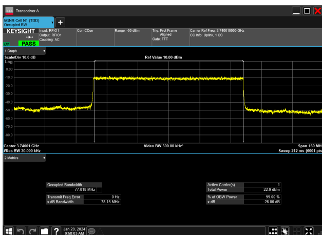
80MHz_30kHz_3740MHz_DFT-s-OFDM PI/2 BPSK_RB216@0&amp;77.018 MHz
