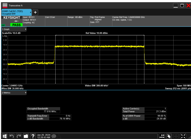
80MHz_30kHz_3840MHz_DFT-s-OFDM 16 QAM_RB216@0&amp;77.016 MHz
