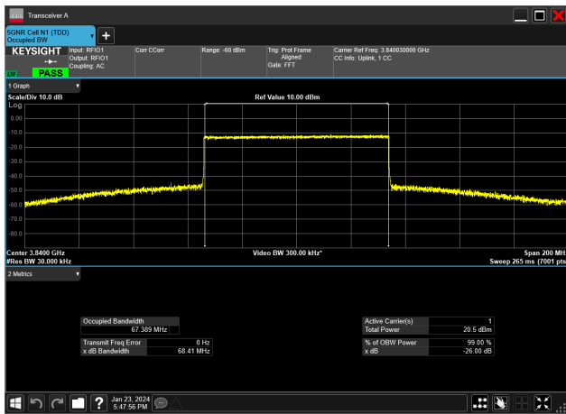
70MHz_30kHz_3840MHz_CP-OFDM QPSK_RB189@0&amp;67.389 MHz
