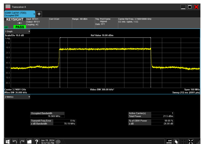
80MHz_30kHz_3740MHz_DFT-s-OFDM 16 QAM_RB216@0&amp;76.969 MHz
