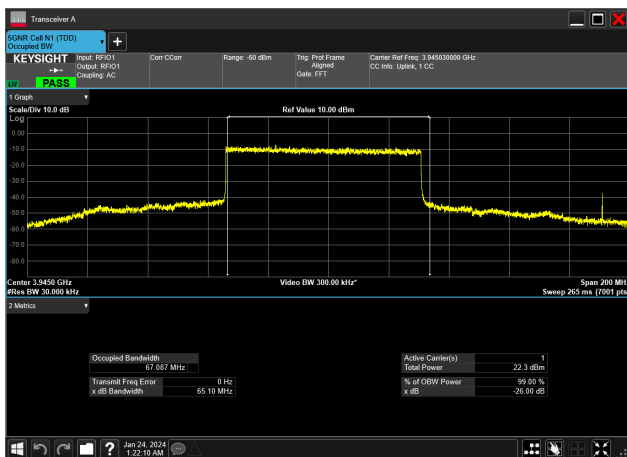
70MHz_30kHz_3945MHz_DFT-s-OFDM QPSK_RB180@0&amp;67.087 MHz
