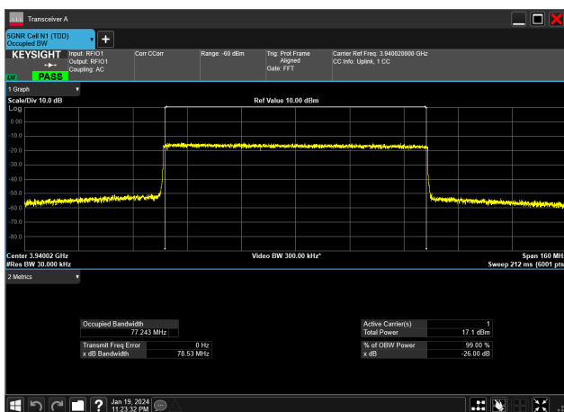
80MHz_30kHz_3940MHz_CP-OFDM 256 QAM_RB217@0&amp;77.243 MHz
