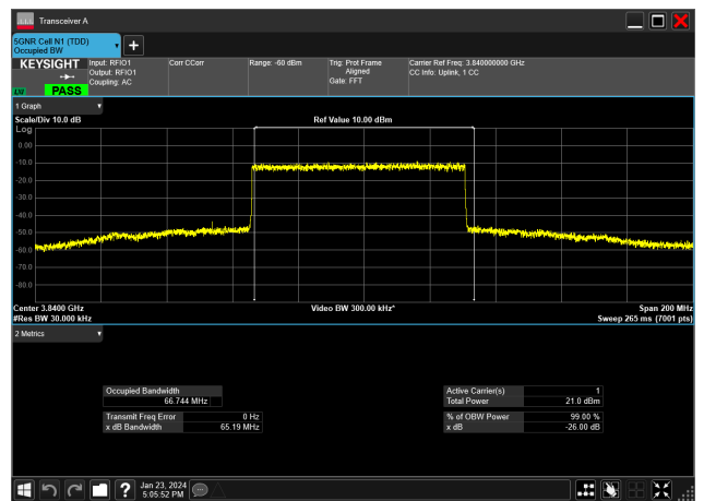
70MHz_30kHz_3840MHz_DFT-s-OFDM 64 QAM_RB180@0&amp;66.744 MHz
