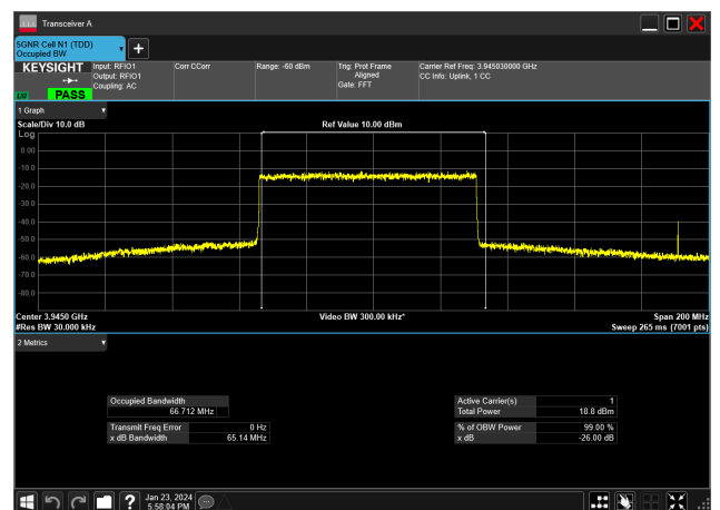
70MHz_30kHz_3945MHz_DFT-s-OFDM 256 QAM_RB180@0&amp;66.712 MHz
