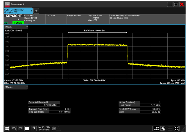
70MHz_30kHz_3735MHz_CP-OFDM 256 QAM_RB189@0&amp;67.330 MHz
