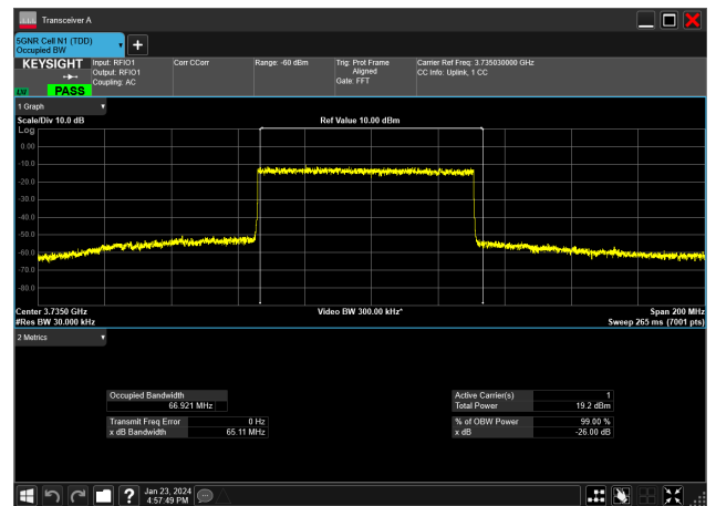
70MHz_30kHz_3735MHz_DFT-s-OFDM 256 QAM_RB180@0&amp;66.921 MHz
