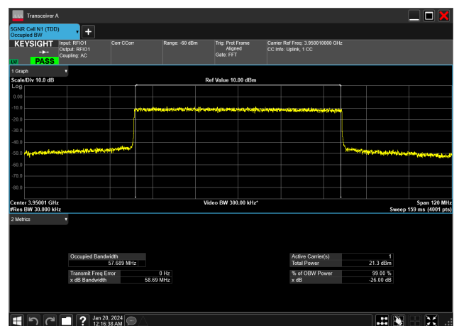
60MHz_30kHz_3950MHz_DFT-s-OFDM 16 QAM_RB162@0&amp;57.689 MHz
