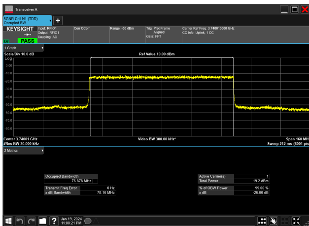
80MHz_30kHz_3740MHz_DFT-s-OFDM 256 QAM_RB216@0&amp;76.878 MHz
