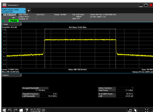
80MHz_30kHz_3740MHz_CP-OFDM 256 QAM_RB217@0&amp;77.199 MHz
