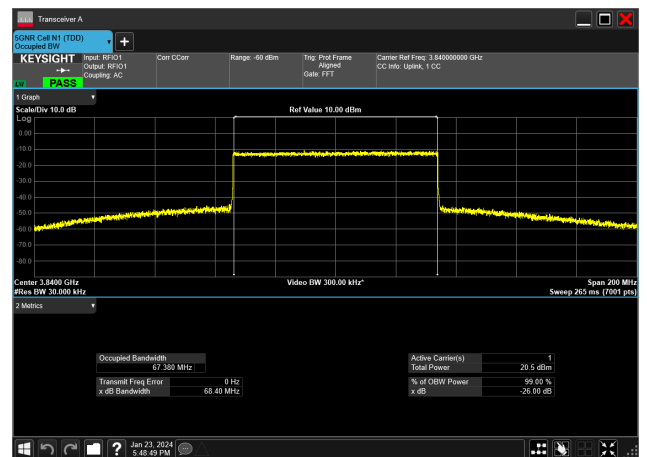
70MHz_30kHz_3840MHz_CP-OFDM 16 QAM_RB189@0&amp;67.380 MHz
