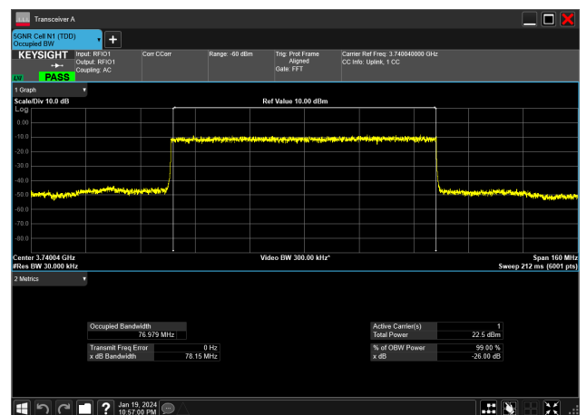
80MHz_30kHz_3740MHz_DFT-s-OFDM QPSK_RB216@0&amp;76.979 MHz
