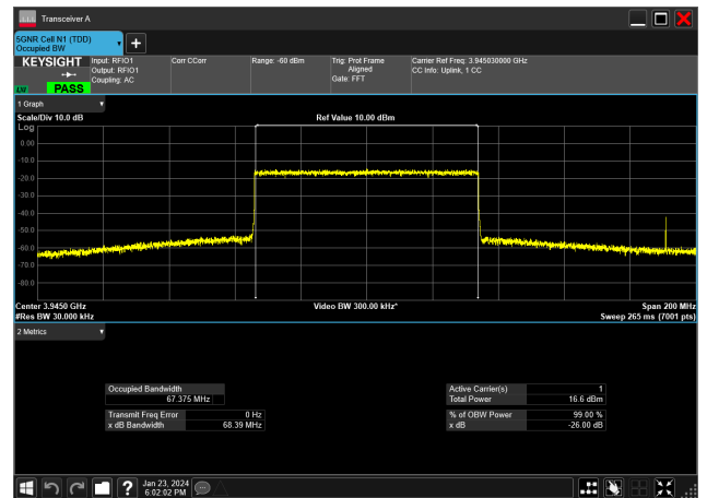
70MHz_30kHz_3945MHz_CP-OFDM 256 QAM_RB189@0&amp;67.375 MHz
