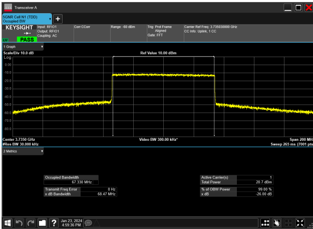
70MHz_30kHz_3735MHz_CP-OFDM 16 QAM_RB189@0&amp;67.330 MHz
