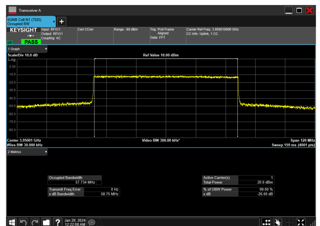
60MHz_30kHz_3950MHz_CP-OFDM 64 QAM_RB162@0&amp;57.734 MHz
