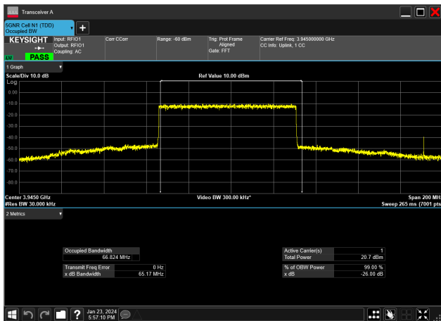
70MHz_30kHz_3945MHz_DFT-s-OFDM 64 QAM_RB180@0&amp;66.824 MHz
