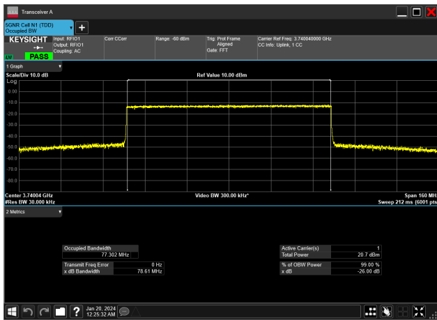
80MHz_30kHz_3740MHz_CP-OFDM QPSK_RB217@0&amp;77.302 MHz
