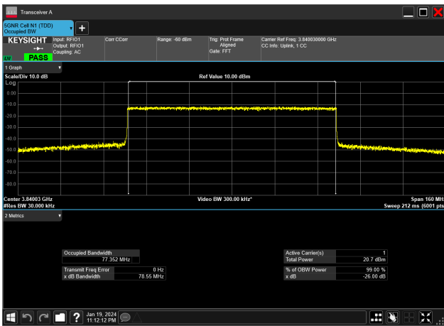
80MHz_30kHz_3840MHz_CP-OFDM 16 QAM_RB217@0&amp;77.352 MHz
