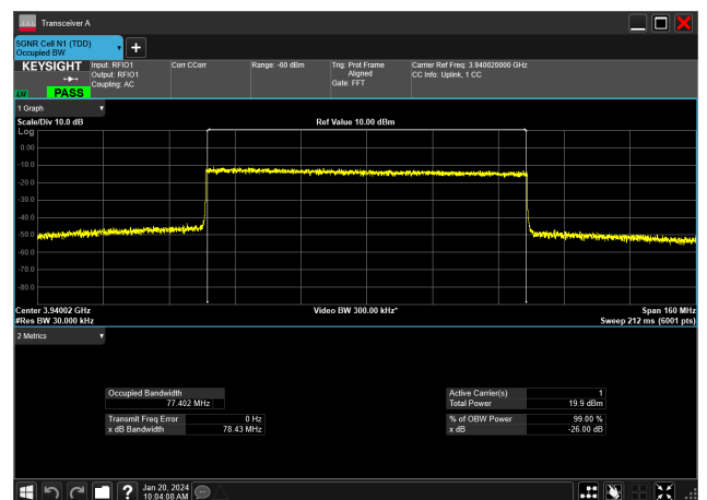
80MHz_30kHz_3940MHz_CP-OFDM 64 QAM_RB217@0&amp;77.402 MHz
