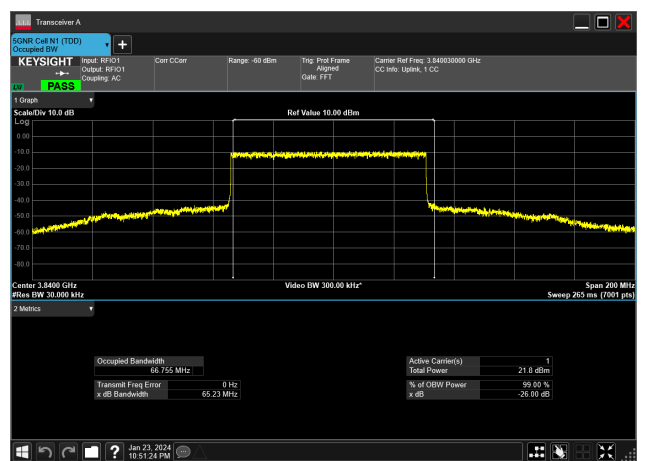
70MHz_30kHz_3840MHz_DFT-s-OFDM 16 QAM_RB180@0&amp;66.755 MHz
