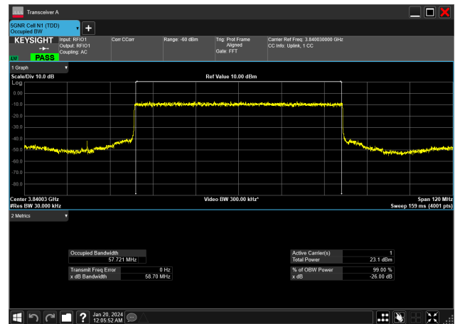
60MHz_30kHz_3840MHz_DFT-s-OFDM PI/2 BPSK_RB162@0&amp;57.721 MHz
