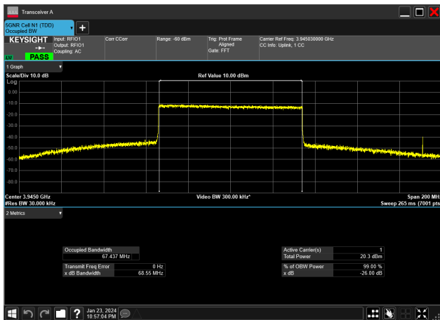
70MHz_30kHz_3945MHz_CP-OFDM 16 QAM_RB189@0&amp;67.437 MHz
