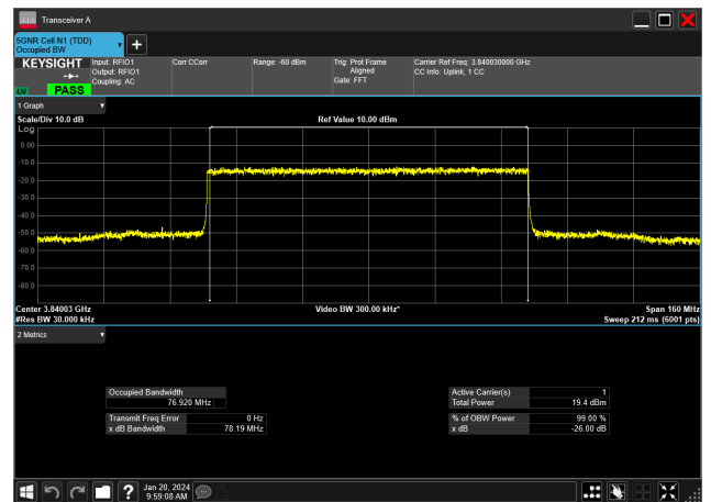
80MHz_30kHz_3840MHz_DFT-s-OFDM 256 QAM_RB216@0&amp;76.920 MHz
