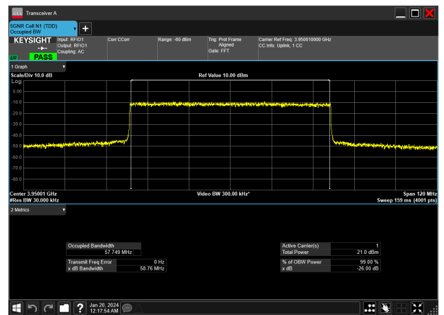
60MHz_30kHz_3950MHz_DFT-s-OFDM 64 QAM_RB162@0&amp;57.749 MHz
