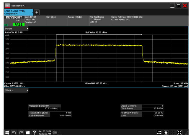
60MHz_30kHz_3950MHz_CP-OFDM 16 QAM_RB162@0&amp;57.724 MHz
