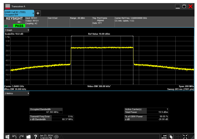
70MHz_30kHz_3840MHz_CP-OFDM 64 QAM_RB189@0&amp;67.393 MHz
