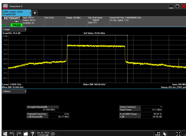
70MHz_30kHz_3945MHz_DFT-s-OFDM 16 QAM_RB180@0&amp;67.094 MHz
