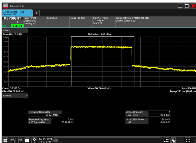
70MHz_30kHz_3735MHz_DFT-s-OFDM QPSK_RB180@0&amp;66.874 MHz
