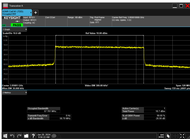
60MHz_30kHz_3950MHz_DFT-s-OFDM 256 QAM_RB162@0&amp;57.781 MHz
