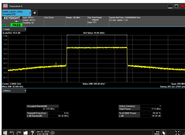
70MHz_30kHz_3840MHz_CP-OFDM 256 QAM_RB189@0&amp;67.379 MHz
