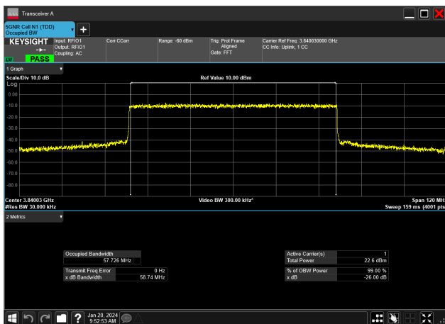
60MHz_30kHz_3840MHz_DFT-s-OFDM QPSK_RB162@0&amp;57.726 MHz
