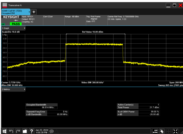
70MHz_30kHz_3735MHz_DFT-s-OFDM 16 QAM_RB180@0&amp;66.814 MHz
