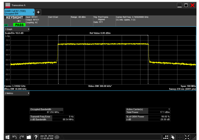
90MHz_30kHz_3745MHz_CP-OFDM 256 QAM_RB245@0&amp;87.255 MHz
