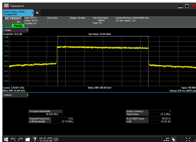
90MHz_30kHz_3935MHz_DFT-s-OFDM QPSK_RB243@0&amp;86.820 MHz
