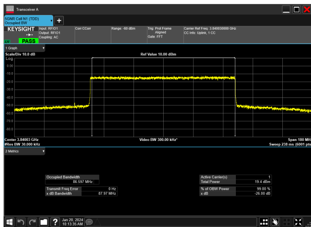
90MHz_30kHz_3840MHz_DFT-s-OFDM 256 QAM_RB243@0&amp;86.597 MHz
