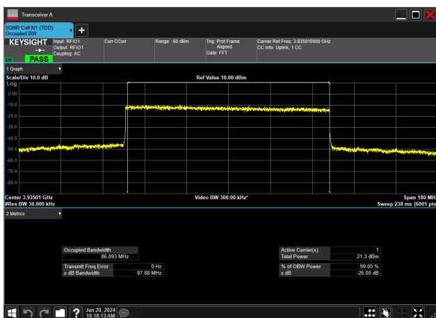
90MHz_30kHz_3935MHz_DFT-s-OFDM 16 QAM_RB243@0&amp;86.893 MHz
