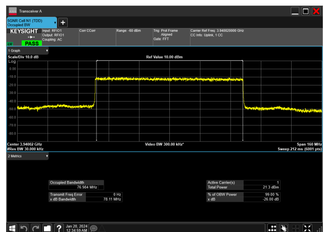
80MHz_30kHz_3940MHz_DFT-s-OFDM 16 QAM_RB216@0&amp;76.984 MHz
