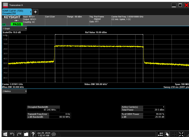
90MHz_30kHz_3935MHz_CP-OFDM 16 QAM_RB245@0&amp;87.245 MHz
