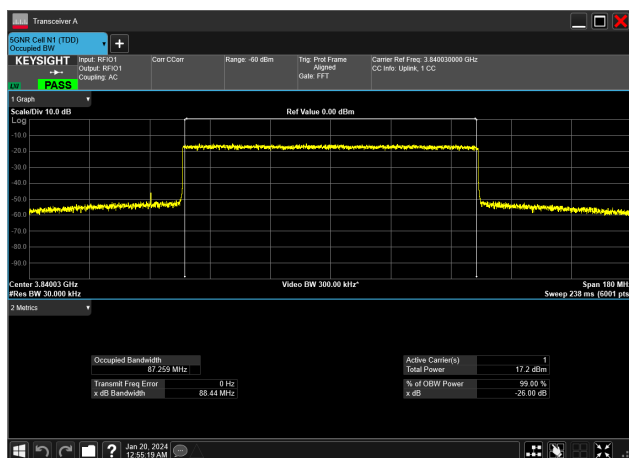
90MHz_30kHz_3840MHz_CP-OFDM 256 QAM_RB245@0&amp;87.259 MHz
