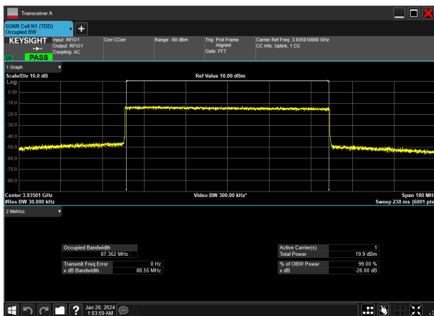
90MHz_30kHz_3935MHz_CP-OFDM 64 QAM_RB245@0&amp;87.362 MHz
