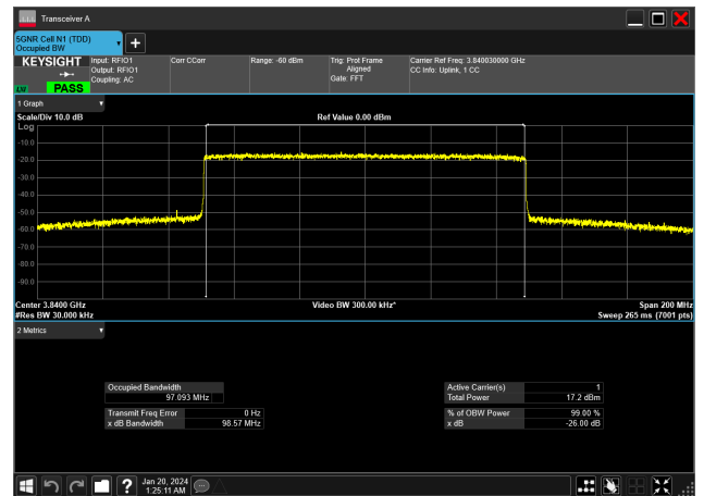
100MHz_30kHz_3840MHz_CP-OFDM 256 QAM_RB273@0&amp;97.093 MHz
