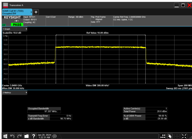
100MHz_30kHz_3840MHz_CP-OFDM 16 QAM_RB273@0&amp;97.207 MHz
