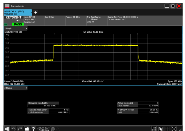
90MHz_30kHz_3840MHz_CP-OFDM 64 QAM_RB245@0&amp;87.360 MHz
