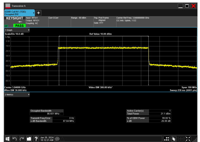
90MHz_30kHz_3840MHz_DFT-s-OFDM 64 QAM_RB243@0&amp;86.601 MHz
