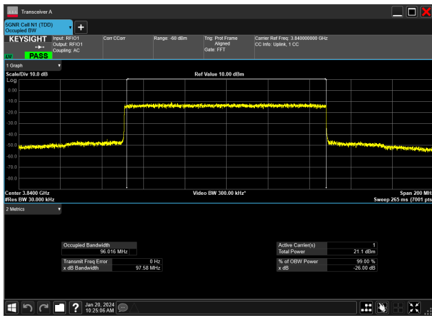
100MHz_30kHz_3840MHz_DFT-s-OFDM 64 QAM_RB270@0&96.016 MHz
