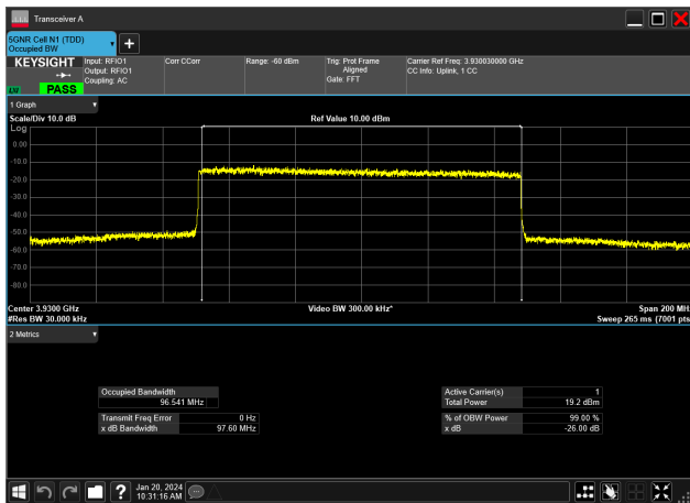
100MHz_30kHz_3930MHz_DFT-s-OFDM 256 QAM_RB270@0&96.541 MHz
