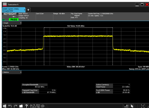
90MHz_30kHz_3745MHz_DFT-s-OFDM QPSK_RB243@0&amp;86.522 MHz
