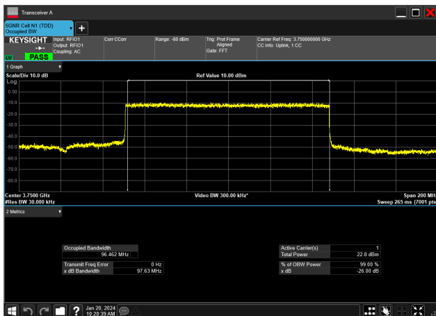
100MHz_30kHz_3750MHz_DFT-s-OFDM PI/2 BPSK_RB270@0&96.462 MHz
