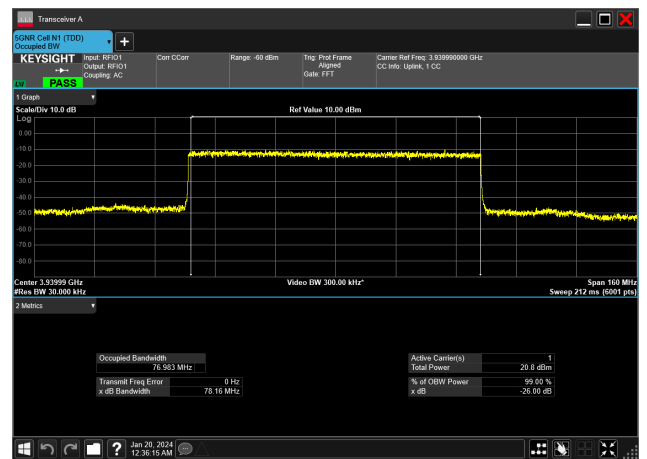
80MHz_30kHz_3940MHz_DFT-s-OFDM 64 QAM_RB216@0&amp;76.983 MHz
