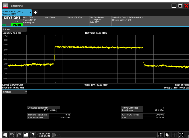
80MHz_30kHz_3940MHz_DFT-s-OFDM 256 QAM_RB216@0&amp;77.033 MHz
