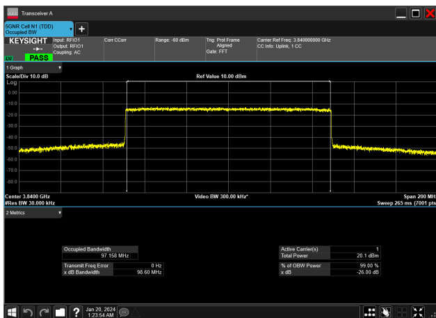
100MHz_30kHz_3840MHz_CP-OFDM 64 QAM_RB273@0&amp;97.158 MHz
