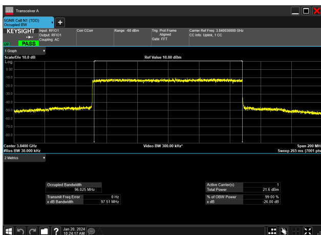
100MHz_30kHz_3840MHz_DFT-s-OFDM 16 QAM_RB270@0&amp;96.025 MHz
