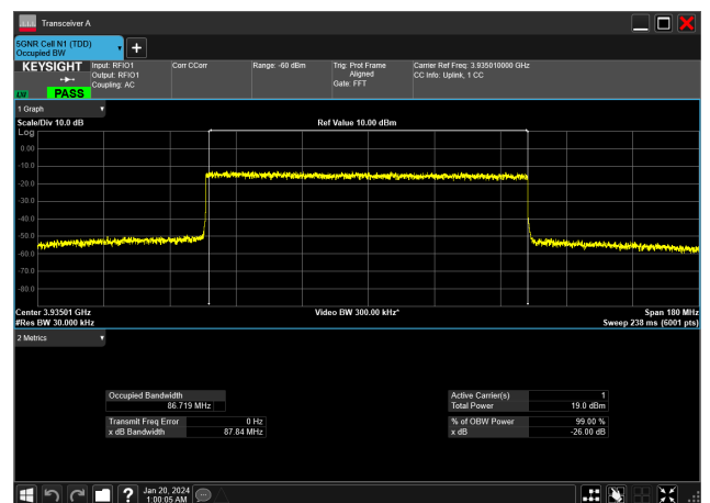
90MHz_30kHz_3935MHz_DFT-s-OFDM 256 QAM_RB243@0&amp;86.719 MHz
