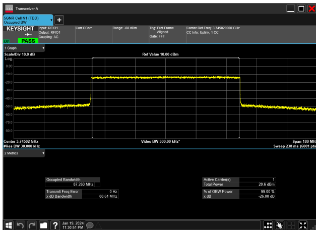
90MHz_30kHz_3745MHz_CP-OFDM 16 QAM_RB245@0&amp;87.263 MHz
