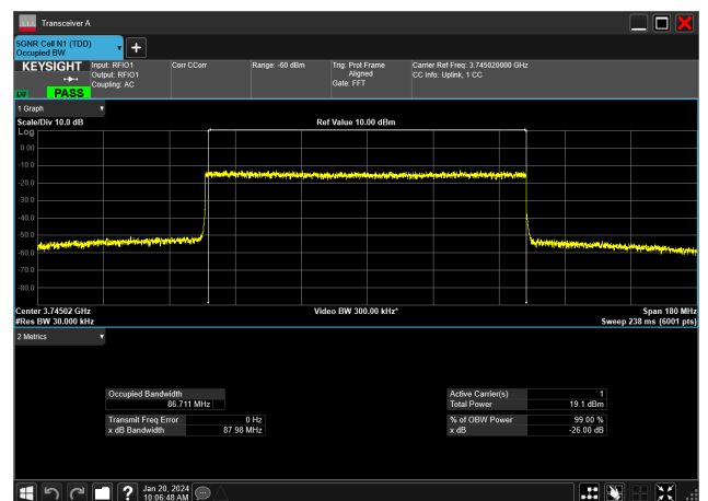
90MHz_30kHz_3745MHz_DFT-s-OFDM 256 QAM_RB243@0&amp;86.711 MHz
