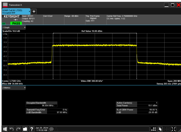
100MHz_30kHz_3750MHz_DFT-s-OFDM 256 QAM_RB270@0&96.004 MHz
