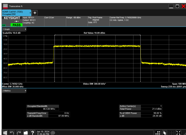
90MHz_30kHz_3745MHz_DFT-s-OFDM 16 QAM_RB243@0&amp;86.538 MHz
