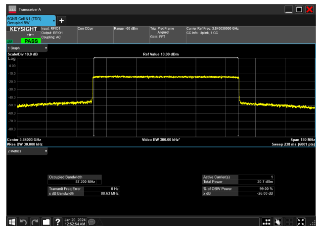
90MHz_30kHz_3840MHz_CP-OFDM 16 QAM_RB245@0&amp;87.200 MHz
