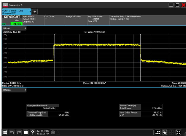
100MHz_30kHz_3840MHz_DFT-s-OFDM QPSK_RB270@0&96.068 MHz
