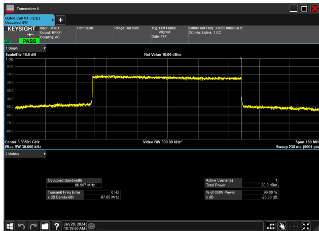
90MHz_30kHz_3935MHz_DFT-s-OFDM 64 QAM_RB243@0&amp;86.907 MHz
