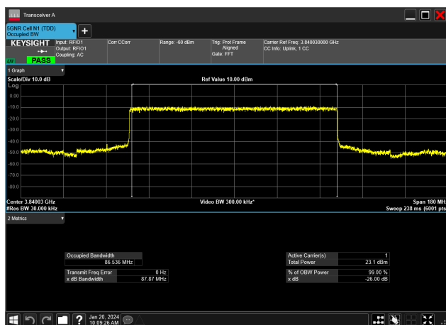
90MHz_30kHz_3840MHz_DFT-s-OFDM PI/2 BPSK_RB243@0&amp;86.536 MHz
