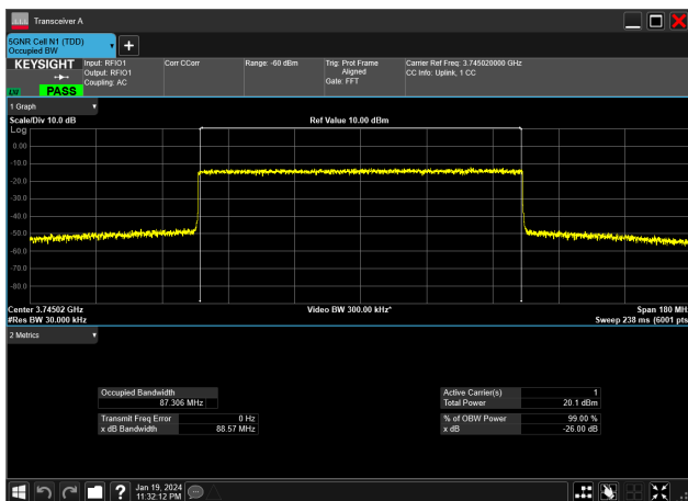
90MHz_30kHz_3745MHz_CP-OFDM 64 QAM_RB245@0&amp;87.306 MHz
