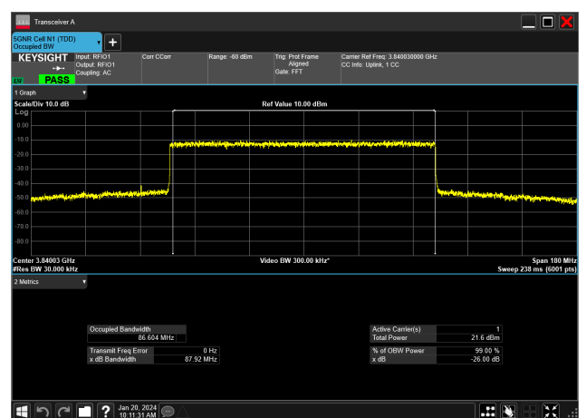
90MHz_30kHz_3840MHz_DFT-s-OFDM 16 QAM_RB243@0&amp;86.604 MHz
