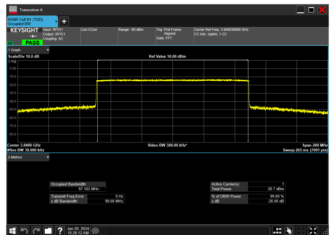
100MHz_30kHz_3840MHz_CP-OFDM QPSK_RB273@0&amp;97.162 MHz
