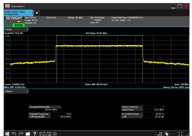
90MHz_30kHz_3840MHz_DFT-s-OFDM QPSK_RB243@0&amp;86.541 MHz
