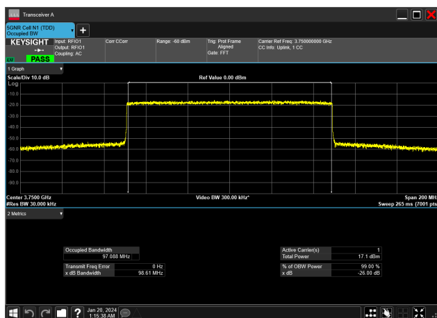
100MHz_30kHz_3750MHz_CP-OFDM 256 QAM_RB273@0&amp;97.088 MHz
