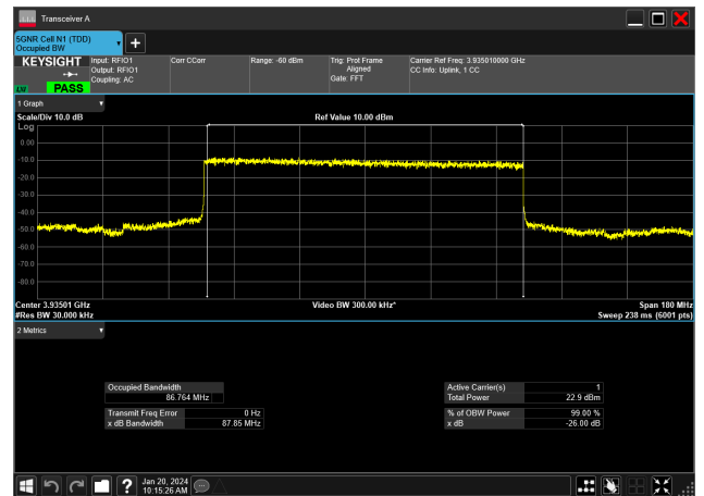
90MHz_30kHz_3935MHz_DFT-s-OFDM PI/2 BPSK_RB243@0&amp;86.764 MHz
