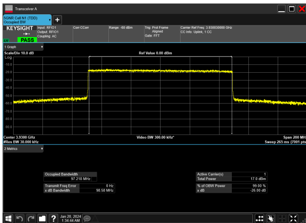
100MHz_30kHz_3930MHz_CP-OFDM 256 QAM_RB273@0&97.218 MHz
