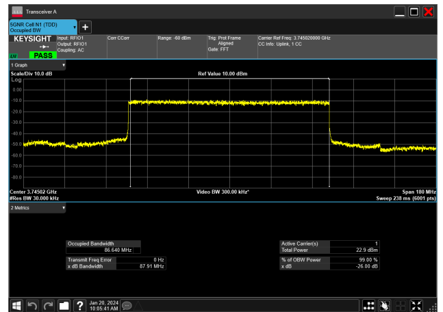
90MHz_30kHz_3745MHz_DFT-s-OFDM PI/2 BPSK_RB243@0&amp;86.640 MHz
