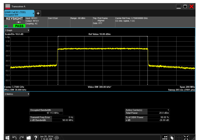
100MHz_30kHz_3750MHz_CP-OFDM 64 QAM_RB273@0&amp;97.113 MHz
