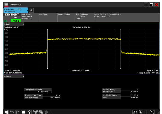
100MHz_30kHz_3750MHz_CP-OFDM 16 QAM_RB273@0&amp;97.156 MHz
