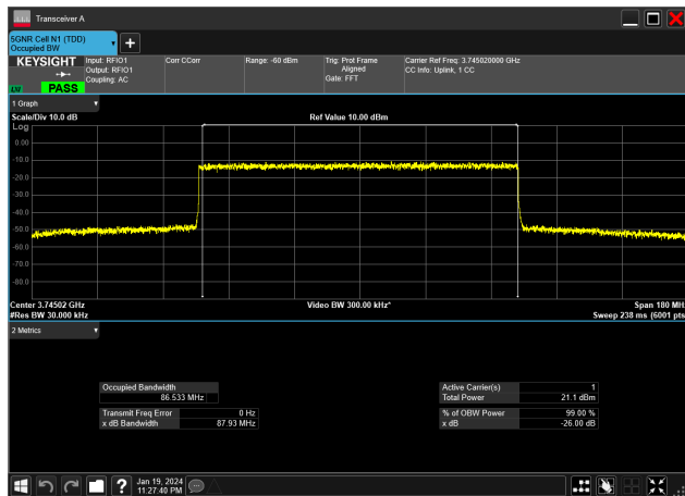
90MHz_30kHz_3745MHz_DFT-s-OFDM 64 QAM_RB243@0&amp;86.533 MHz
