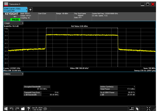
90MHz_30kHz_3935MHz_CP-OFDM 256 QAM_RB245@0&amp;87.303 MHz
