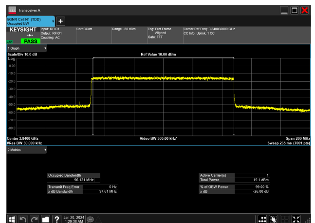
100MHz_30kHz_3840MHz_DFT-s-OFDM 256 QAM_RB270@0&amp;96.121 MHz
