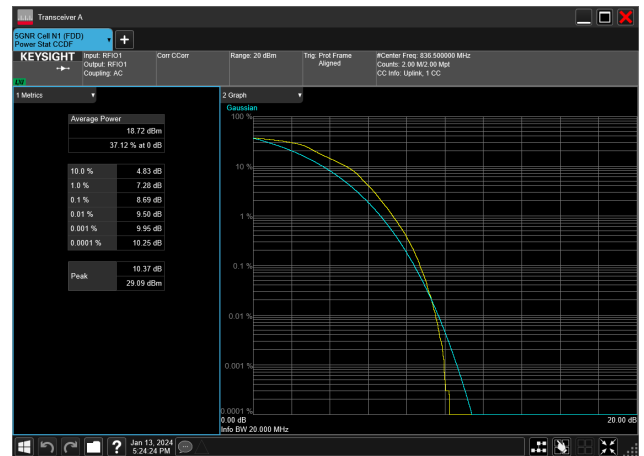
20MHz_15kHz_836.5MHz_DFT-s-OFDM 16 QAM_RB100@0&amp;8.69 dB
