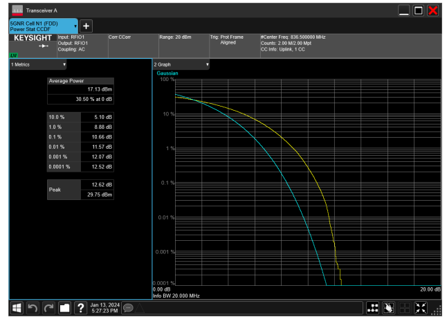
20MHz_15kHz_836.5MHz_CP-OFDM 64 QAM_RB106@0&amp;10.66 dB
