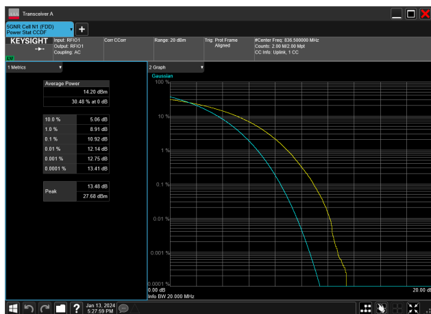
20MHz_15kHz_836.5MHz_CP-OFDM 256 QAM_RB106@0&amp;10.92 dB
