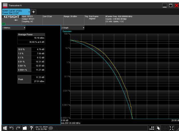
20MHz_15kHz_836.5MHz_DFT-s-OFDM 256 QAM_RB100@0&amp;9.12 dB
