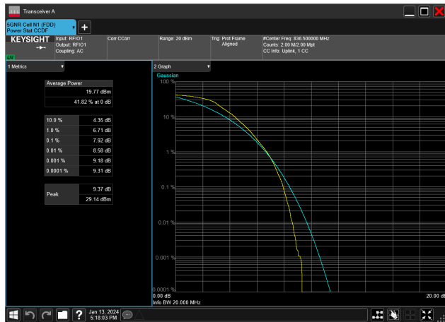
15MHz_15kHz_836.5MHz_DFT-s-OFDM QPSK_RB75@0&amp;7.92 dB
