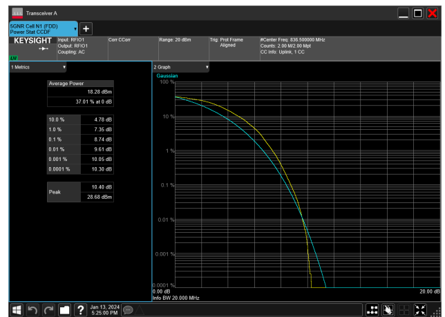
20MHz_15kHz_836.5MHz_DFT-s-OFDM 64 QAM_RB100@0&amp;8.74 dB
