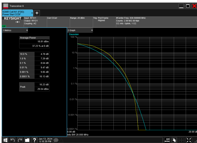
15MHz_15kHz_836.5MHz_DFT-s-OFDM 16 QAM_RB75@0&amp;8.64 dB
