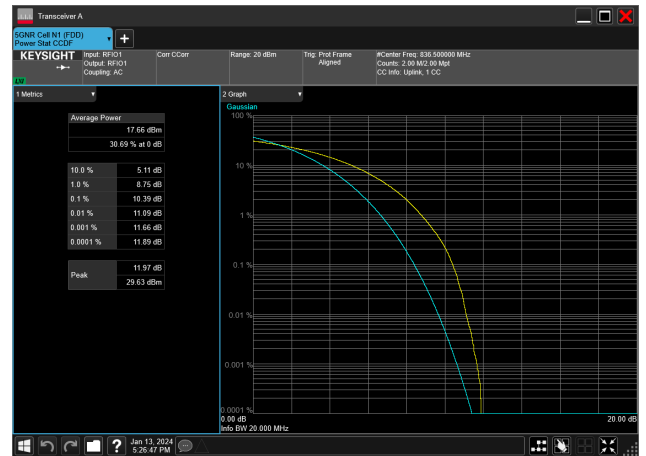
20MHz_15kHz_836.5MHz_CP-OFDM 16 QAM_RB106@0&amp;10.39 dB
