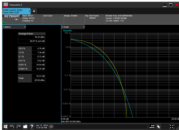
15MHz_15kHz_836.5MHz_DFT-s-OFDM 64 QAM_RB75@0&amp;8.72 dB
