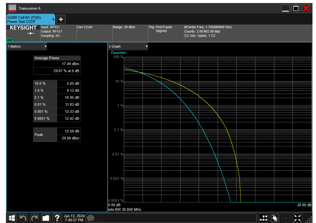
30MHz_15kHz_1745MHz_CP-OFDM 64 QAM_RB160@0&amp;10.95 dB
