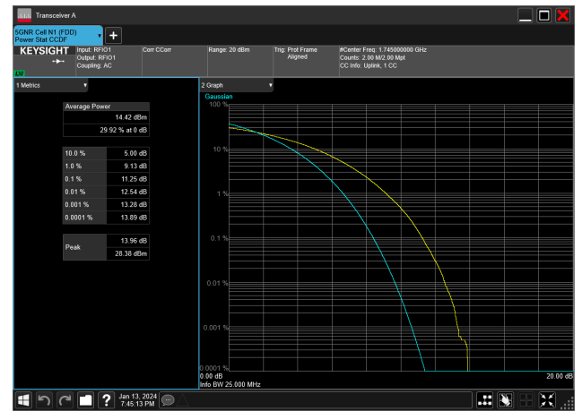
25MHz_15kHz_1745MHz_CP-OFDM 256 QAM_RB133@0&amp;11.25 dB
