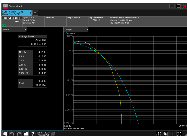
20MHz_15kHz_1745MHz_DFT-s-OFDM PI/2 BPSK_RB100@0&amp;7.26 dB
