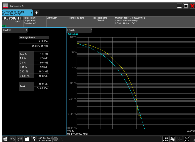
15MHz_15kHz_1745MHz_DFT-s-OFDM 16 QAM_RB75@0&amp;9.08 dB
