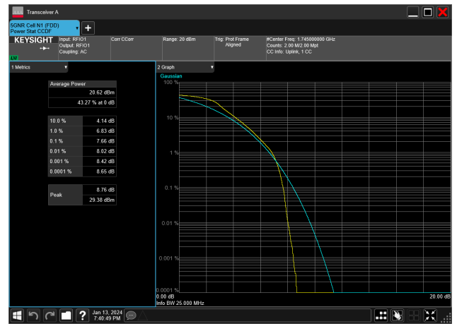
25MHz_15kHz_1745MHz_DFT-s-OFDM PI/2 BPSK_RB128@0&amp;7.66 dB
