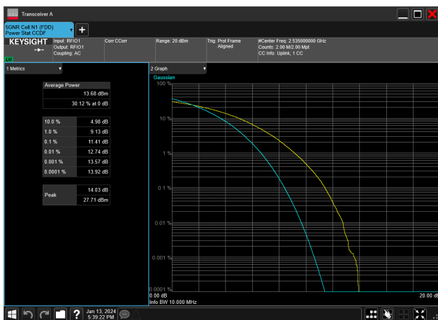
10MHz_15kHz_2535MHz_CP-OFDM 256 QAM_RB52@0&amp;11.41 dB
