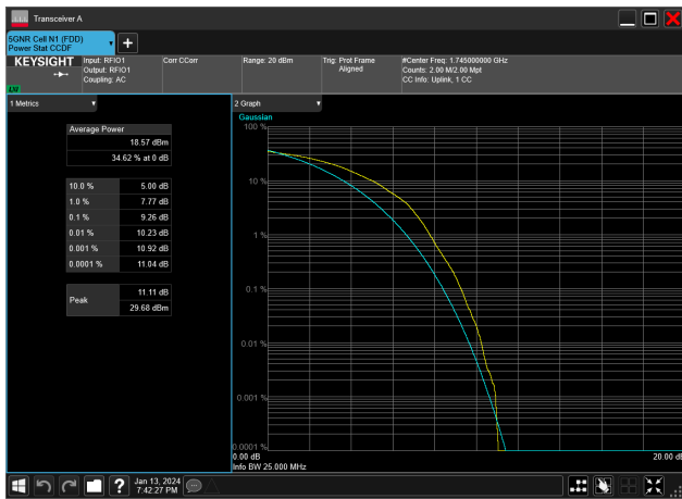
25MHz_15kHz_1745MHz_DFT-s-OFDM 64 QAM_RB128@0&amp;9.26 dB
