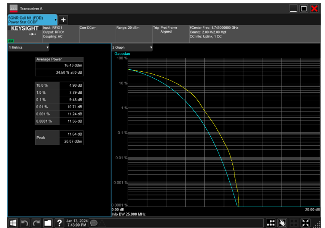
25MHz_15kHz_1745MHz_DFT-s-OFDM 256 QAM_RB128@0&amp;9.48 dB
