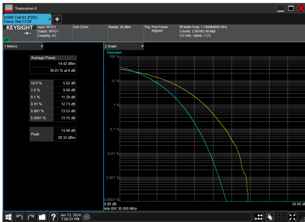
30MHz_15kHz_1745MHz_CP-OFDM 256 QAM_RB160@0&amp;11.29 dB
