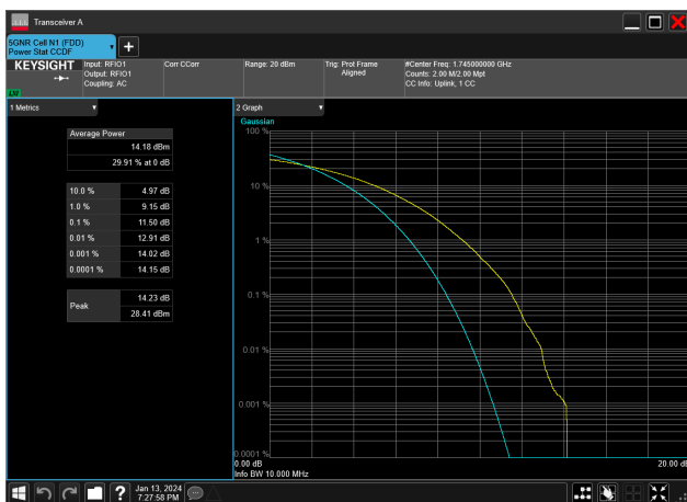
10MHz_15kHz_1745MHz_CP-OFDM 256 QAM_RB52@0&amp;11.50 dB
