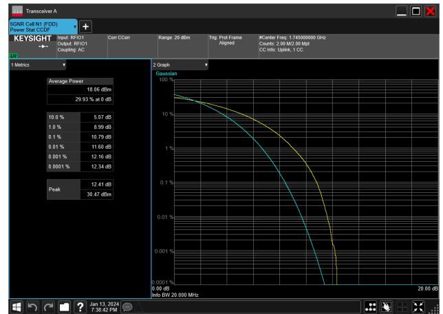
20MHz_15kHz_1745MHz_CP-OFDM 16 QAM_RB106@0&amp;10.79 dB
