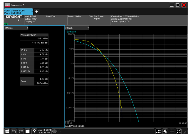
15MHz_15kHz_2535MHz_DFT-s-OFDM PI/2 BPSK_RB75@0&amp;7.11 dB
