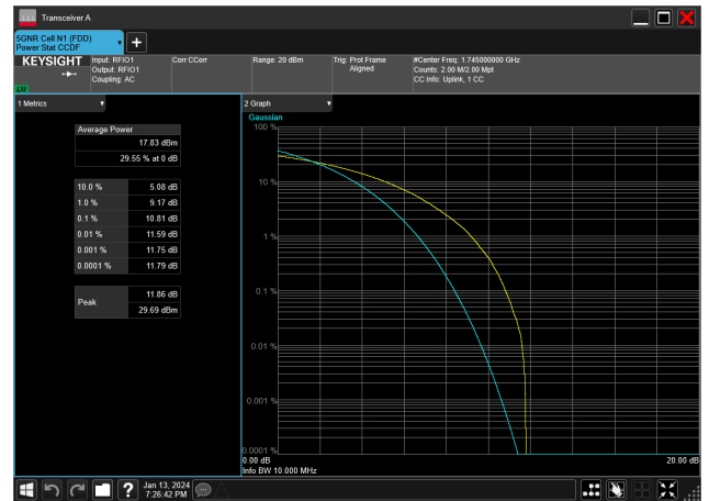
10MHz_15kHz_1745MHz_CP-OFDM 16 QAM_RB52@0&amp;10.81 dB
