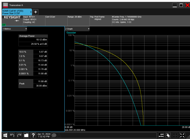
15MHz_15kHz_1745MHz_CP-OFDM 16 QAM_RB79@0&amp;10.73 dB
