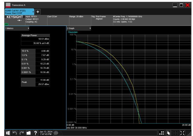
30MHz_15kHz_1745MHz_DFT-s-OFDM 64 QAM_RB160@0&amp;9.29 dB
