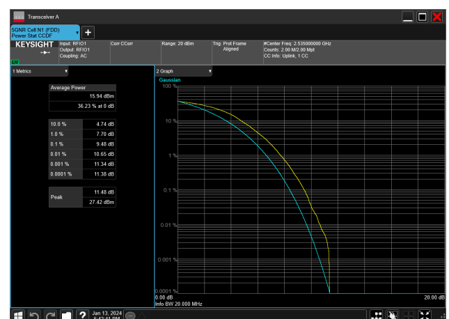
15MHz_15kHz_2535MHz_DFT-s-OFDM 256 QAM_RB75@0&amp;9.48 dB
