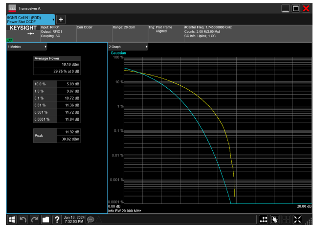
15MHz_15kHz_1745MHz_CP-OFDM QPSK_RB79@0&amp;10.72 dB
