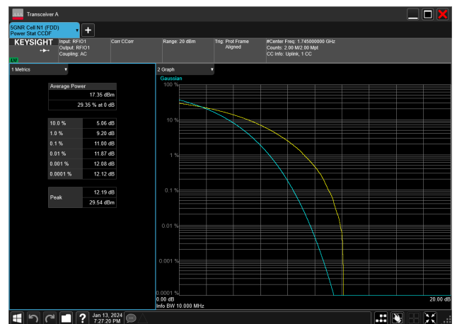
10MHz_15kHz_1745MHz_CP-OFDM 64 QAM_RB52@0&amp;11.00 dB
