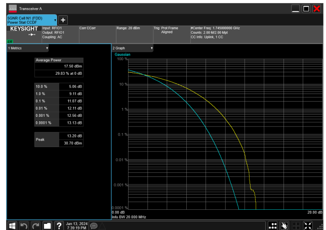
20MHz_15kHz_1745MHz_CP-OFDM 64 QAM_RB106@0&amp;11.07 dB
