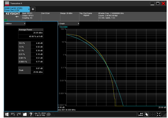
30MHz_15kHz_1745MHz_DFT-s-OFDM QPSK_RB160@0&amp;8.30 dB
