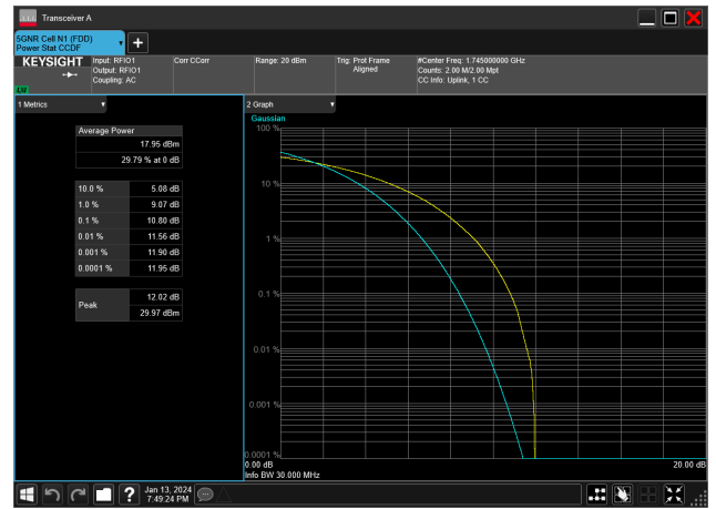
30MHz_15kHz_1745MHz_CP-OFDM 16 QAM_RB160@0&amp;10.80 dB
