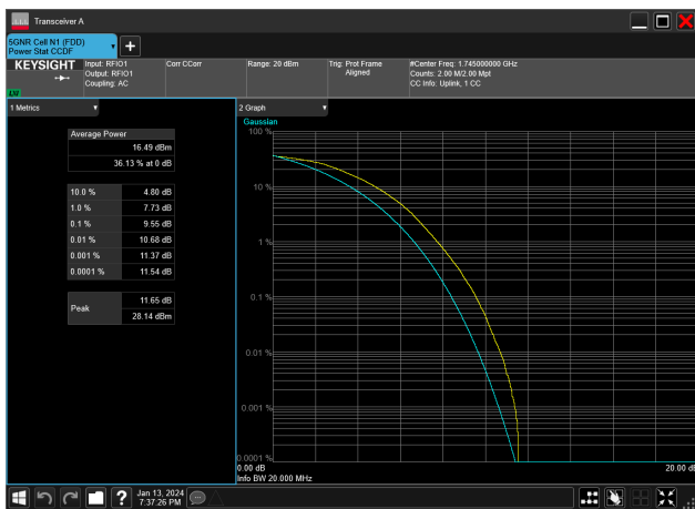
20MHz_15kHz_1745MHz_DFT-s-OFDM 256 QAM_RB100@0&amp;9.55 dB
