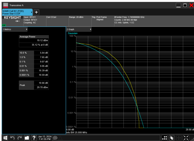
25MHz_15kHz_1745MHz_DFT-s-OFDM 16 QAM_RB128@0&amp;9.07 dB
