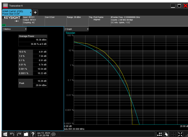
15MHz_15kHz_2535MHz_DFT-s-OFDM 16 QAM_RB75@0&amp;8.91 dB
