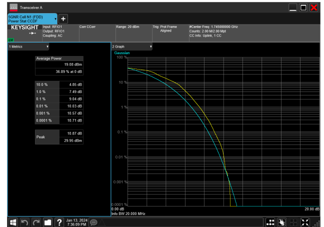
20MHz_15kHz_1745MHz_DFT-s-OFDM 16 QAM_RB100@0&amp;9.04 dB
