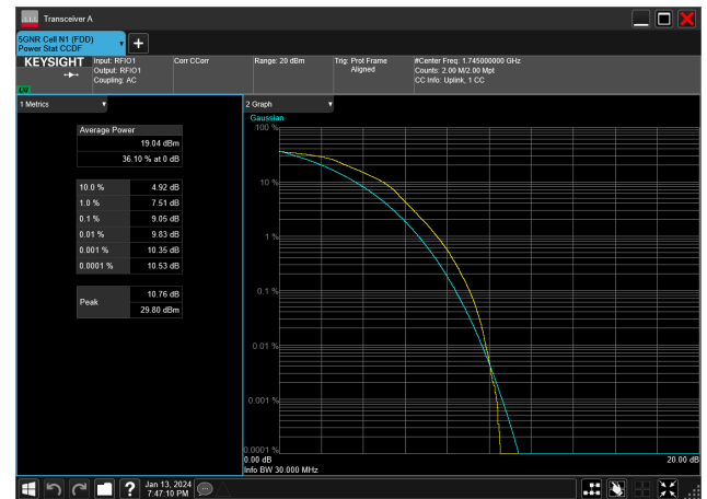
30MHz_15kHz_1745MHz_DFT-s-OFDM 16 QAM_RB160@0&amp;9.05 dB
