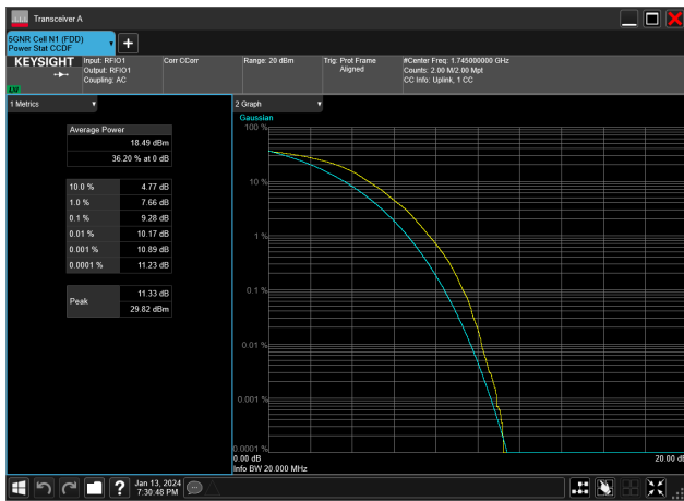
15MHz_15kHz_1745MHz_DFT-s-OFDM 64 QAM_RB75@0&amp;9.28 dB
