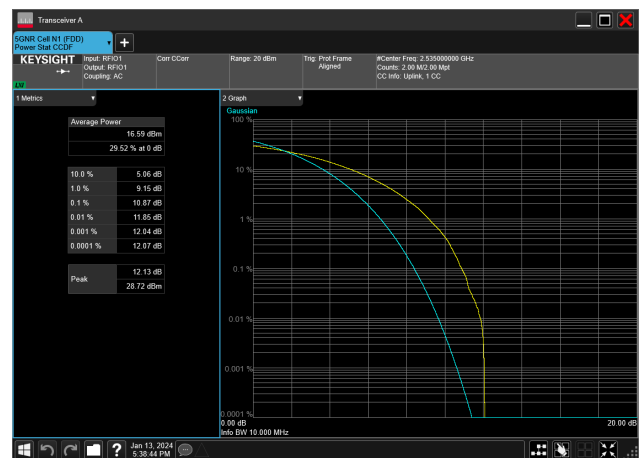
10MHz_15kHz_2535MHz_CP-OFDM 64 QAM_RB52@0&amp;10.87 dB
