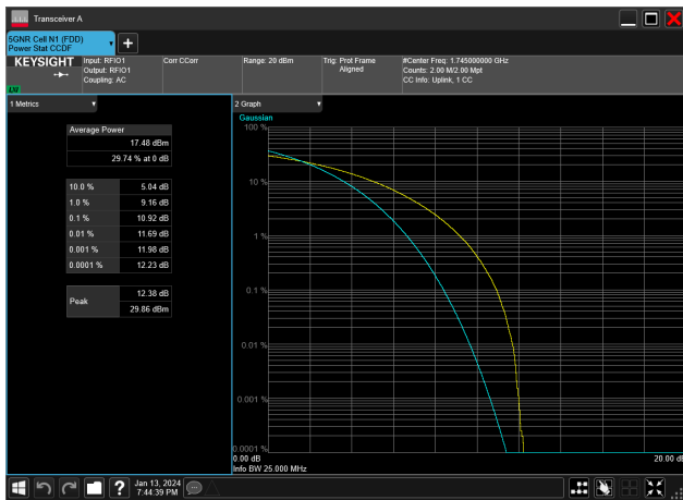
25MHz_15kHz_1745MHz_CP-OFDM 64 QAM_RB133@0&amp;10.92 dB
