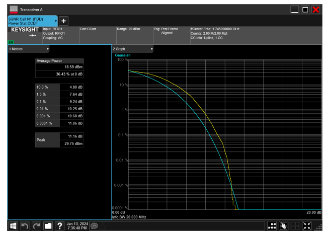
20MHz_15kHz_1745MHz_DFT-s-OFDM 64 QAM_RB100@0&amp;9.24 dB
