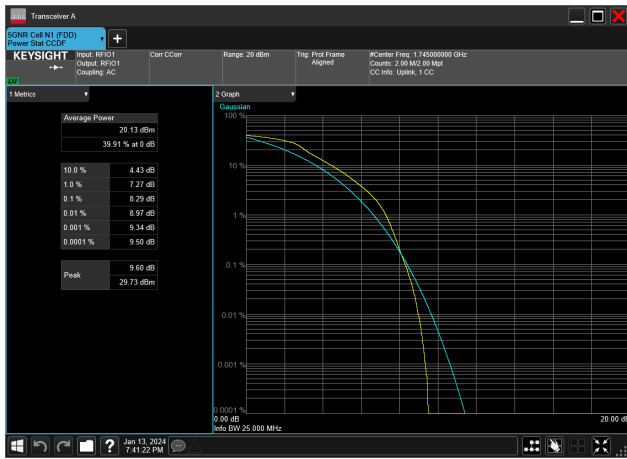
25MHz_15kHz_1745MHz_DFT-s-OFDM QPSK_RB128@0&amp;8.29 dB
