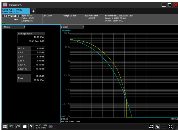
5MHz_15kHz_2535MHz_DFT-s-OFDM 64 QAM_RB25@0&amp;9.15 dB
