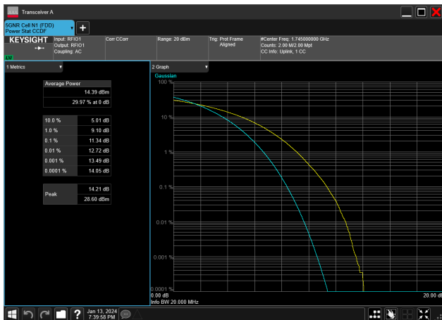
20MHz_15kHz_1745MHz_CP-OFDM 256 QAM_RB106@0&amp;11.34 dB
