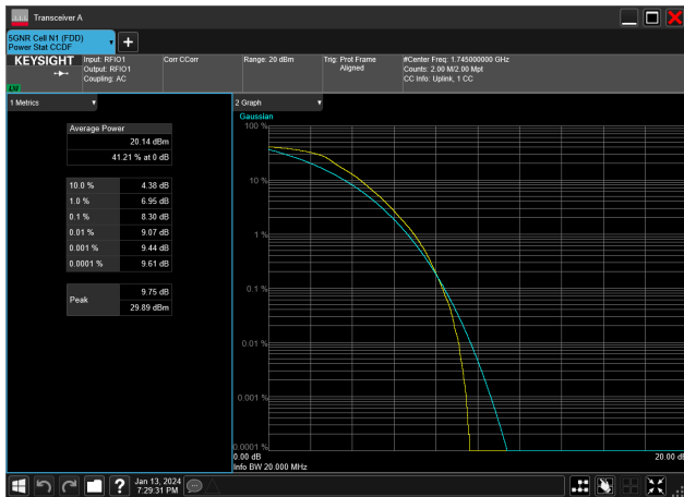
15MHz_15kHz_1745MHz_DFT-s-OFDM QPSK_RB75@0&amp;8.30 dB
