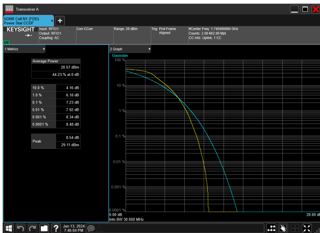
30MHz_15kHz_1745MHz_DFT-s-OFDM PI/2 BPSK_RB160@0&amp;7.23 dB
