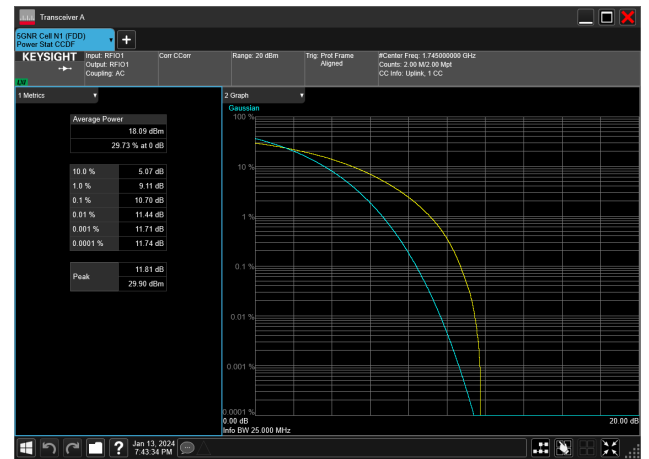
25MHz_15kHz_1745MHz_CP-OFDM QPSK_RB133@0&amp;10.70 dB
