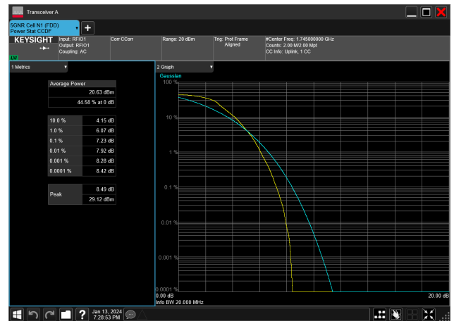
15MHz_15kHz_1745MHz_DFT-s-OFDM PI/2 BPSK_RB75@0&amp;7.23 dB
