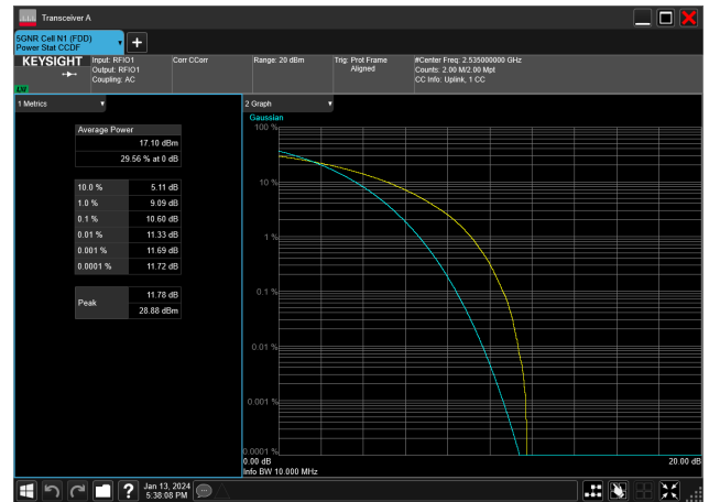
10MHz_15kHz_2535MHz_CP-OFDM 16 QAM_RB52@0&amp;10.60 dB
