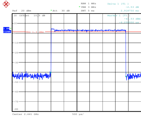
2DH5_Hopping 2.919ms
