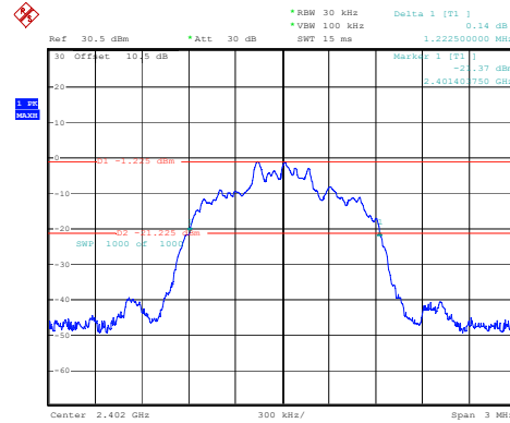
3DH1_Low 1.223MHz
