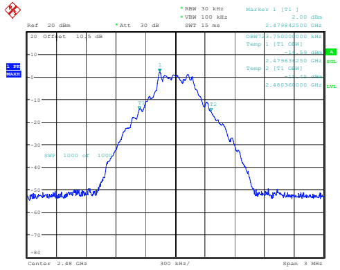
DH1_High 0.724MHz
