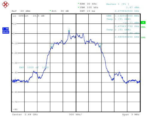
2DH1_High 1.133MHz
