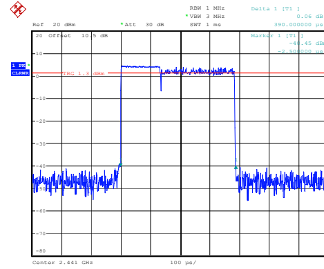
3DH1_Hopping 0.390ms
