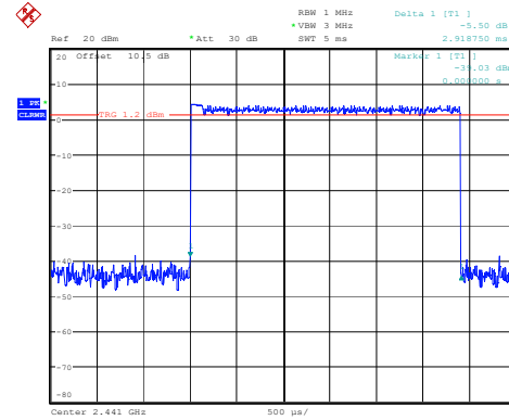
3DH5_Hopping 2.919ms
