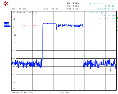
2DH1_Hopping 0.390ms
