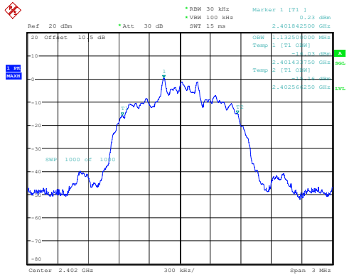
2DH1_Low 1.133MHz
