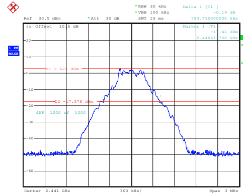
DH1_Middle 0.784MHz
