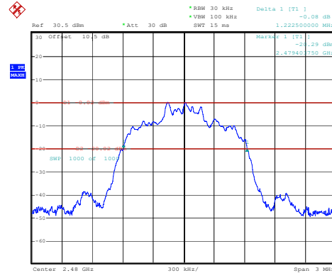
3DH1_High 1.223MHz
