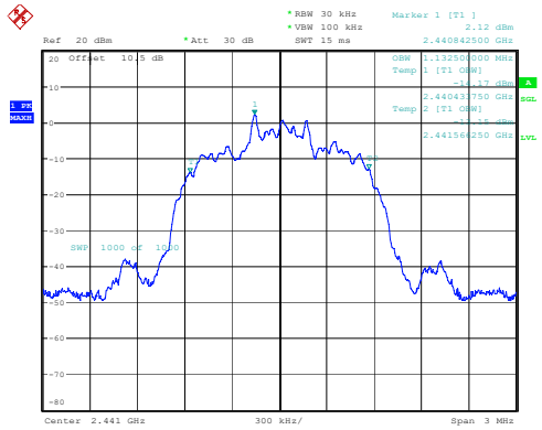
2DH1_Middle 1.133MHz
