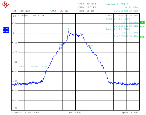
DH1_Low 0.724MHz
