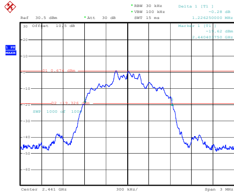
3DH1_Middle 1.226MHz
