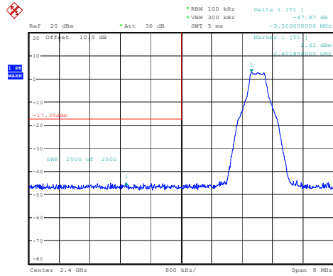
DH1_Low
