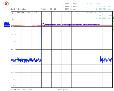
2DH5_Hopping 2.919ms
