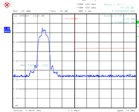
2DH1_High
