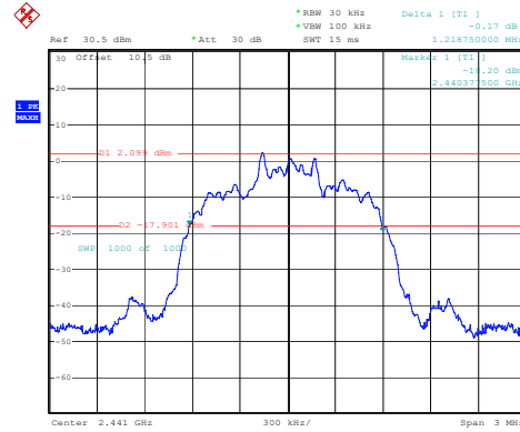
2DH1_Middle 1.219MHz
