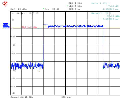
3DH3_Hopping 1.650ms
