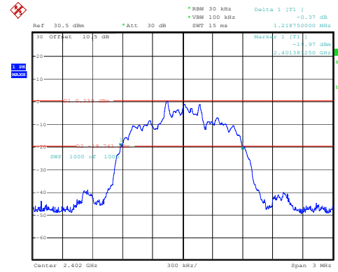
2DH1_Low 1.219MHz
