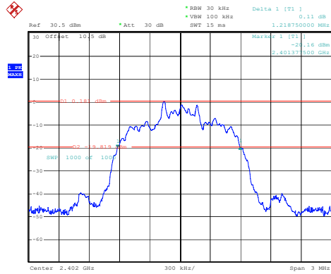
2DH1_Low 1.219MHz
