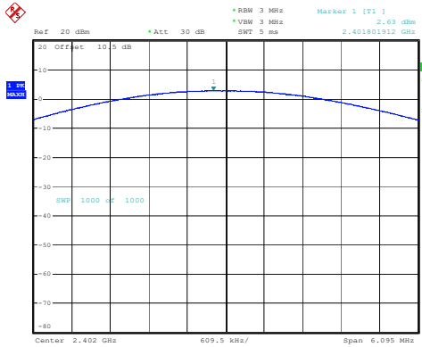
2DH1_Low 2.63dBm
