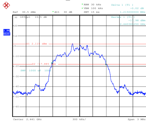
2DH1_Middle 1.215MHz
