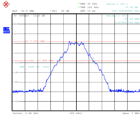
DH1_High 0.784MHz
