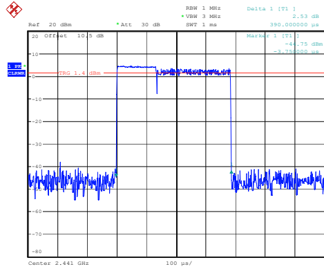
2DH1_Hopping 0.390ms
