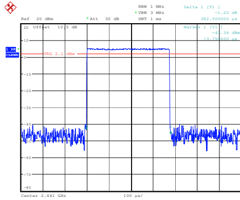
DH1_Hopping 0.383ms
