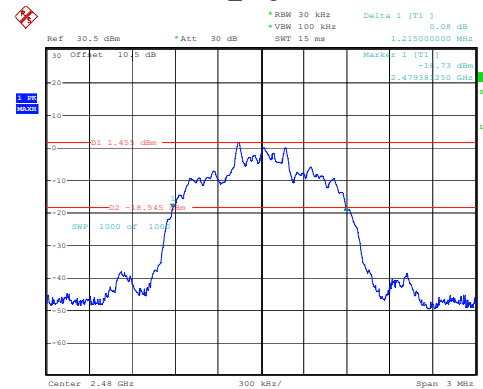
2DH1_High 1.215MHz
