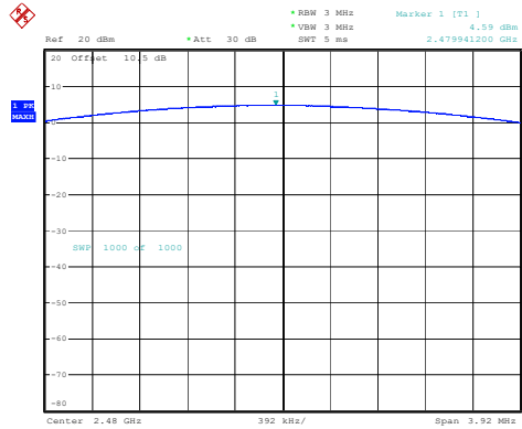
DH1_High 4.59dBm
