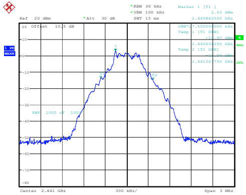
DH1_Middle 0.728MHz
