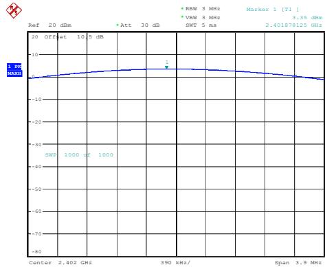
DH1_Low 3.35dBm
