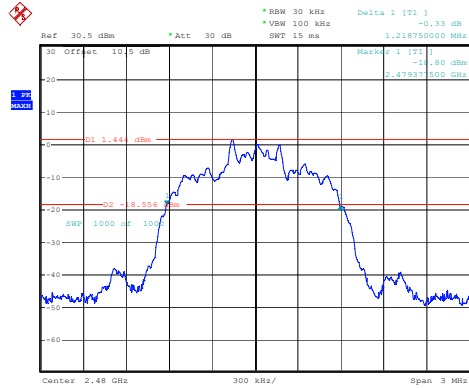
2DH1_High 1.219MHz
