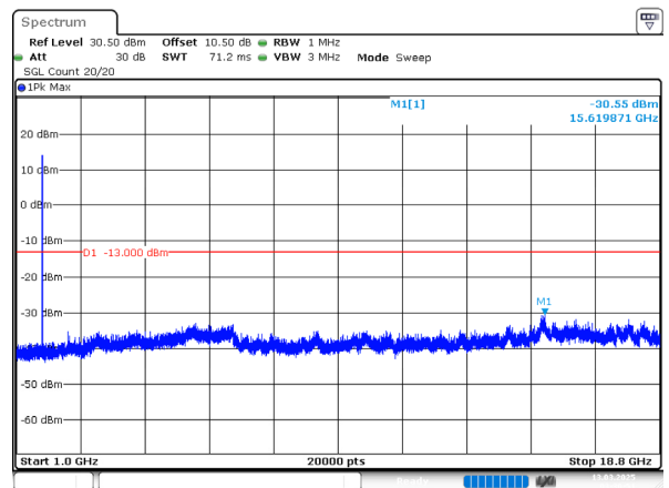
1.4MHz_Low_QPSK_1@0(1GHz~18.8GHz)
