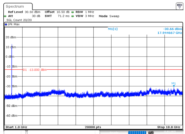
1.4MHz_Low_QPSK_6@0(1GHz~18.8GHz)
