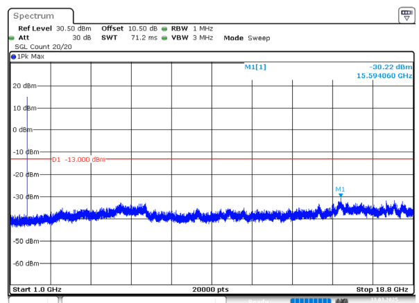
1.4MHz_Middle_QPSK_1@0(1GHz~18.8GHz)
