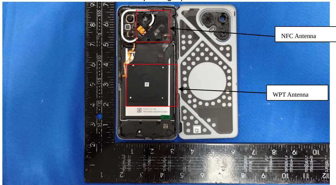
Internal photograph of EUT
