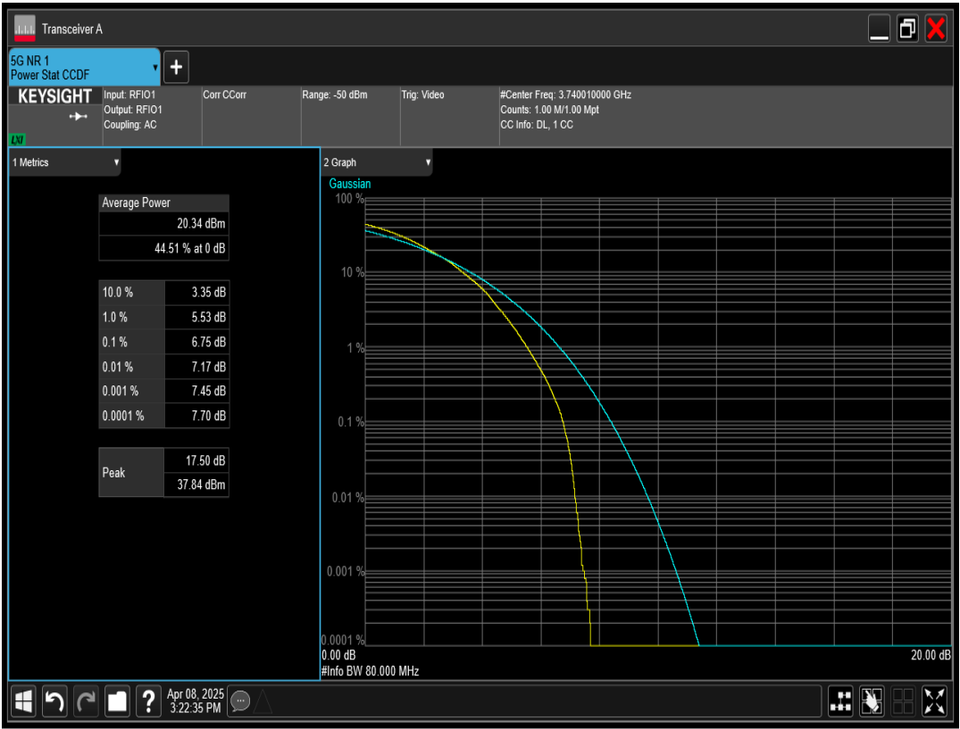
n78(3700-3800) SCS=30kHz DFT_QAM64 BW=80MHz Channel=649334 RB=216@0
