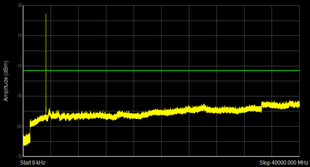
n77 SCS=30kHz CP_QPSK BW=10MHz Channel=620334 RB=1@23
