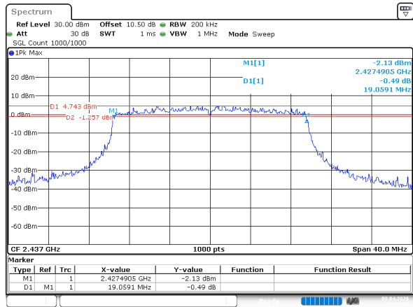
802.11ax20_2437MHz_RU_Full_Chain 0
