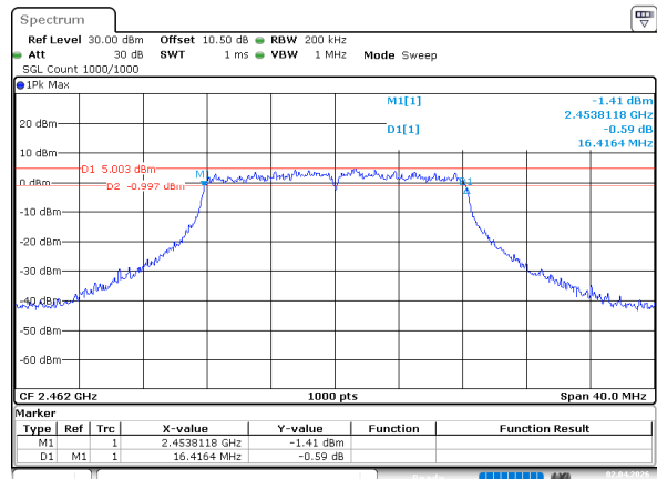
802.11g_2462MHz_Chain 0
