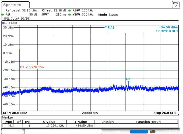
802.11g_2462MHz_Chain 0
