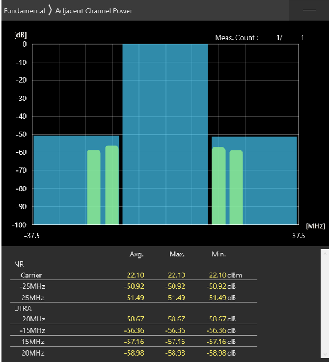
25MHz_30kHz_3687.5MHz-OFDM QPSK_RB32@16 -50.92,-51.49dB
