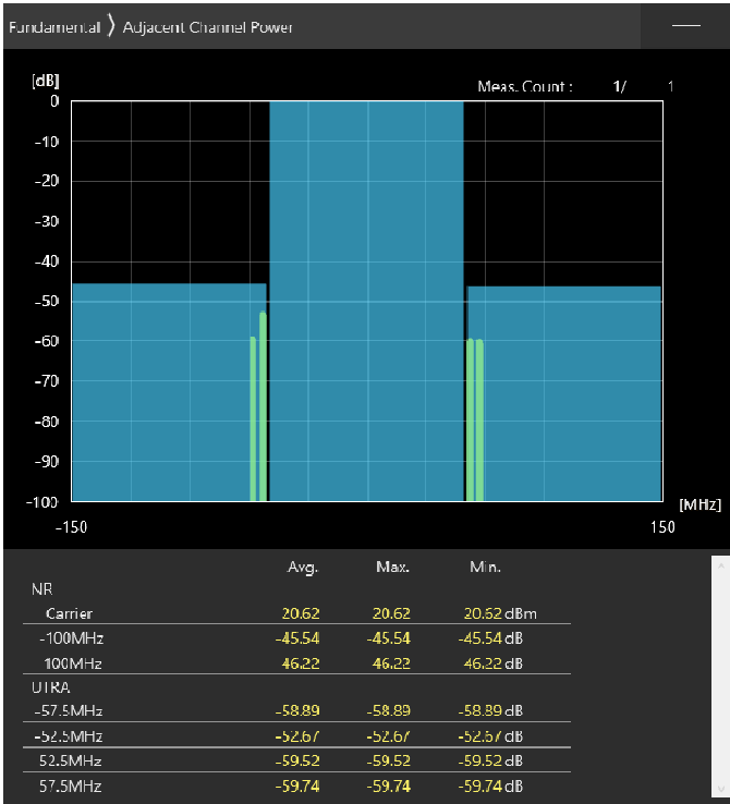
100MHz_30kHz_3600MHz-OFDM QPSK_RB1@0 -45.54,-46.22dB
