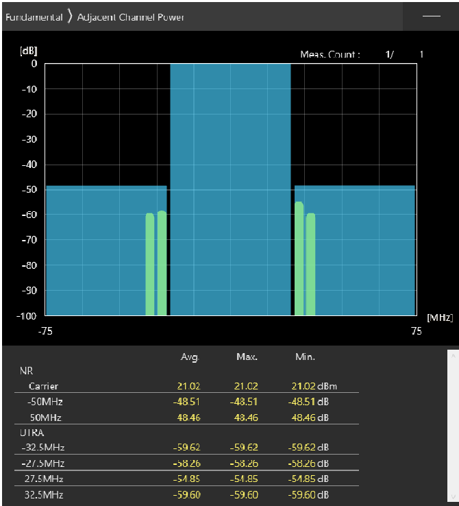
50MHz_30kHz_3575MHz-OFDM QPSK_RB1@132 -48.51,-48.46dB
