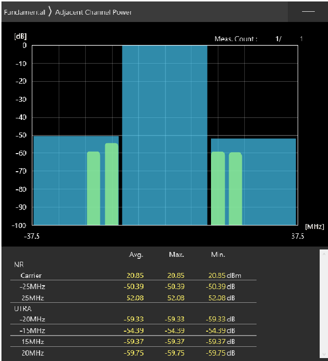
25MHz_30kHz_3562.5MHz-OFDM QPSK_RB1@0 -50.39,-52.08dB
