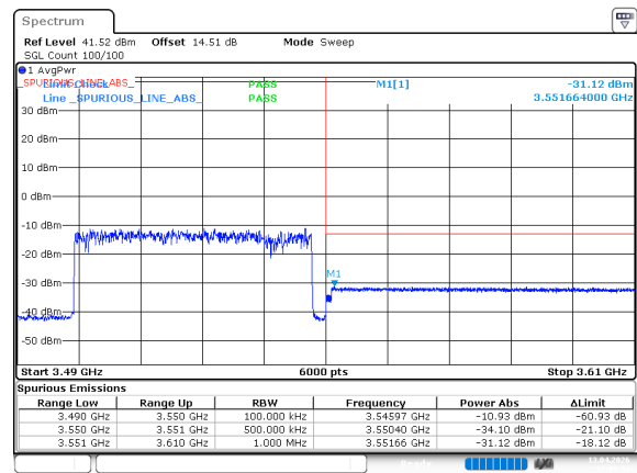
n77_1_50MHz_30kHz_3525MHz_DFT-s-OFDM QPSK_RB128@0
