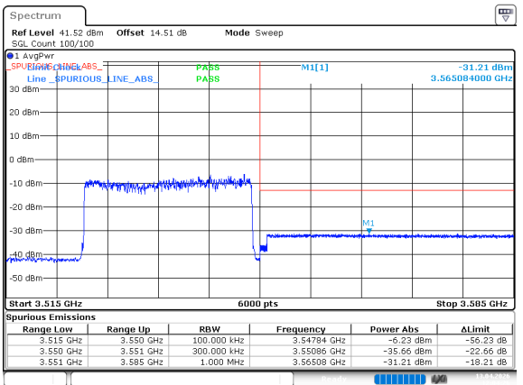
n77_1_25MHz_30kHz_3537.5MHz_DFT-s-OFDM QPSK_RB64@0
