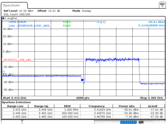
n77_1_25MHz_30kHz_3462.5MHz_DFT-s-OFDM QPSK_RB64@0
