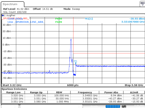
n77_1_20MHz_30kHz_3540MHz_DFT-s-OFDM QPSK_RB1@50
