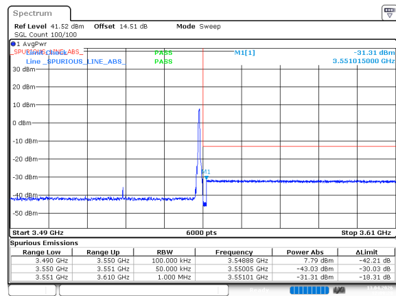
n77_1_50MHz_30kHz_3525MHz_DFT-s-OFDM QPSK_RB1@132
