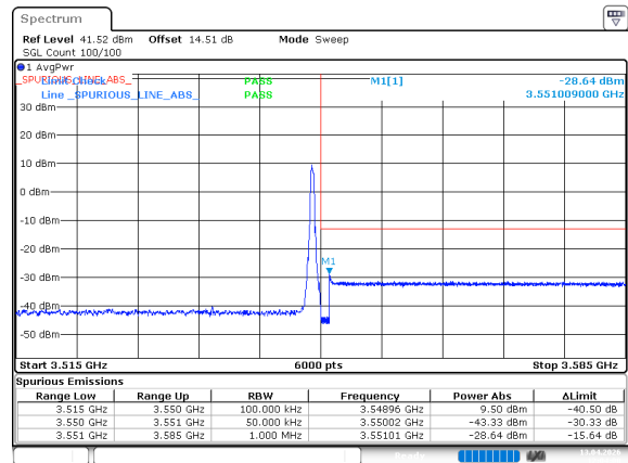
n77_1_25MHz_30kHz_3537.5MHz_DFT-s-OFDM QPSK_RB1@64
