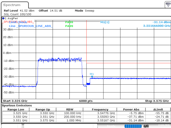
n77_1_15MHz_30kHz_3542.5MHz_DFT-s-OFDM QPSK_RB36@0
