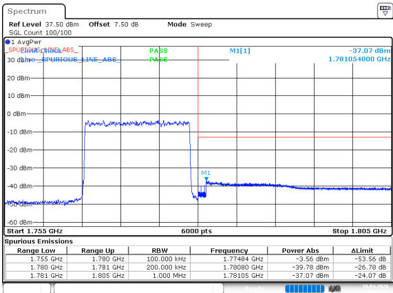
n66_15MHz_15kHz_1772.5MHz_DFT-s-OFDM QPSK_RB75@0
