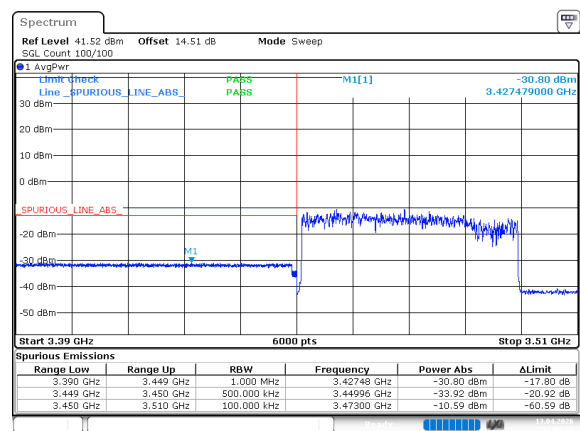
n77_1_50MHz_30kHz_3475MHz_DFT-s-OFDM QPSK_RB128@0
