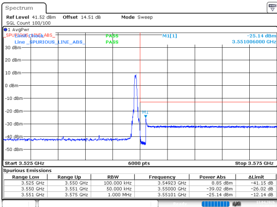
n77_1_15MHz_30kHz_3542.5MHz_DFT-s-OFDM QPSK_RB1@37
