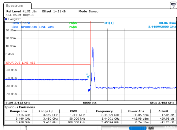
n77_1_25MHz_30kHz_3462.5MHz_DFT-s-OFDM QPSK_RB1@0
