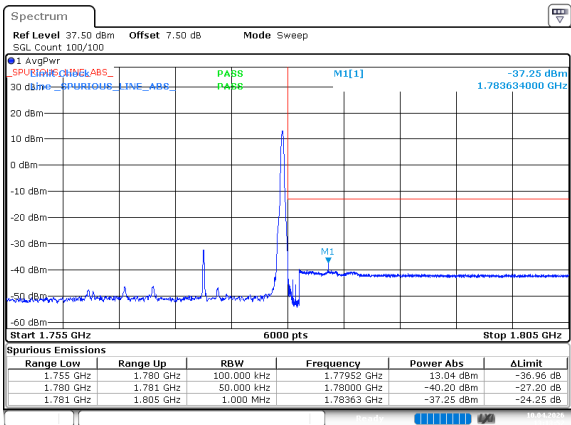
n66_15MHz_15kHz_1772.5MHz_DFT-s-OFDM QPSK_RB1@78
