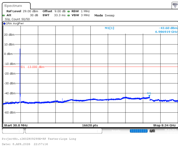
n5_20MHz_15kHz_834MHz_DFT-s-OFDM QPSK_RB100@0 -43.60dBm
