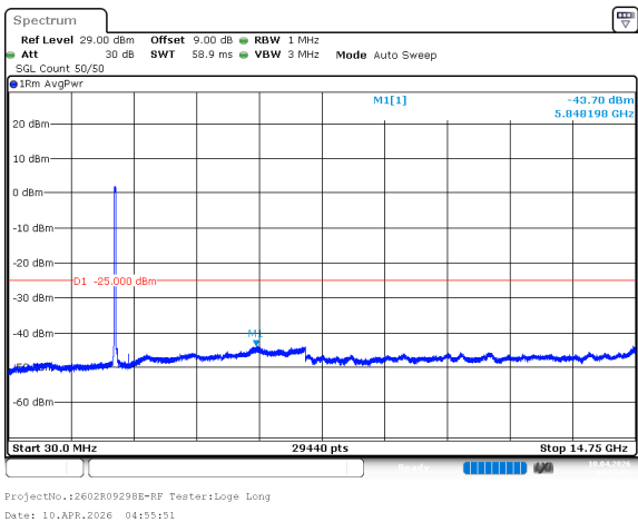
n7_50MHz_15kHz_2525MHz_DFT-s-OFDM QPSK_RB270@0 -43.70dBm
