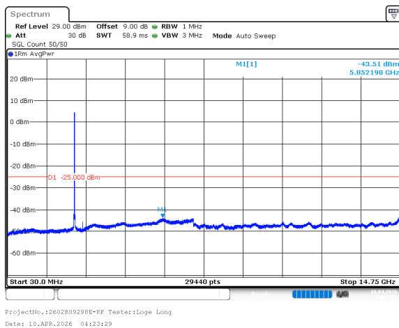
n7_25MHz_15kHz_2535MHz_DFT-s-OFDM QPSK_RB128@0 -43.51dBm
