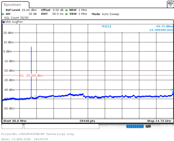
n7_20MHz_15kHz_2510MHz_DFT-s-OFDM QPSK_RB100@0 -43.72dBm
