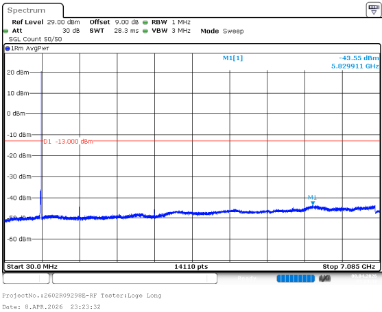
n12_15MHz_15kHz_708.5MHz_DFT-s-OFDM QPSK_RB1@78 -43.55dBm
