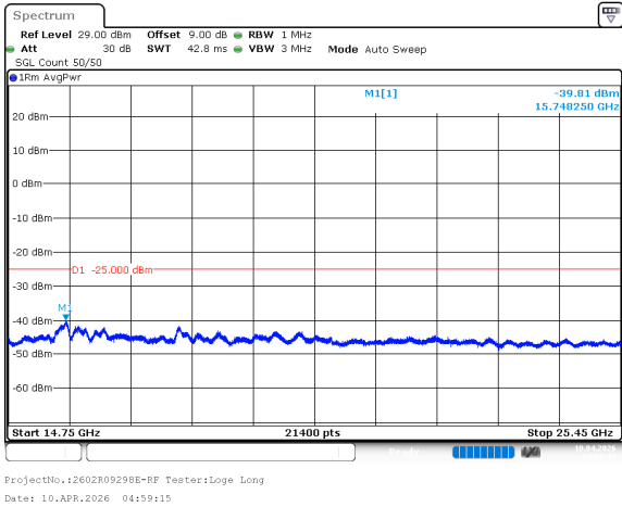
n7_50MHz_15kHz_2545MHz_DFT-s-OFDM QPSK_RB1@269 -39.71dBm
