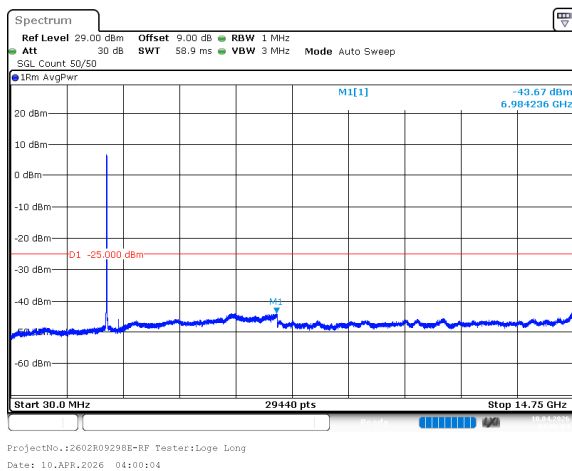
n7_15MHz_15kHz_2535MHz_DFT-s-OFDM QPSK_RB75@0 -43.67dBm
