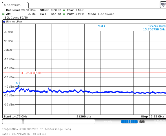
n7_30MHz_15kHz_2535MHz_DFT-s-OFDM QPSK_RB160@0 -39.91dBm
