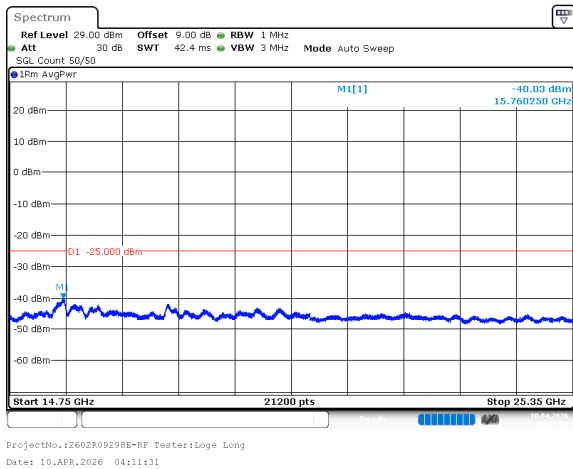
n7_20MHz_15kHz_2535MHz_DFT-s-OFDM QPSK_RB100@0 -40.03dBm
