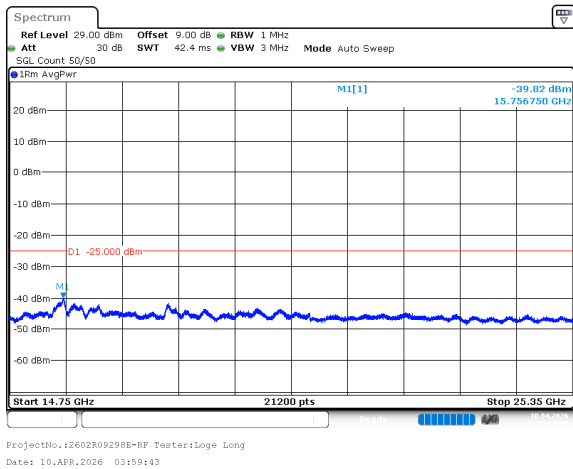
n7_15MHz_15kHz_2535MHz_DFT-s-OFDM QPSK_RB75@0 -39.82dBm
