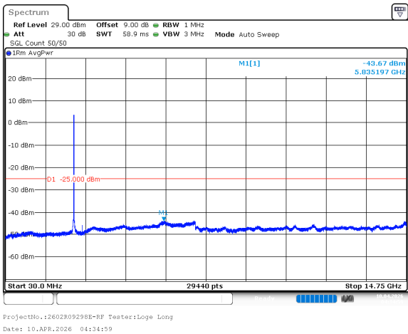
n7_30MHz_15kHz_2535MHz_DFT-s-OFDM QPSK_RB160@0 -43.67dBm
