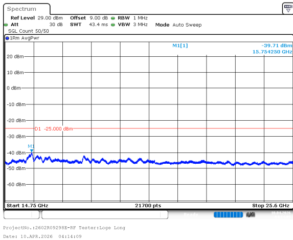
n7_20MHz_15kHz_2560MHz_DFT-s-OFDM QPSK_RB100@0 -39.71dBm
