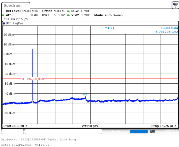
n7_20MHz_15kHz_2560MHz_DFT-s-OFDM QPSK_RB100@0 -43.83dBm
