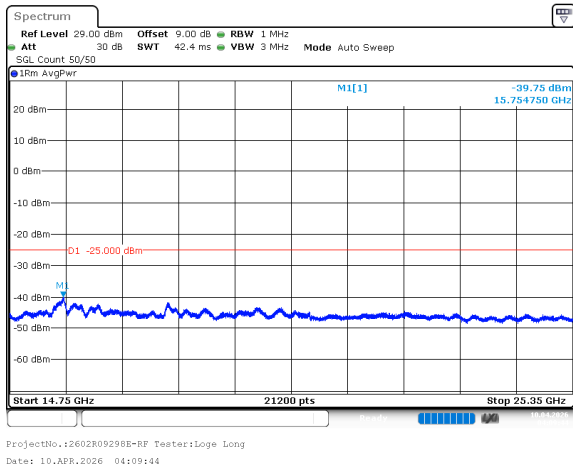
n7_20MHz_15kHz_2535MHz_DFT-s-OFDM QPSK_RB1@105 -40dBm
