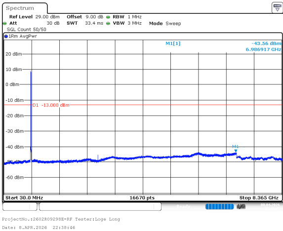
n5_10MHz_15kHz_844MHz_DFT-s-OFDM QPSK_RB1@51 -43.60dBm
