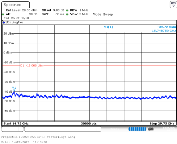
n77_3_60MHz_30kHz_3840MHz_DFT-s-OFDM QPSK_RB162@0 -39.72dBm
