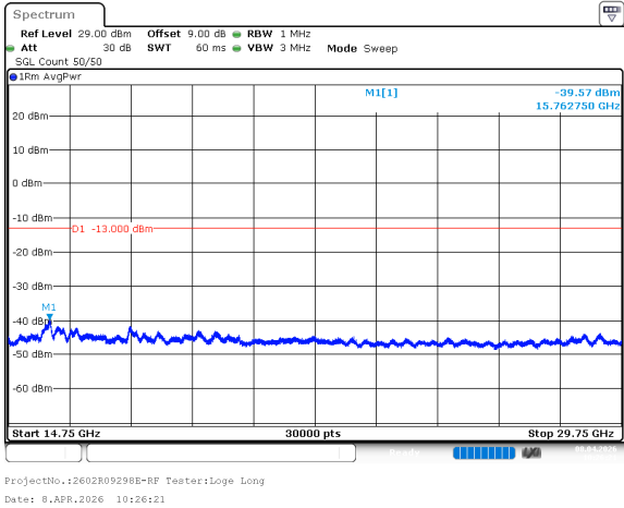
n77_3_25MHz_30kHz_3712.5MHz_DFT-s-OFDM QPSK_RB1@64 -39.57dBm
