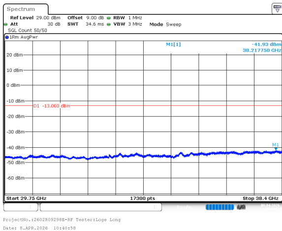
n77_3_30MHz_30kHz_3840MHz_DFT-s-OFDM QPSK_RB1@77 -41.93dBm
