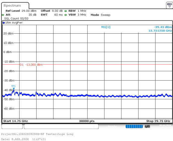
n77_3_70MHz_30kHz_3945MHz_DFT-s-OFDM QPSK_RB180@0 -39.43dBm
