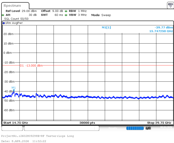
n77_3_80MHz_30kHz_3840MHz_DFT-s-OFDM QPSK_RB1@0 -39.77dBm
