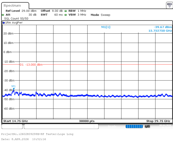
n77_3_40MHz_30kHz_3840MHz_DFT-s-OFDM QPSK_RB100@0 -39.67dBm
