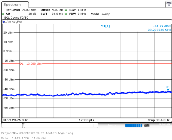
n77_3_80MHz_30kHz_3840MHz_DFT-s-OFDM QPSK_RB216@0 -41.77dBm
