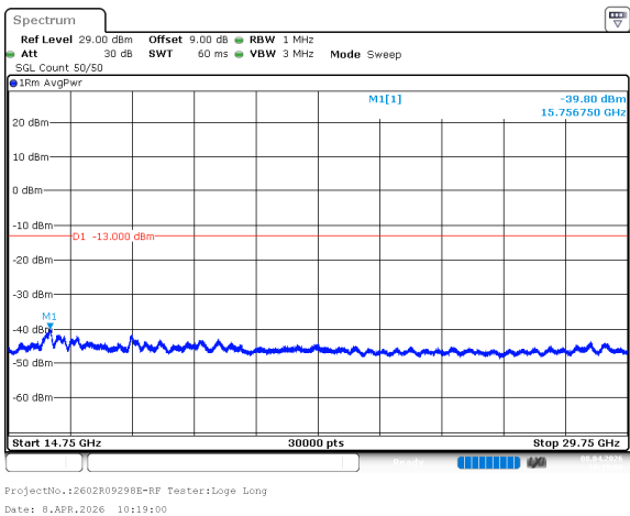
n77_3_20MHz_30kHz_3840MHz_DFT-s-OFDM QPSK_RB1@50 -39.80dBm
