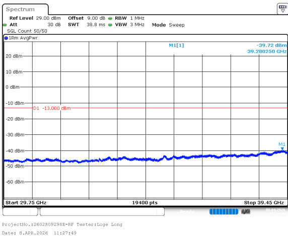
n77_3_70MHz_30kHz_3945MHz_DFT-s-OFDM QPSK_RB180@0 -39.72dBm
