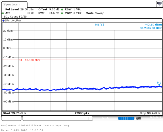
n77_3_25MHz_30kHz_3840MHz_DFT-s-OFDM QPSK_RB1@0 -42.10dBm
