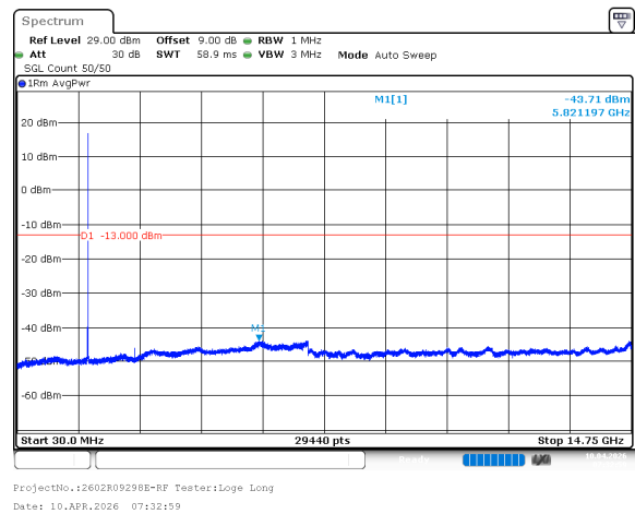
n66_15MHz_15kHz_1717.5MHz_DFT-s-OFDM QPSK_RB1@78 -43.71dBm
