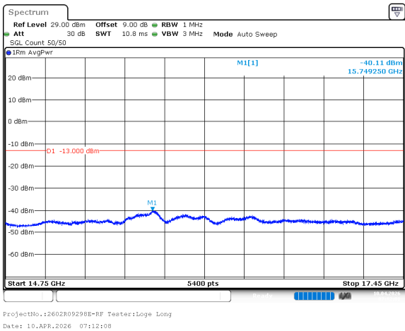
n66_5MHz_15kHz_1745MHz_DFT-s-OFDM QPSK_RB1@0 -40.11dBm
