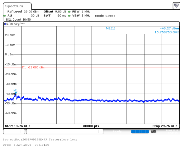
n77_1_10MHz_30kHz_3500MHz_DFT-s-OFDM QPSK_RB1@23 -40.27dBm
