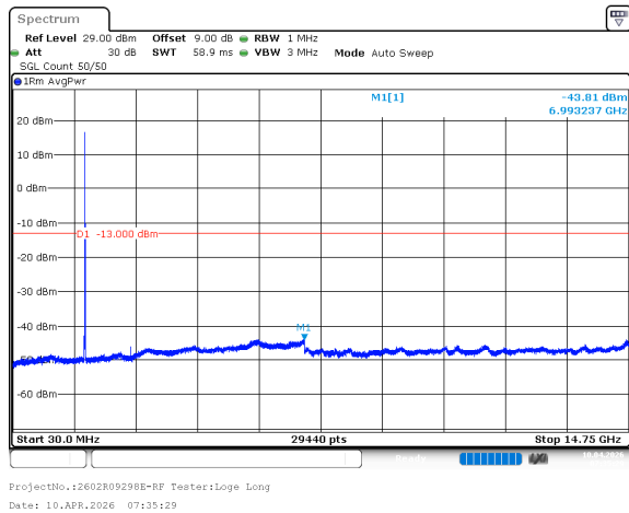
n66_15MHz_15kHz_1745MHz_DFT-s-OFDM QPSK_RB1@78 -43.81dBm
