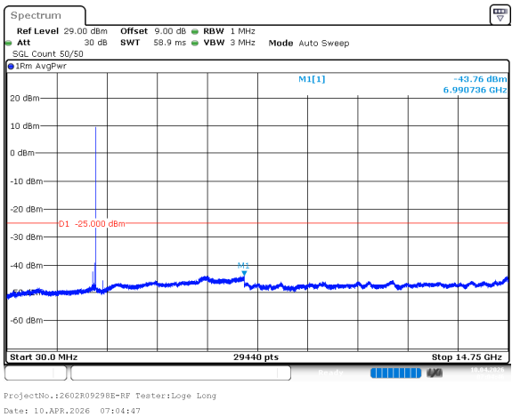
n41_100MHz_30kHz_2592.99MHz_DFT-s-OFDM QPSK_RB1@272 -43.76dBm
