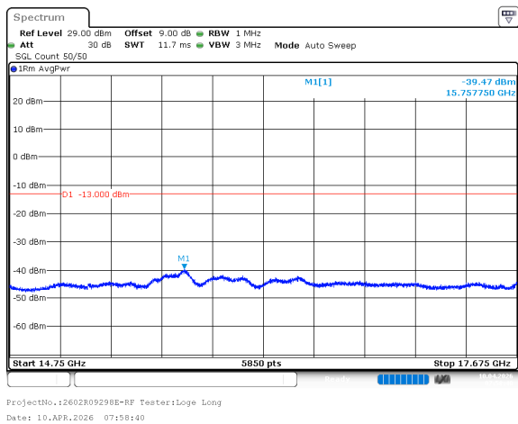
n66_25MHz_15kHz_1767.5MHz_DFT-s-OFDM QPSK_RB1@0 -39.47dBm
