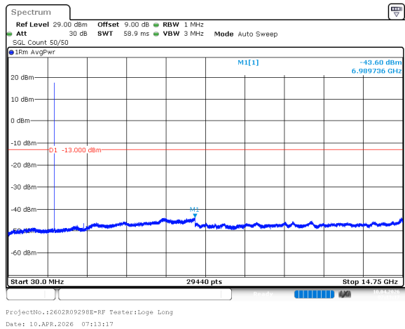
n66_5MHz_15kHz_1745MHz_DFT-s-OFDM QPSK_RB1@24 -43.60dBm
