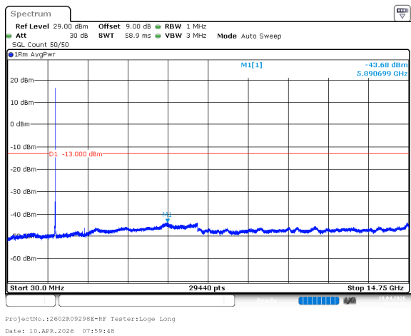
n66_25MHz_15kHz_1767.5MHz_DFT-s-OFDM QPSK_RB1@132 -43.68dBm
