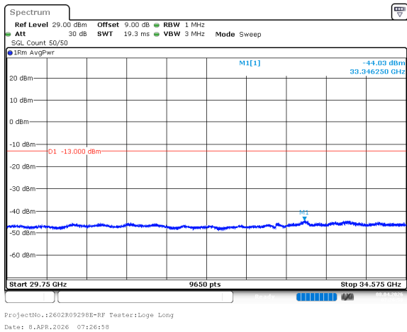
n77_1_15MHz_30kHz_3457.5MHz_DFT-s-OFDM QPSK_RB1@37 -44.03dBm
