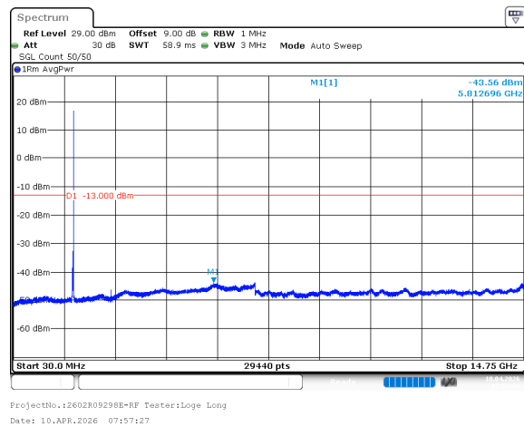
n66_25MHz_15kHz_1745MHz_DFT-s-OFDM QPSK_RB1@132 -43.56dBm
