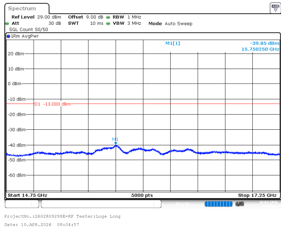
n66_30MHz_15kHz_1725MHz_DFT-s-OFDM QPSK_RB1@0 -39.85dBm
