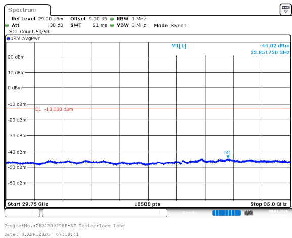
n77_1_10MHz_30kHz_3500MHz_DFT-s-OFDM QPSK_RB1@23 -44.02dBm
