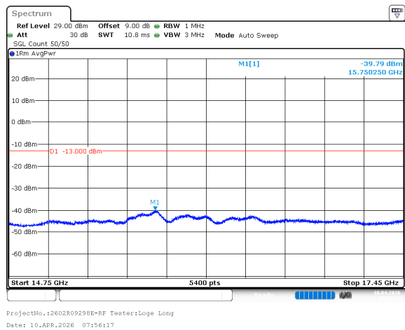
n66_25MHz_15kHz_1745MHz_DFT-s-OFDM QPSK_RB1@0 -39.79dBm
