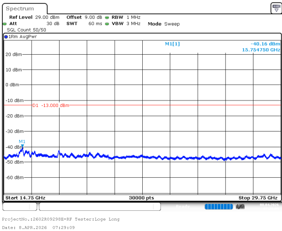
n77_1_15MHz_30kHz_3500MHz_DFT-s-OFDM QPSK_RB1@0 -40.16dBm
