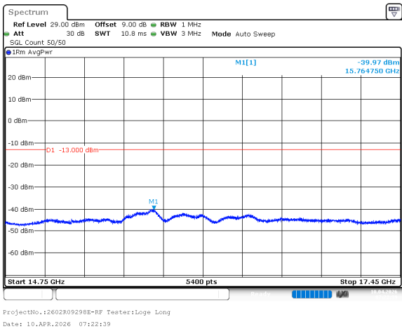
n66_10MHz_15kHz_1745MHz_DFT-s-OFDM QPSK_RB1@0 -39.97dBm
