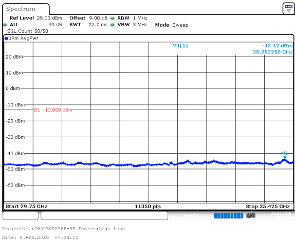
n77_1_15MHz_30kHz_3542.5MHz_DFT-s-OFDM QPSK_RB1@37 -43.42dBm
