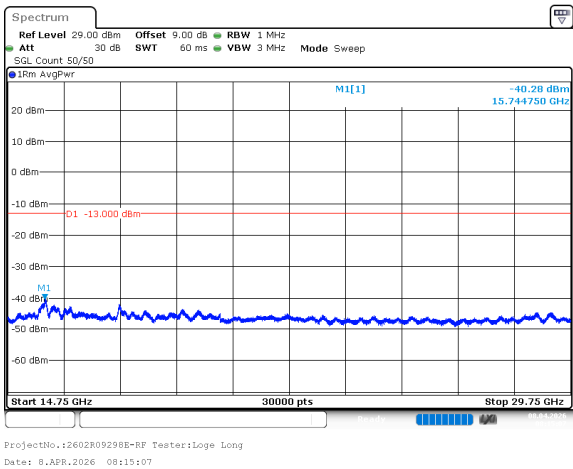
n77_1_40MHz_30kHz_3500MHz_DFT-s-OFDM QPSK_RB100@0 -40.28dBm
