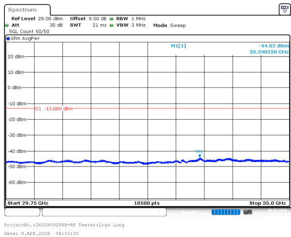
n77_1_30MHz_30kHz_3500MHz_DFT-s-OFDM QPSK_RB1@77 -44.02dBm
