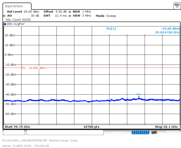
n77_1_80MHz_30kHz_3510MHz_DFT-s-OFDM QPSK_RB1@216 -43.68dBm
