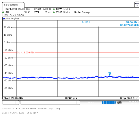
n77_1_80MHz_30kHz_3500MHz_DFT-s-OFDM QPSK_RB216@0 -43.56dBm
