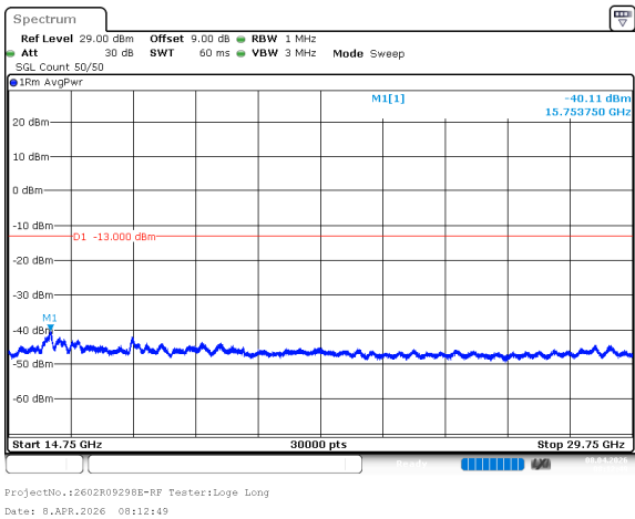
n77_1_40MHz_30kHz_3500MHz_DFT-s-OFDM QPSK_RB1@0 -40.11dBm
