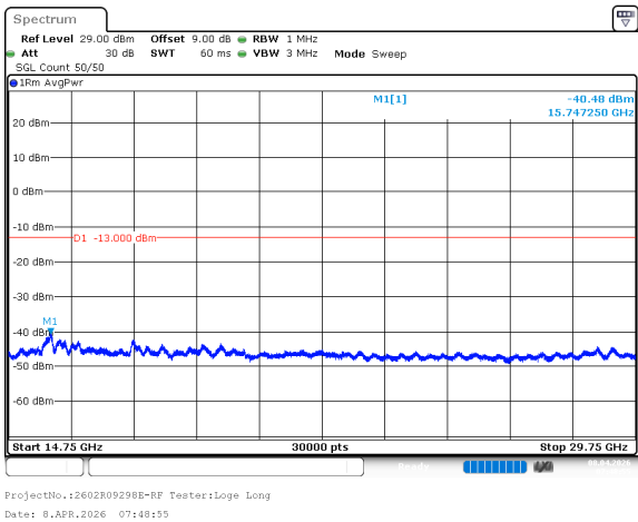
n77_1_25MHz_30kHz_3462.5MHz_DFT-s-OFDM QPSK_RB1@64 -40.48dBm
