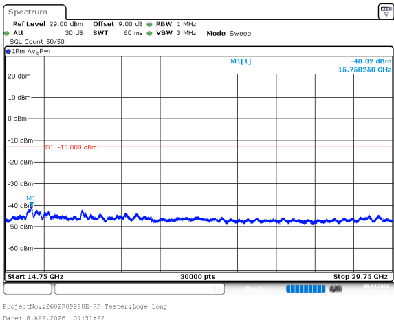
n77_1_25MHz_30kHz_3500MHz_DFT-s-OFDM QPSK_RB1@0 -40.32dBm
