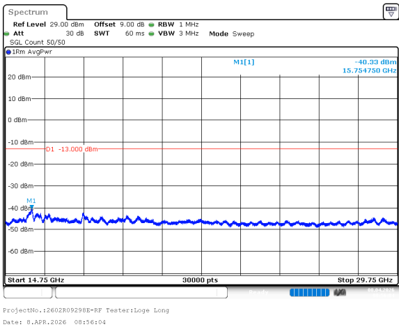
n77_1_80MHz_30kHz_3500MHz_DFT-s-OFDM QPSK_RB1@0 -40.33dBm
