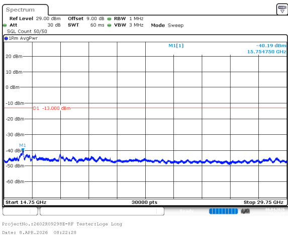
n77_1_50MHz_30kHz_3475MHz_DFT-s-OFDM QPSK_RB128@0 -40.19dBm
