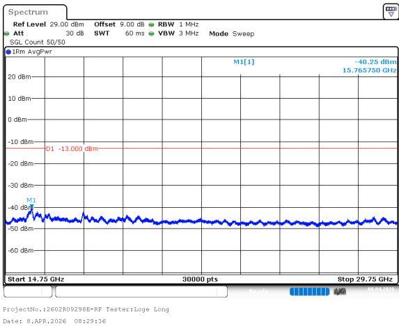
n77_1_50MHz_30kHz_3525MHz_DFT-s-OFDM QPSK_RB128@0 -40.25dBm
