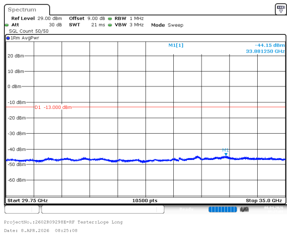
n77_1_50MHz_30kHz_3500MHz_DFT-s-OFDM QPSK_RB1@132 -44.15dBm
