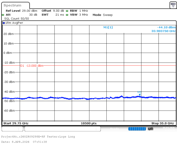
n77_1_25MHz_30kHz_3500MHz_DFT-s-OFDM QPSK_RB1@0 -44.10dBm
