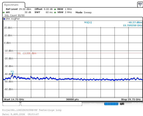
n77_1_80MHz_30kHz_3490MHz_DFT-s-OFDM QPSK_RB1@216 -40.27dBm
