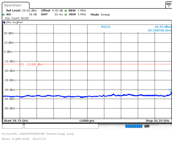
n77_1_50MHz_30kHz_3525MHz_DFT-s-OFDM QPSK_RB1@0 -43.53dBm
