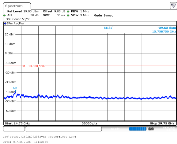
n77_3_70MHz_30kHz_3840MHz_DFT-s-OFDM QPSK_RB1@188 -39.63dBm
