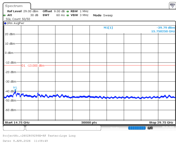
n77_3_60MHz_30kHz_3730MHz_DFT-s-OFDM QPSK_RB1@161 -39.79dBm
