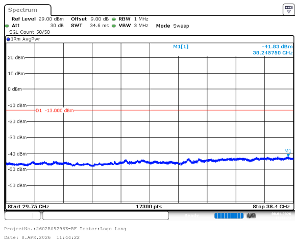
n77_3_90MHz_30kHz_3840MHz_DFT-s-OFDM QPSK_RB1@244 -41.83dBm
