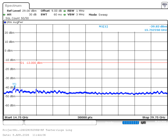
n77_3_90MHz_30kHz_3840MHz_DFT-s-OFDM QPSK_RB1@244 -39.83dBm
