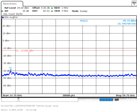
n78_1_15MHz_30kHz_3457.5MHz_DFT-s-OFDM QPSK_RB1@37 -39.73dBm
