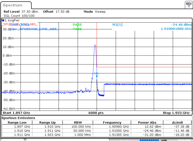
3MHz_High_QPSK_1@14
