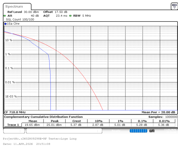
5MHz_Middle_QPSK_1@0
