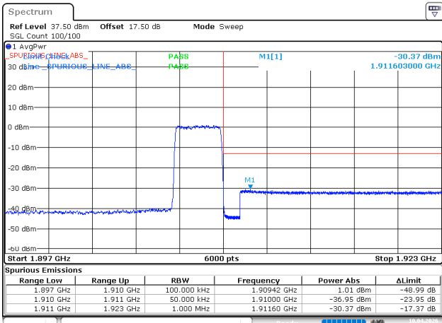
3MHz_High_QPSK_15@0
