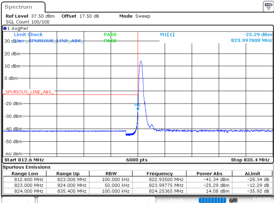
1.4MHz_Low_16QAM_1@0
