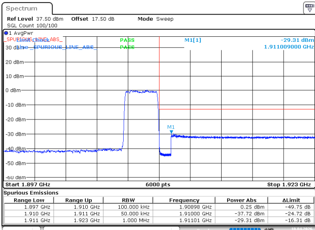
3MHz_High_16QAM_15@0
