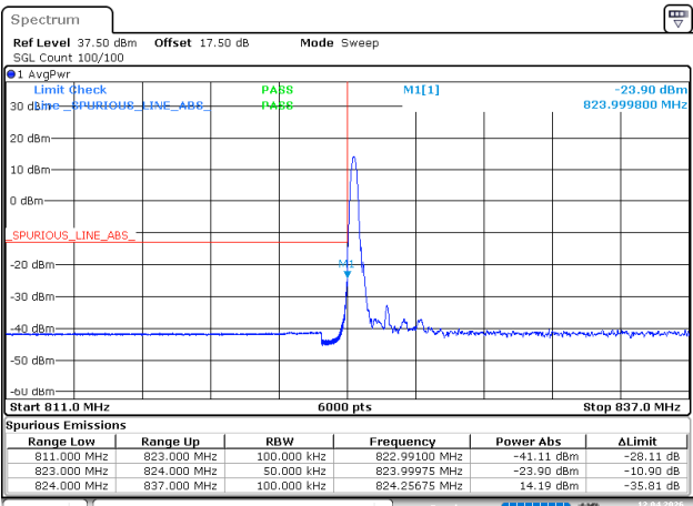
3MHz_Low_16QAM_1@0
