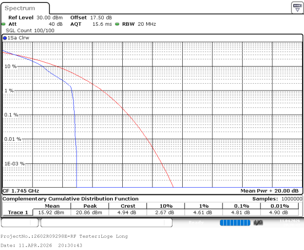
15MHz_Middle_16QAM_1@0
