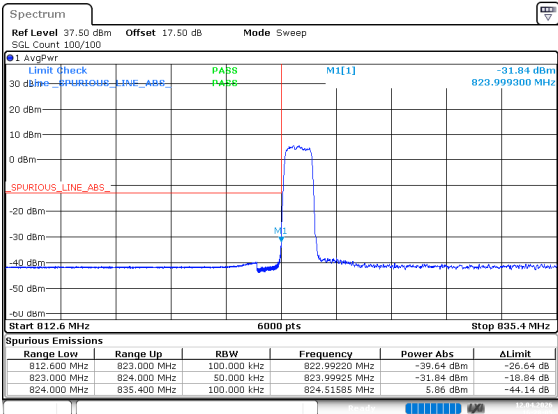
1.4MHz_Low_16QAM_6@0
