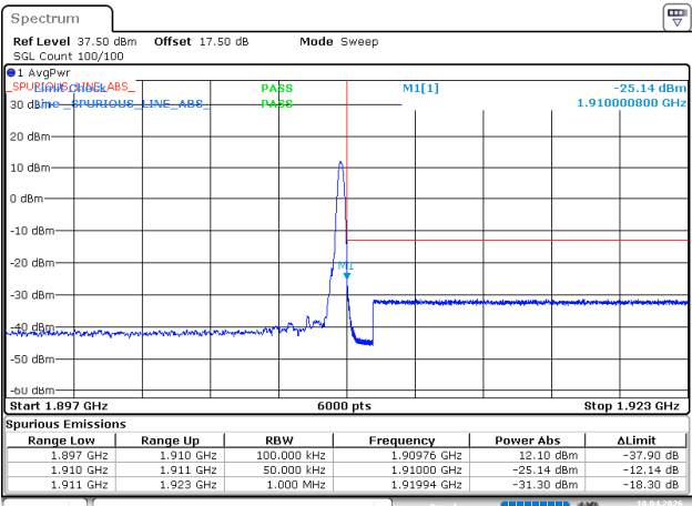
3MHz_High_16QAM_1@14
