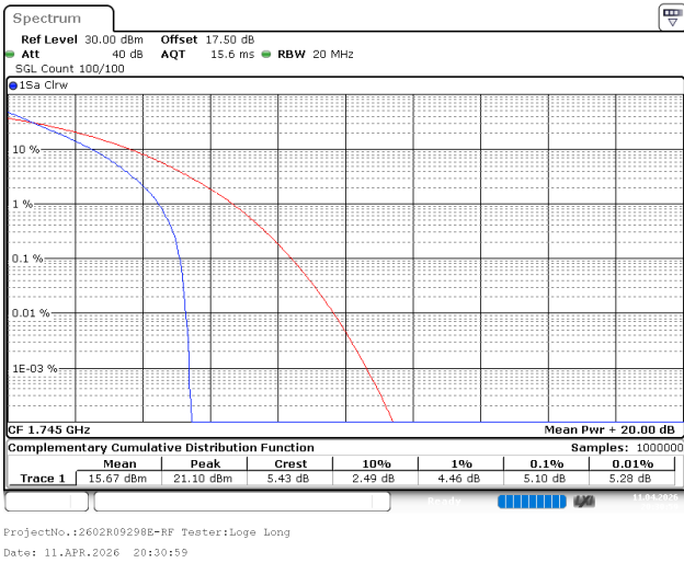
15MHz_Middle_16QAM_75@0
