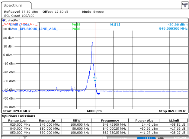
10MHz_High_QPSK_1@49
