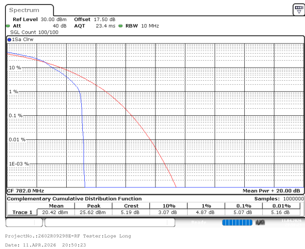
10MHz_Middle_16QAM_1@0
