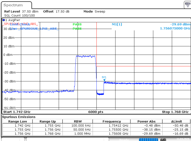
3MHz_High_16QAM_15@0
