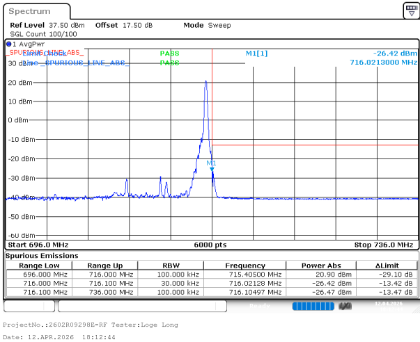
10MHz_High_16QAM_1@49
