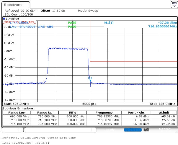
10MHz_High_16QAM_50@0
