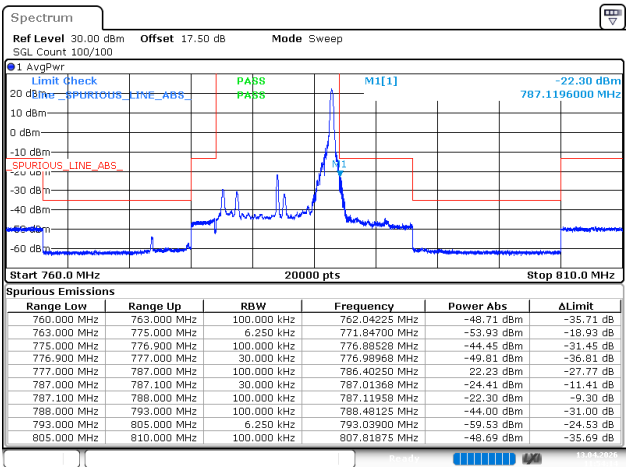
10MHz_Middle_16QAM_1@49
