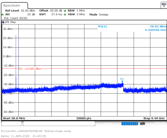
3MHz_High_QPSK_1@(30MHz~9.49GHz)
