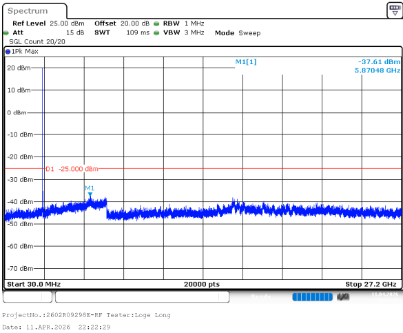
10MHz_High_QPSK_1@0(30MHz~27.2GHz)
