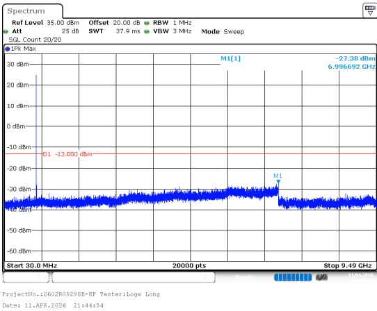
3MHz_Low_QPSK_1@(30MHz~9.49GHz)
