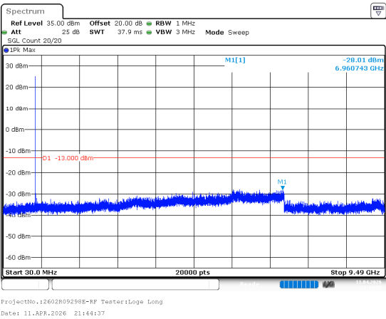
1.4MHz_High_QPSK_1@(30MHz~9.49GHz)
