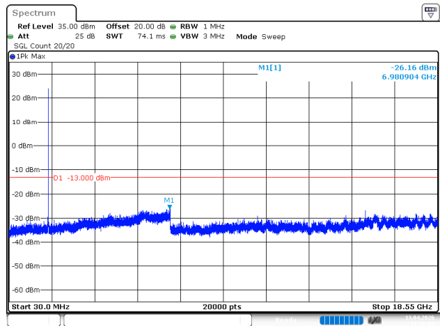
20MHz_Low_QPSK_1@0(30MHz~18.55GHz)
