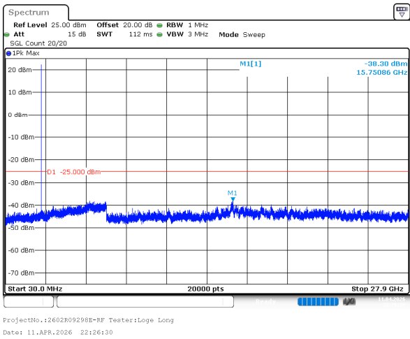
5MHz_High_QPSK_1@0(30MHz~27.9GHz)
