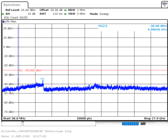
10MHz_Middle_QPSK_1@0(30MHz~27.9GHz)
