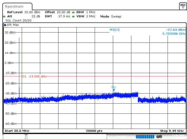
10MHz_Middle_QPSK_1@0(30MHz~9.49GHz)
