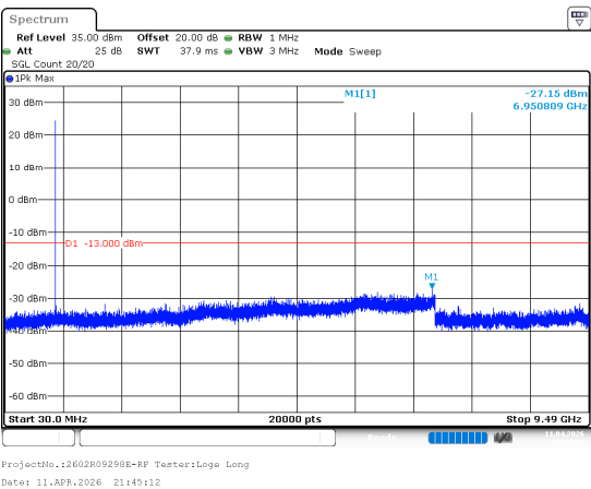
3MHz_Middle_QPSK_1@(30MHz~9.49GHz)
