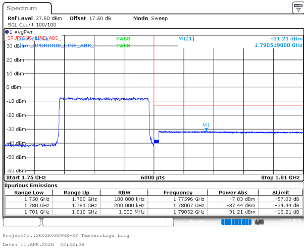
20MHz_High_16QAM_100@0
