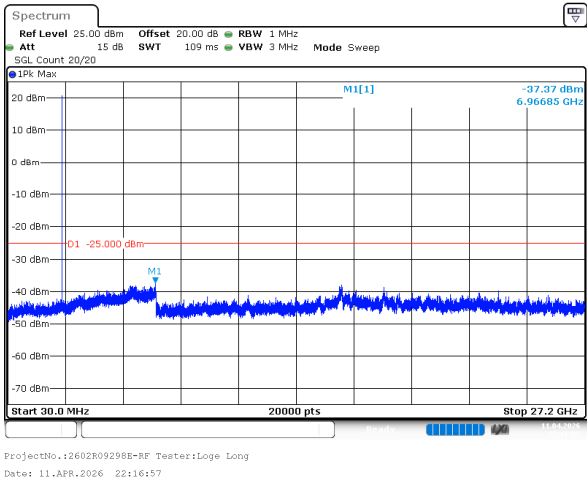
5MHz_High_QPSK_1@0(30MHz~27.2GHz)
