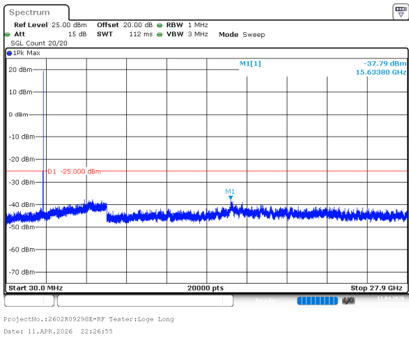
10MHz_Low_QPSK_1@0(30MHz~27.9GHz)
