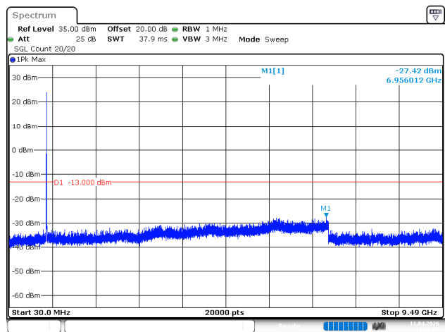
10MHz_High_QPSK_1@0(30MHz~9.49GHz)
