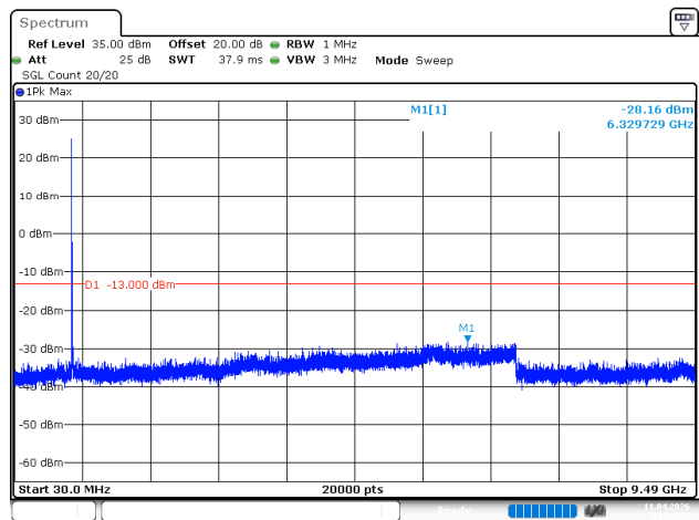
10MHz_Low_QPSK_1@0(30MHz~9.49GHz)
