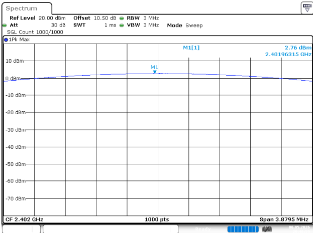
BDR_DH1_Low
