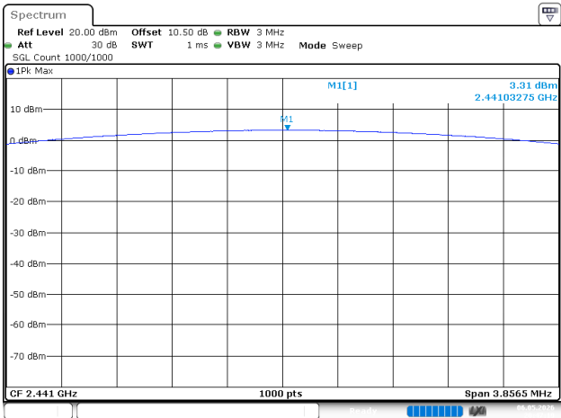
BDR_DH1_Middle
