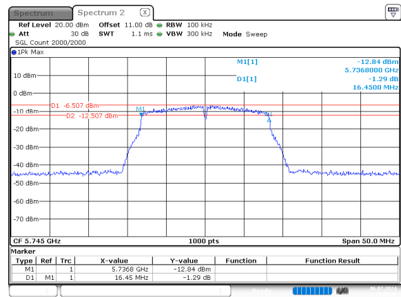
a_5745MHz_Chain 0
