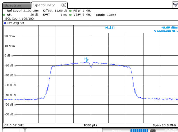
n40_5670MHz_Chain 0
