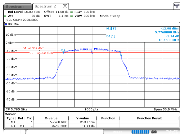
a_5785MHz_Chain 0
