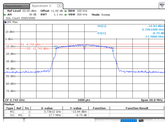
n20_5745MHz_Chain 0
