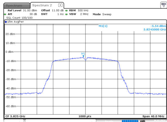
a_5825MHz_Chain 0
