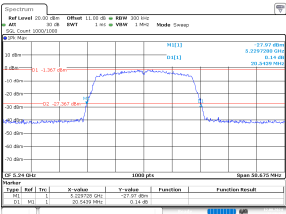
n20_5240MHz_Chain 0
