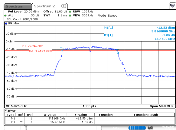
a_5825MHz_Chain 0
