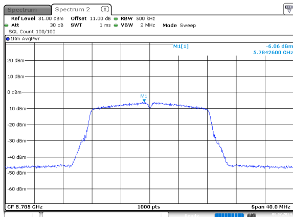
a_5785MHz_Chain 0
