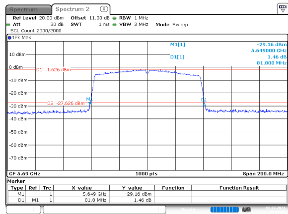
ac80_5690MHz_Chain 0
