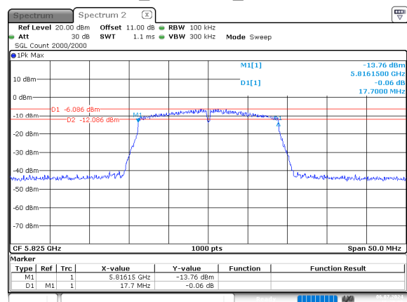
n20_5825MHz_Chain 0
