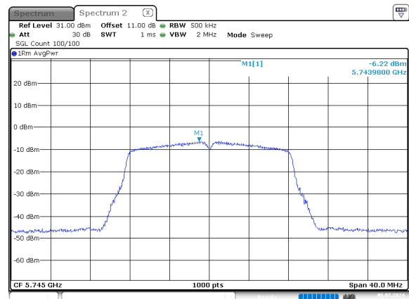
a_5745MHz_Chain 0
