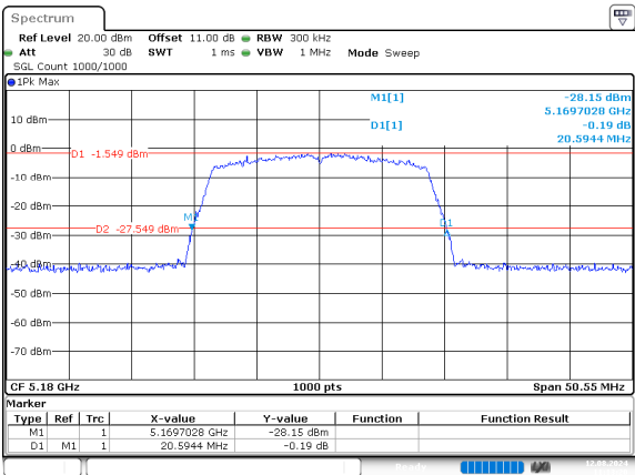
n20_5180MHz_Chain 0
