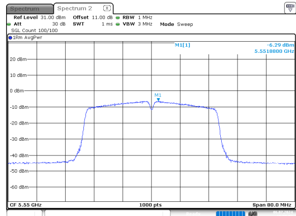
n40_5550MHz_Chain 0
