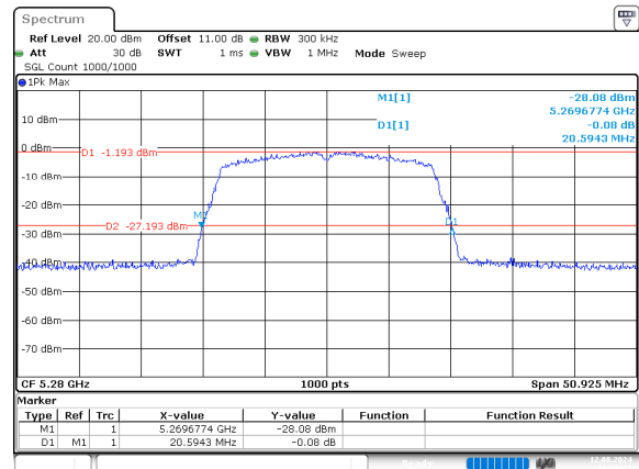
n20_5280MHz_Chain 0
