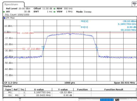
n20_5200MHz_Chain 0
