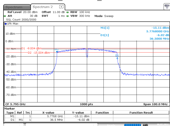
n40_5795MHz_Chain 0
