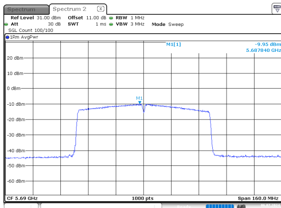
ac80_5690MHz_Chain 0
