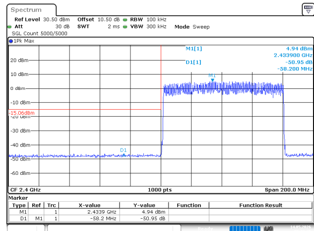
3EDR_DH1_Hopping_Lower
