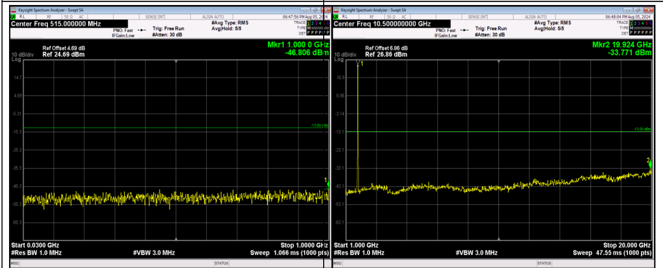
Band66-20MHz-16QAM-132072-1RB#0-Range1:3 0~1000MHz
