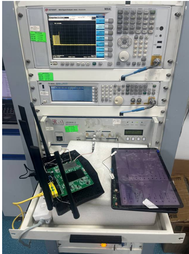
RF Conducted Test Photo
