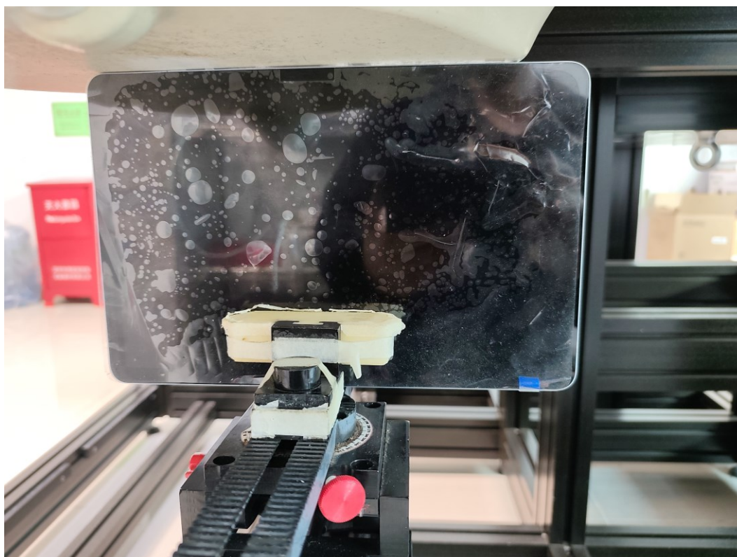
WLAN 2.4G Body Top Setup Photo (0 mm)
