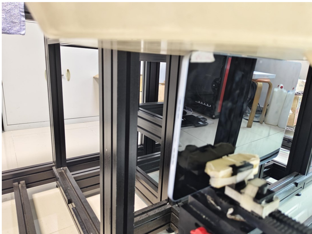
WLAN 5G Body Top Setup Photo (0 mm)
