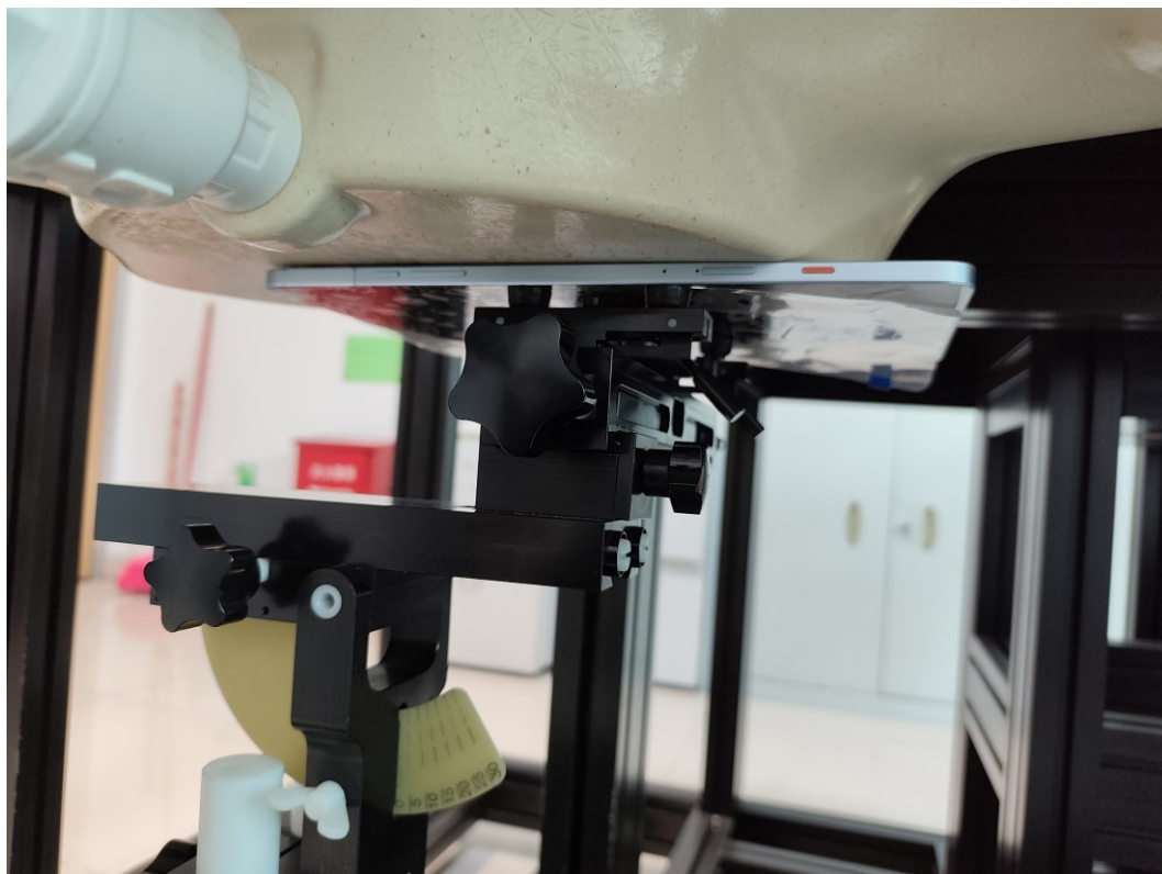
WLAN 2.4G Body Back Setup Photo (0 mm)
