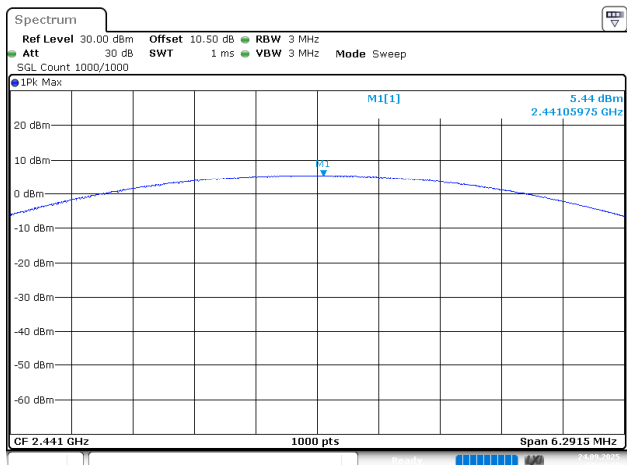
2EDR_DH1_Middle
