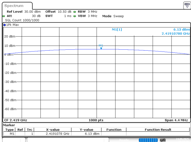
BDR_DH1_Additional (2419MHz)
