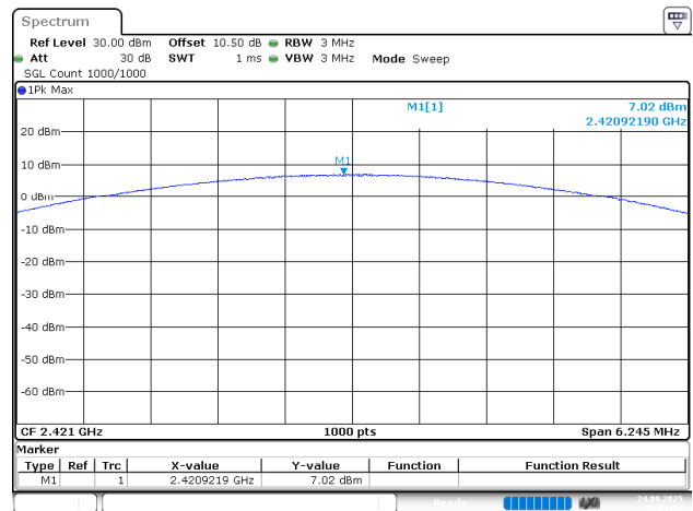
3EDR_DH1_Additional(2421MHz)
