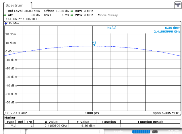
2EDR_DH1_Additional (2418MHz)
