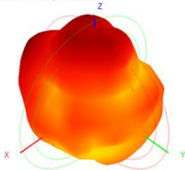
2450.0MHz H+V, Eff: 49.2%
