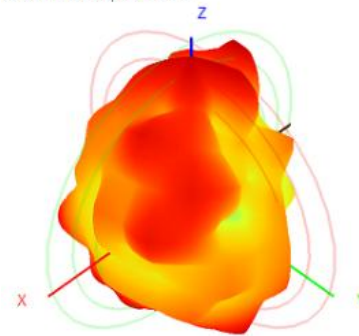
5850.0MHz H+V, Eff: 42.9%
