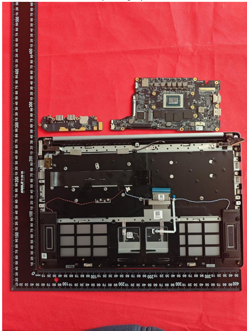
Internal photograph of EUT
