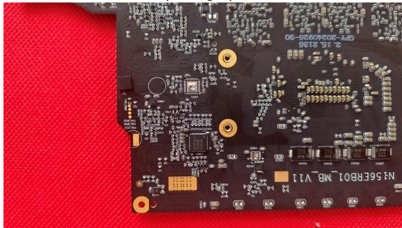
Internal photograph of EUT
