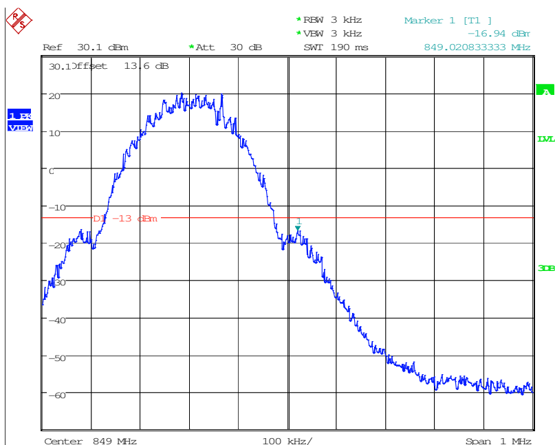
High Band Edge GSM 850 BAND CH 251
