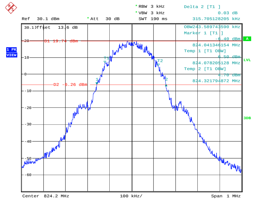
Occupied Bandwidth (99% and -26dBc) GSM 850 BAND CH 128
