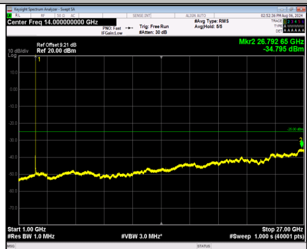
7-7-20MHz-20MHz-QPSK-QPSK-21152-21350-1RB#99-0R B#0-1000~27000MHz-PASS
