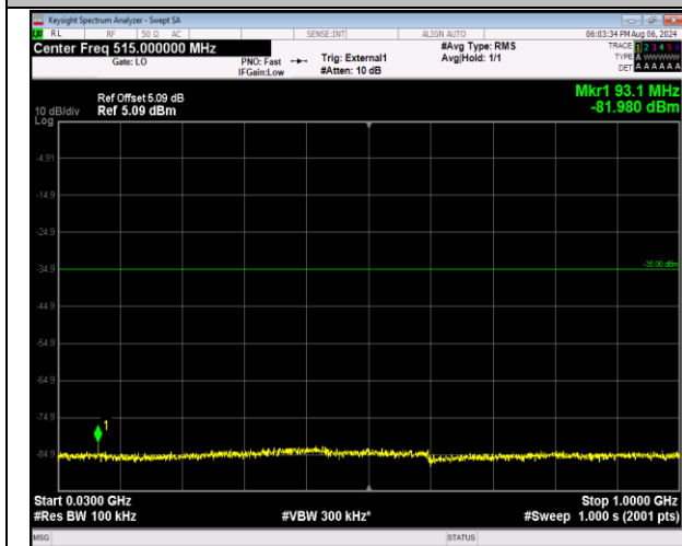
41-41-20MHz-5MHz-16QAM-16QAM-39750-39867-1RB# 99-ORB#0-30~1000MHz-PASS
