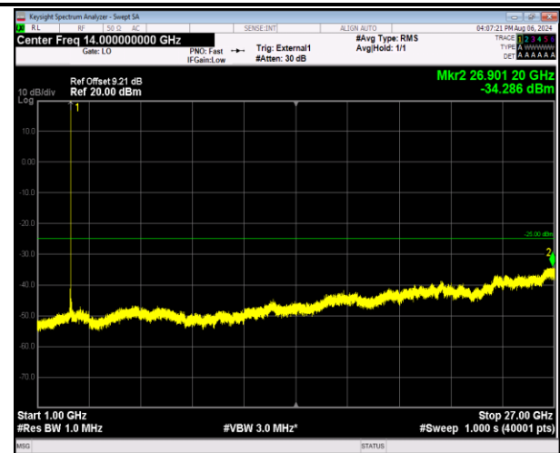
41-41-5MHz-20MHz-16QAM-16QAM-41373-41490-1RB#24 -ORB#0-1000~27000MHz-PASS
