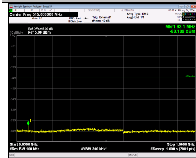
41-41-20MHz-5MHz-QPSK-QPSK-39750-39867-1RB#99 -ORB#0-30~1000MHz-PASS
