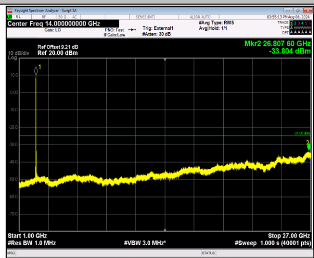
41-41-5MHz-20MHz-16QAM-16QAM-39683-39800-1RB#0-1RB#99-1000~27000MHz-PASS
