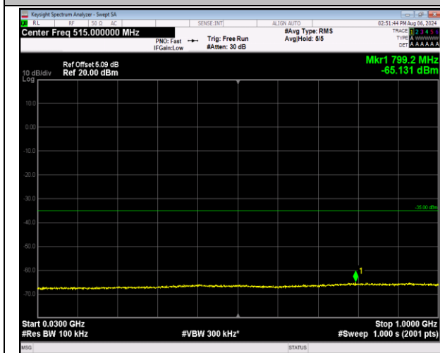
7-7-20MHz-20MHz-16QAM-16QAM-21152-21350-1RB#0 -ORB#0-30~1000MHz-PASS
