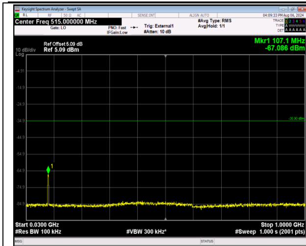
41-41-5MHz-20MHz-QPSK-QPSK-41373-41490-25RB#0 -100RB#0-30~1000MHz-PASS
