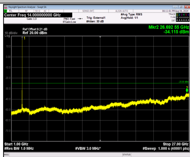
41-41-20MHz-5MHz-16QAM-16QAM-40595-40712-1RB#99-0RB#0-1000~27000MHz-PASS
