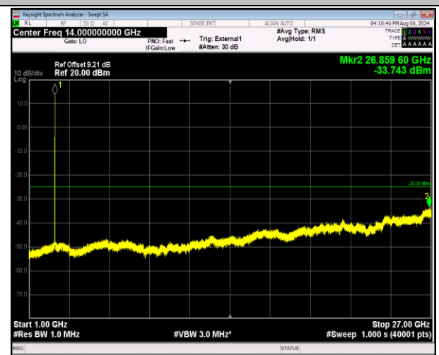
41-41-5MHz-20MHz-16QAM-16QAM-41373-41490-25RB#0 -100RB#0-1000~27000MHz-PASS
