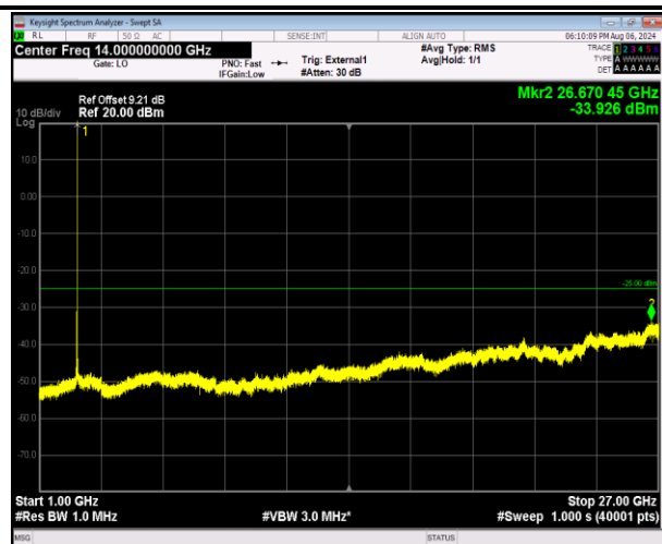
41-41-20MHz-5MHz-QPSK-QPSK-40595-40712-1RB#99-0 RB#0-1000~27000MHz-PASS
