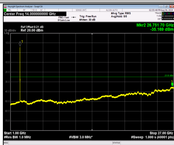
7-7-20MHz-20MHz-16QAM-16QAM-21152-21350-100RB#0 -100RB#0-1000~27000MHz-PASS
