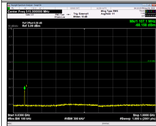
41-41-5MHz-20MHz-16QAM-16QAM-41373-41490-25RB#0 #0-100RB#0-30~1000MHz-PASS
