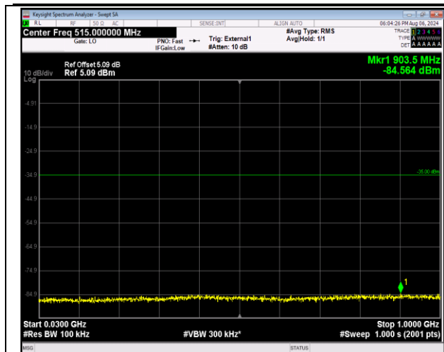
41-41-20MHz-5MHz-QPSK-QPSK-39750-39867-1RB#0-1RB#24-30~1000MHz-PASS
