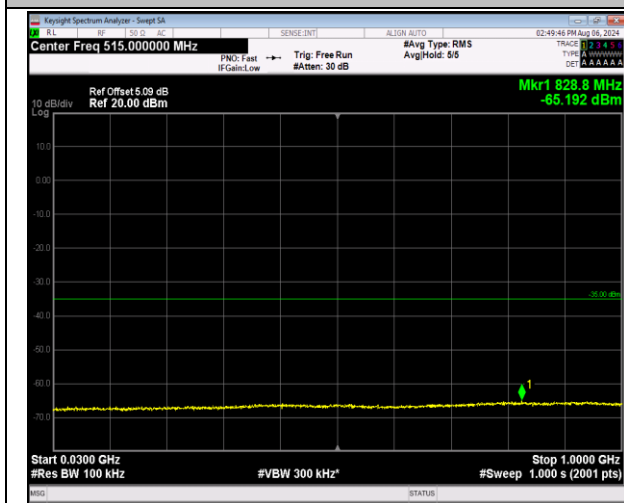
7-7-20MHz-20MHz-QPSK-QPSK-21001-21199-100RB#0 -100RB#0-30~1000MHz-PASS
