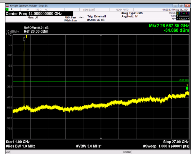
41-41-5MHz-20MHz-16QAM-16QAM-41373-41490-1RB#0-1RB#99-1000~27000MHz-PASS
