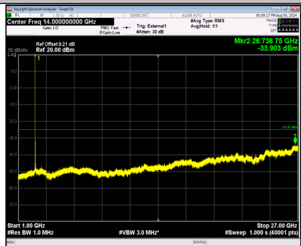
41-41-20MHz-5MHz-16QAM-16QAM-40595-40712-1RB#0-0RB#0-1000~27000MHz-PASS
