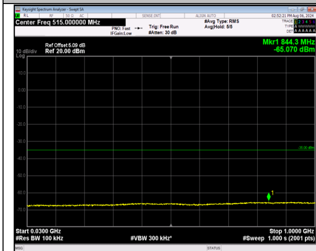
7-7-20MHz-20MHz-QPSK-QPSK-21152-21350-1RB#99-99 ORB#0-30~1000MHz-PASS
