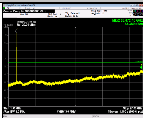
41-41-20MHz-5MHz-16QAM-16QAM-39750-39867-1RB#0-1RB#24-1000~27000MHz-PASS
