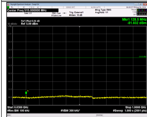
41-41-20MHz-5MHz-QPSK-QPSK-39750-39867-1RB#0-0 ORB#0-30~1000MHz-PASS
