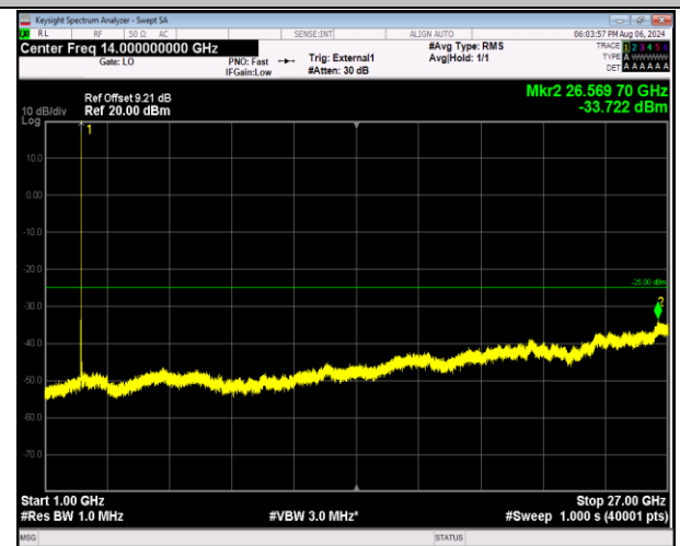
41-41-20MHz-5MHz-16QAM-16QAM-39750-39867-1RB#99 -ORB#0-1000~27000MHz-PASS
