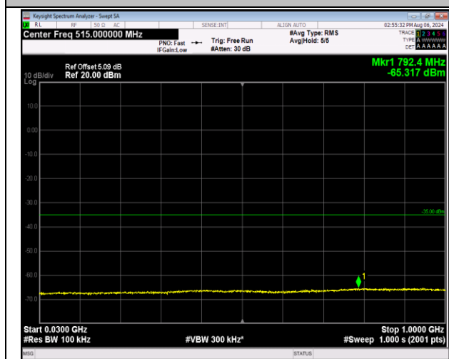
7-7-20MHz-20MHz-16QAM-16QAM-21152-21350-100RB #0-100RB#0-30~1000MHz-PASS
