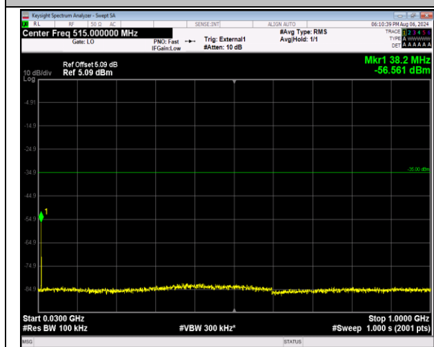
41-41-20MHz-5MHz-16QAM-16QAM-40595-40712-1RB#99-0RB#0-30~1000MHz-PASS
