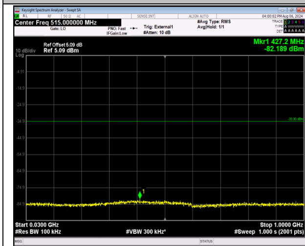
41-41-5MHz-20MHz-16QAM-16QAM-40528-40645-1RB# 24-0RB#0-30~1000MHz-PASS
