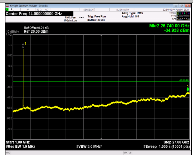
7-7-20MHz-20MHz-16QAM-16QAM-21001-21199-100RB#0 -100RB#0-1000~27000MHz-PASS
