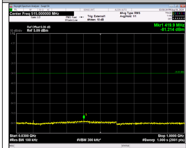
41-41-5MHz-20MHz-QPSK-QPSK-39683-39800-1RB#0-0 ORB#0-30~1000MHz-PASS
