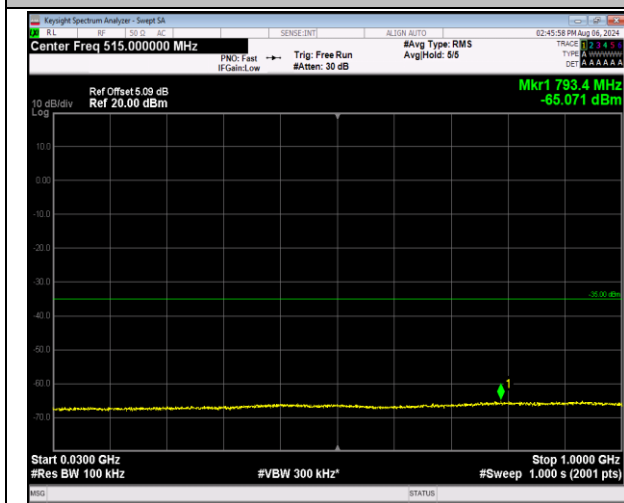
7-7-20MHz-20MHz-QPSK-QPSK-21001-21199-1RB#0-0 RB#0-30~1000MHz-PASS
