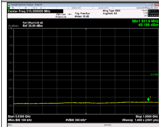
7-7-20MHz-20MHz-16QAM-16QAM-20850-21048-1RB#9 9-ORB#0-30~1000MHz-PASS
