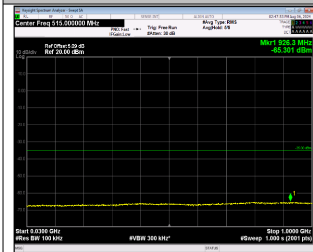
7-7-20MHz-20MHz-16QAM-16QAM-21001-21199-1RB#99-ORB#0-30~1000MHz-PASS
