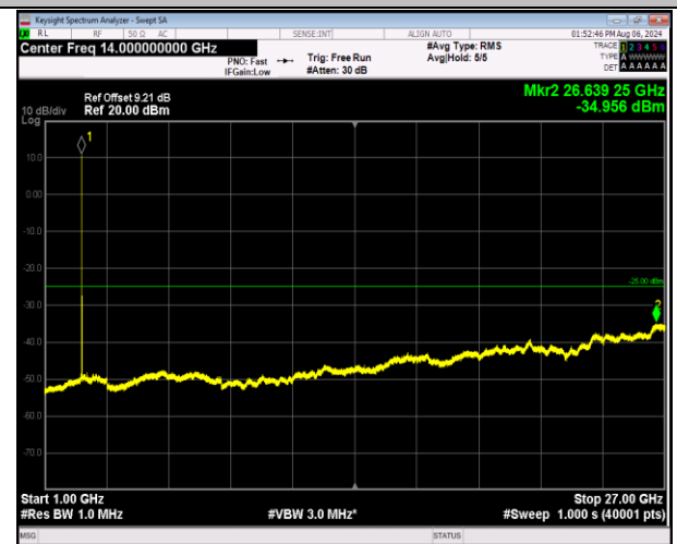
7-7-20MHz-10MHz-16QAM-16QAM-21251-21395-1RB#0-1 RB#49-1000~27000MHz-PASS
