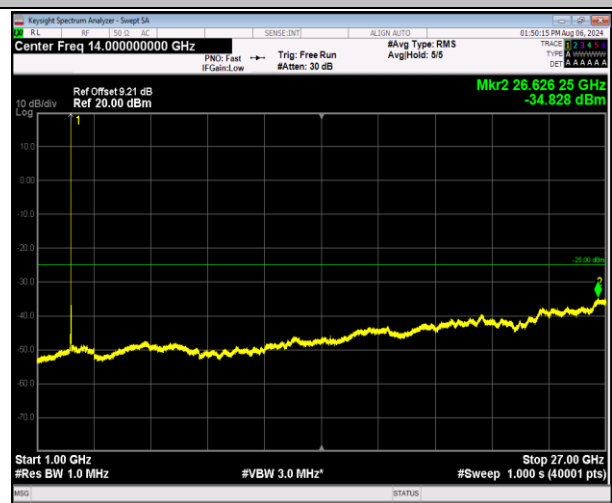
7-7-20MHz-10MHz-16QAM-16QAM-21251-21395-1RB#0-0 RB#0-1000~27000MHz-PASS
