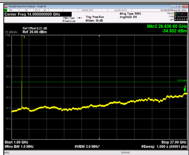
7-7-20MHz-20MHz-16QAM-16QAM-21001-21199-1RB#99-ORB#0-1000~27000MHz-PASS
