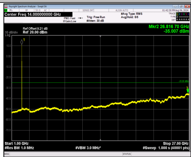
7-7-20MHz-10MHz-16QAM-16QAM-20850-20994-1RB#0-1 RB#49-1000~27000MHz-PASS
