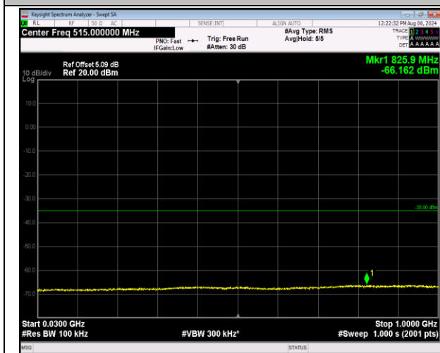
7-7-10MHz-20MHz-16QAM-16QAM-21006-21150-1RB#49-ORB#0-30~1000MHz-PASS
