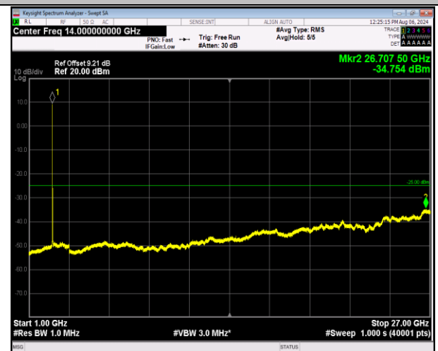
7-7-10MHz-20MHz-16QAM-16QAM-21006-21150-50RB#0-100RB#0-1000~27000MHz-PASS
