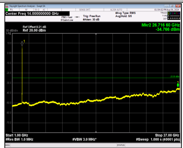
7-7-20MHz-10MHz-16QAM-16QAM-21251-21395-100RB#0-50RB#0-1000~27000MHz-PASS
