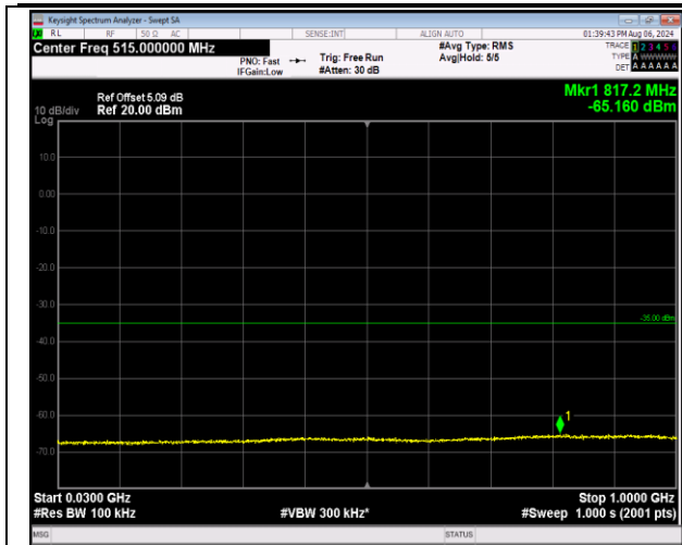
7-7-20MHz-10MHz-16QAM-16QAM-20850-20994-1RB#0 -ORB#0-30~1000MHz-PASS
