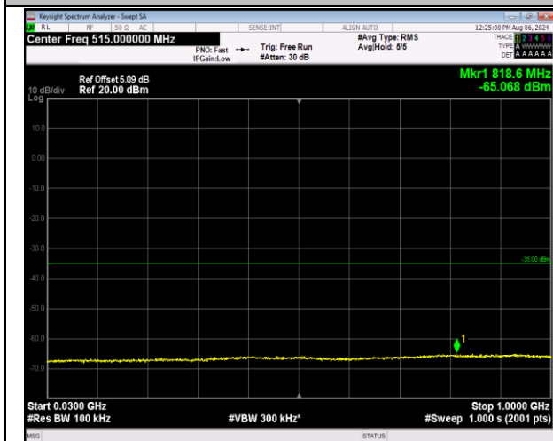
7-7-10MHz-20MHz-16QAM-16QAM-21006-21150-50RB#0-100RB#0-30~1000MHz-PASS
