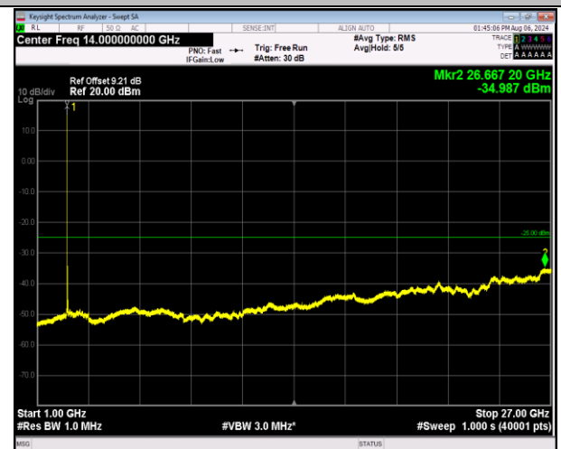
7-7-20MHz-10MHz-16QAM-16QAM-21051-21195-1RB#0-0 RB#0-1000~27000MHz-PASS
