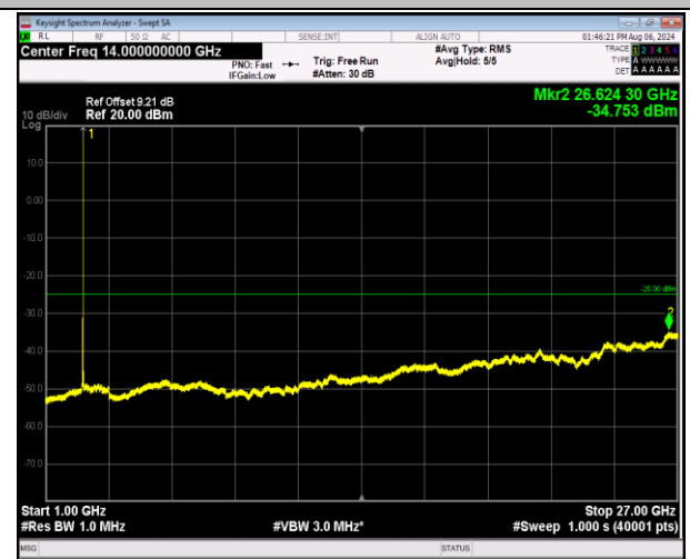
7-7-20MHz-10MHz-16QAM-16QAM-21051-21195-1RB#99-ORB#0-1000~27000MHz-PASS
