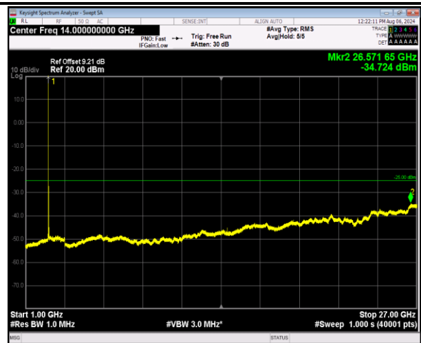
7-7-10MHz-20MHz-QPSK-QPSK-21006-21150-1RB#49-ORB#0-1000~27000MHz-PASS
