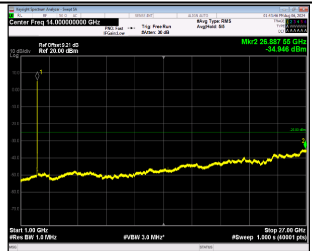
7-7-20MHz-10MHz-16QAM-16QAM-20850-20994-100RB#0 -50RB#0-1000~27000MHz-PASS
