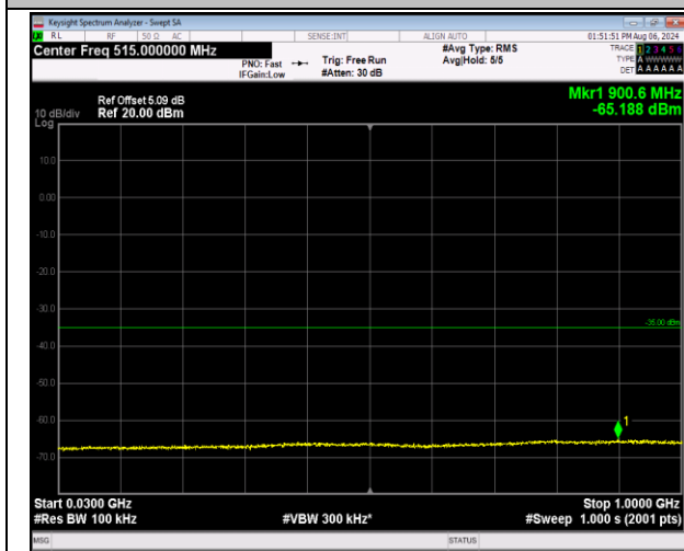
7-7-20MHz-10MHz-QPSK-QPSK-21251-21395-1RB#0-1 RB#49-30~1000MHz-PASS
