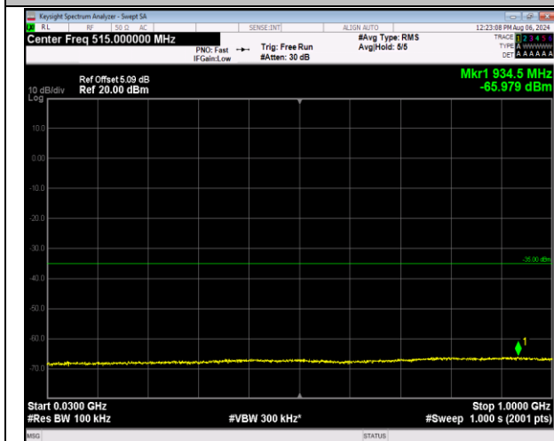
7-7-10MHz-20MHz-QPSK-QPSK-21006-21150-1RB#0-1RB#99-30~1000MHz-PASS
