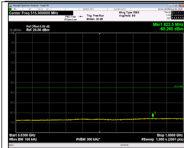
7-7-20MHz-20MHz-16QAM-16QAM-20850-21048-1RB#0 -ORB#0-30~1000MHz-PASS
