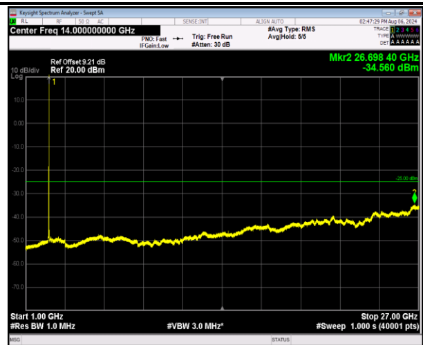
7-7-20MHz-20MHz-QPSK-QPSK-21001-21199-1RB#99-ORB#0-1000~27000MHz-PASS
