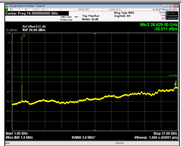
7-7-20MHz-10MHz-QPSK-QPSK-21251-21395-1RB#0-1RB #49-1000~27000MHz-PASS
