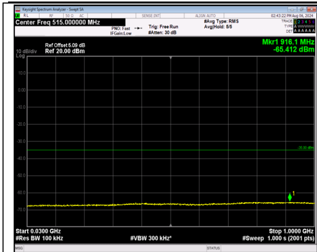
7-7-20MHz-20MHz-QPSK-QPSK-20850-21048-1RB#0-1 RB#99-30~1000MHz-PASS
