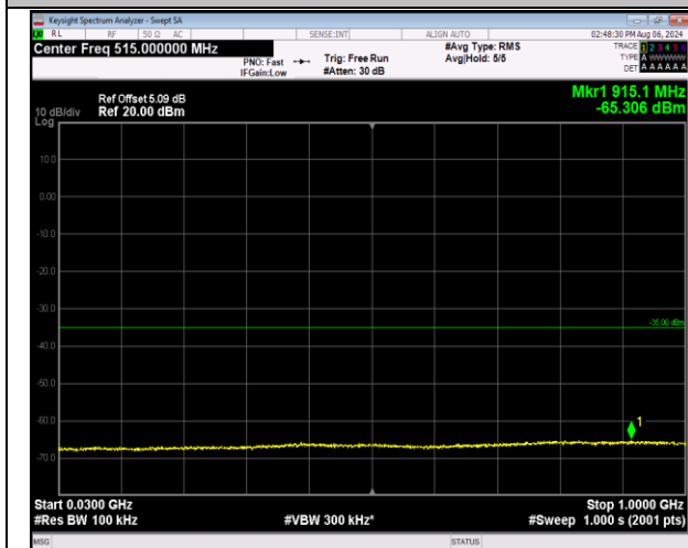
7-7-20MHz-20MHz-QPSK-QPSK-21001-21199-1RB#0-1RB#99-30~1000MHz-PASS
