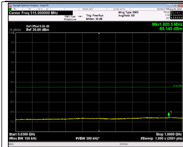
7-7-20MHz-20MHz-16QAM-16QAM-20850-21048-100RB #0-100RB#0-30~1000MHz-PASS
