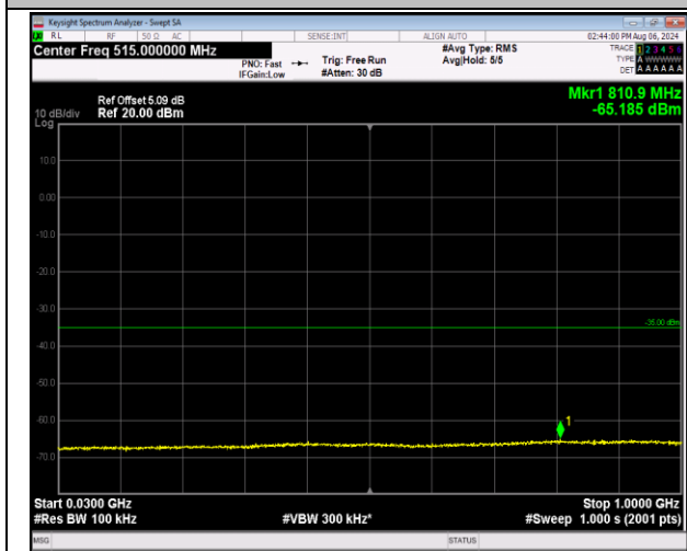
7-7-20MHz-20MHz-16QAM-16QAM-20850-21048-1RB#0-1RB#99-30~1000MHz-PASS
