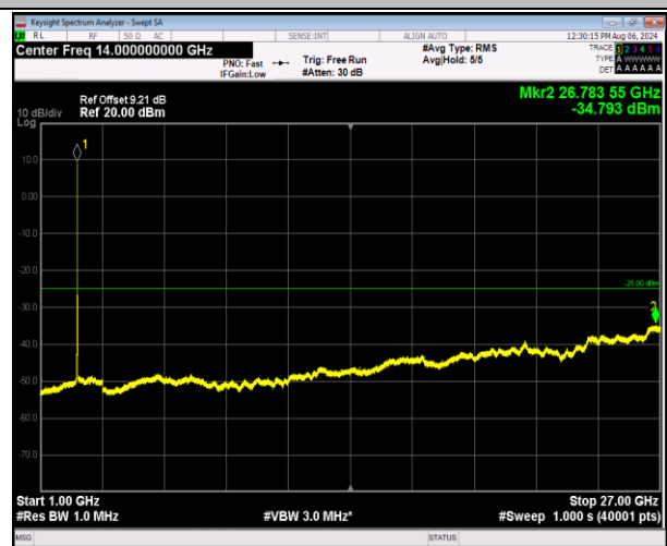
7-7-10MHz-20MHz-16QAM-16QAM-21206-21350-50RB#0-100RB#0-1000~27000MHz-PASS
