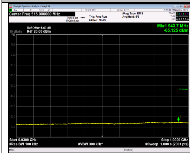
7-7-10MHz-20MHz-16QAM-16QAM-21206-21350-1RB#0-0 -ORB#0-30~1000MHz-PASS
