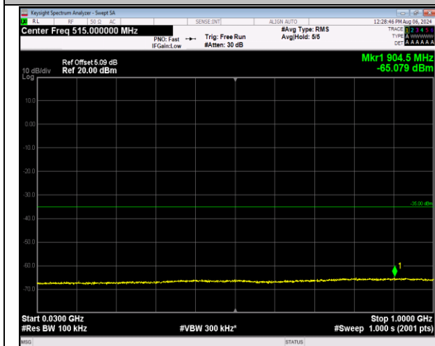
7-7-10MHz-20MHz-16QAM-16QAM-21206-21350-1RB#0 -1RB#99-30~1000MHz-PASS
