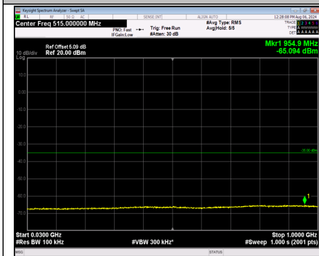
7-7-10MHz-20MHz-QPSK-QPSK-21206-21350-1RB#0-1 RB#99-30~1000MHz-PASS
