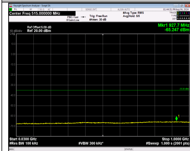
7-7-20MHz-10MHz-16QAM-16QAM-21051-21195-1RB#0 -0RB#0-30~1000MHz-PASS
