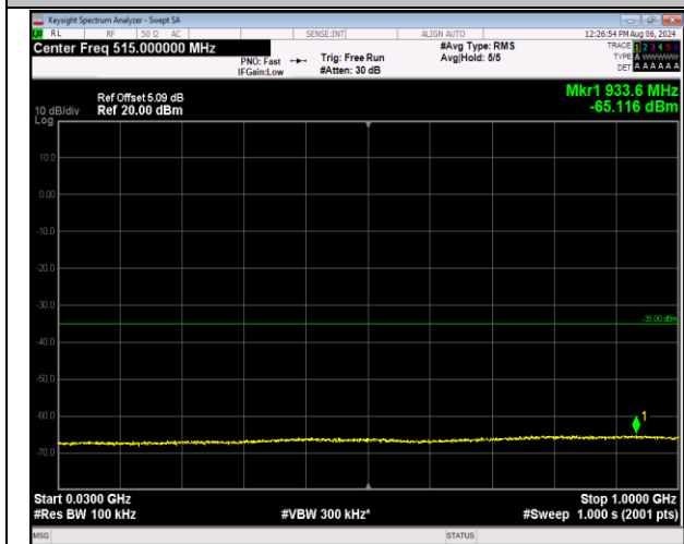
7-7-10MHz-20MHz-QPSK-QPSK-21206-21350-1RB#49-0 ORB#0-30~1000MHz-PASS
