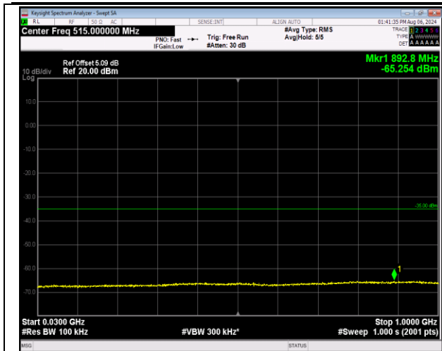
7-7-20MHz-10MHz-QPSK-QPSK-20850-20994-1RB#0-1 RB#49-30~1000MHz-PASS
