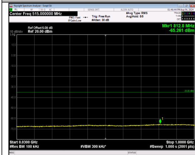
7-7-20MHz-10MHz-QPSK-QPSK-21051-21195-1RB#0-1RB#49-30~1000MHz-PASS
