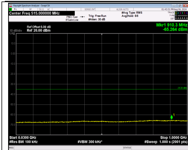
7-7-20MHz-10MHz-16QAM-16QAM-20850-20994-100RB #0-50RB#0-30~1000MHz-PASS
