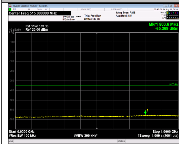
7-7-20MHz-20MHz-QPSK-QPSK-20850-21048-1RB#99-0 ORB#0-30~1000MHz-PASS
