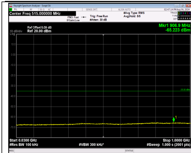
7-7-20MHz-20MHz-QPSK-QPSK-21001-21199-1RB#99-ORB#0-30~1000MHz-PASS
