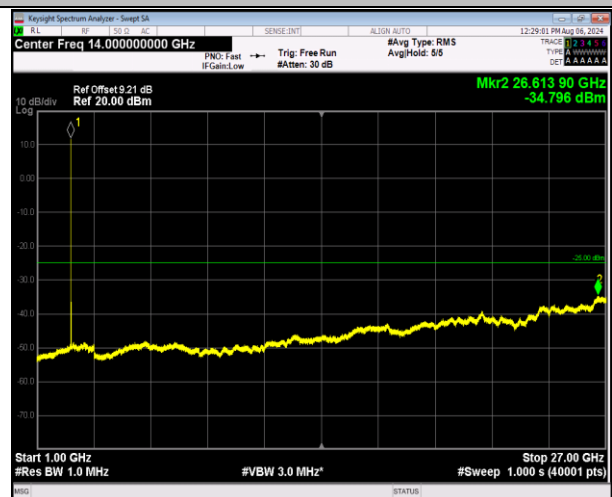
7-7-10MHz-20MHz-16QAM-16QAM-21206-21350-1RB#0-1 RB#99-1000~27000MHz-PASS
