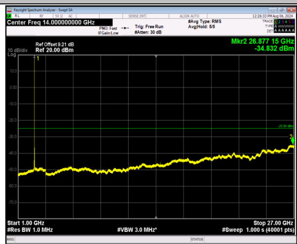
7-7-10MHz-20MHz-16QAM-16QAM-21206-21350-1RB#0-0 RB#0-1000~27000MHz-PASS
