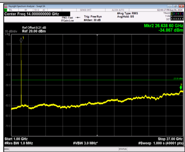
7-7-20MHz-20MHz-16QAM-16QAM-20850-21048-1RB#0-1RB#99-1000~27000MHz-PASS
