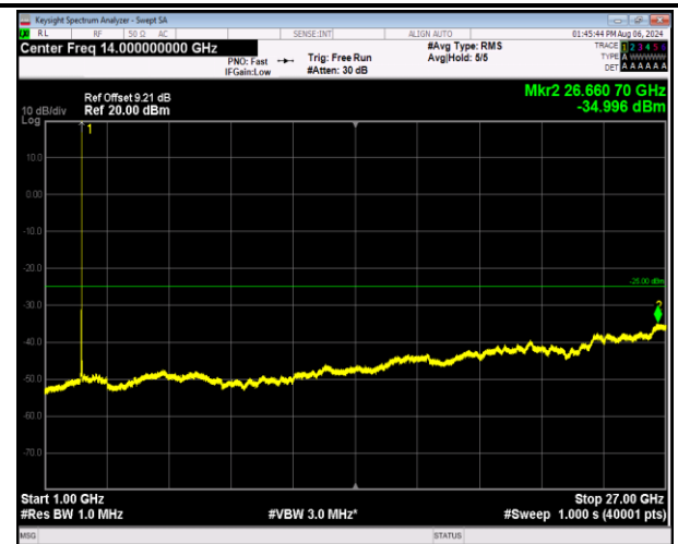
7-7-20MHz-10MHz-QPSK-QPSK-21051-21195-1RB#99-ORB#0-1000~27000MHz-PASS
