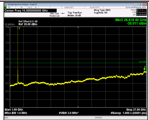
7-7-20MHz-20MHz-16QAM-16QAM-20850-21048-1RB#0-0 RB#0-1000~27000MHz-PASS
