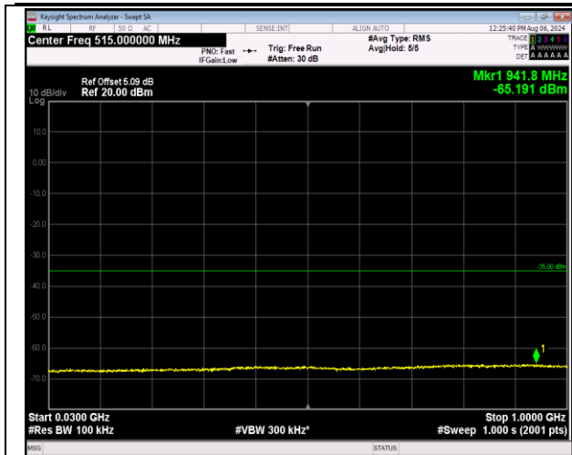
7-7-10MHz-20MHz-QPSK-QPSK-21206-21350-1RB#0-0 RB#0-30~1000MHz-PASS
