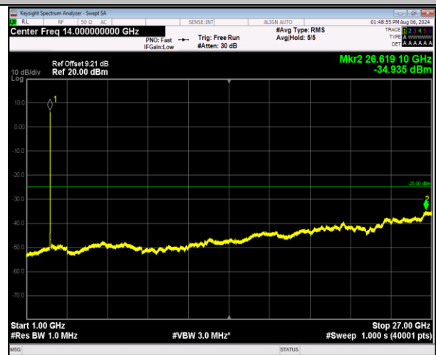
7-7-20MHz-10MHz-16QAM-16QAM-21051-21195-100RB#0 -50RB#0-1000~27000MHz-PASS
