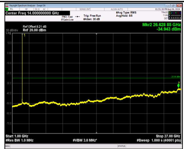
7-7-20MHz-10MHz-16QAM-16QAM-21251-21395-1RB#99- ORB#0-1000~27000MHz-PASS
