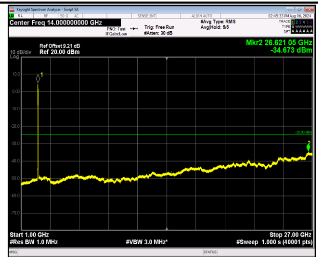
7-7-20MHz-20MHz-16QAM-16QAM-20850-21048-100RB#0 -100RB#0-1000~27000MHz-PASS
