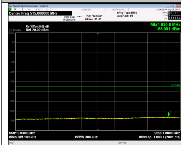
7-7-10MHz-20MHz-QPSK-QPSK-21006-21150-50RB#0-100RB#0-30~1000MHz-PASS
