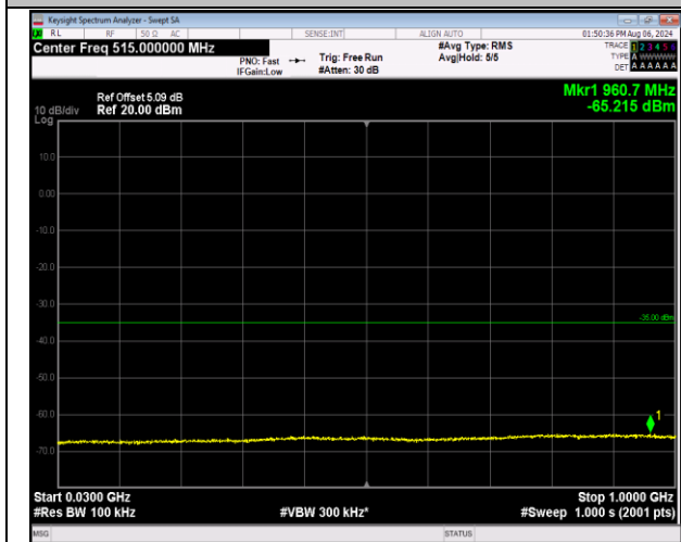
7-7-20MHz-10MHz-QPSK-QPSK-21251-21395-1RB#99-99 ORB#0-30~1000MHz-PASS
