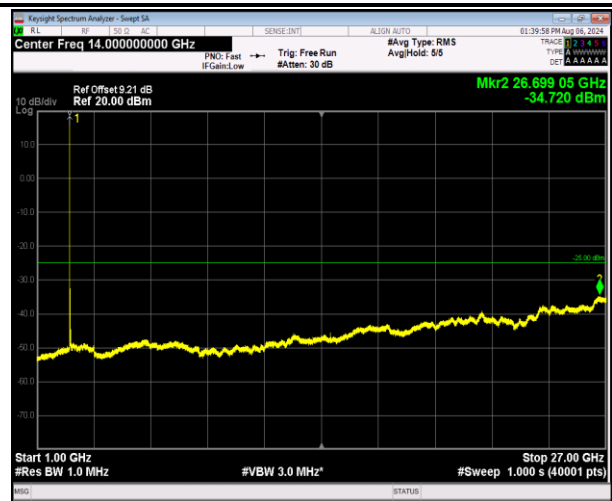
7-7-20MHz-10MHz-16QAM-16QAM-20850-20994-1RB#0-0 RB#0-1000~27000MHz-PASS
