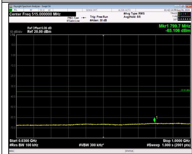
7-7-20MHz-10MHz-16QAM-16QAM-20850-20994-1RB#0 -1RB#49-30~1000MHz-PASS
