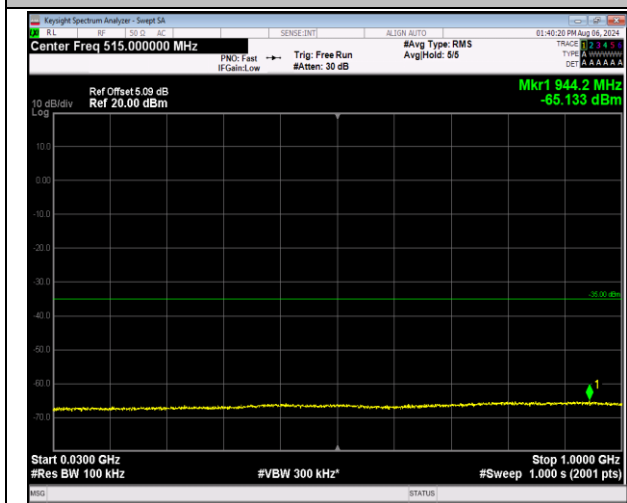
7-7-20MHz-10MHz-QPSK-QPSK-20850-20994-1RB#99-0 ORB#0-30~1000MHz-PASS
