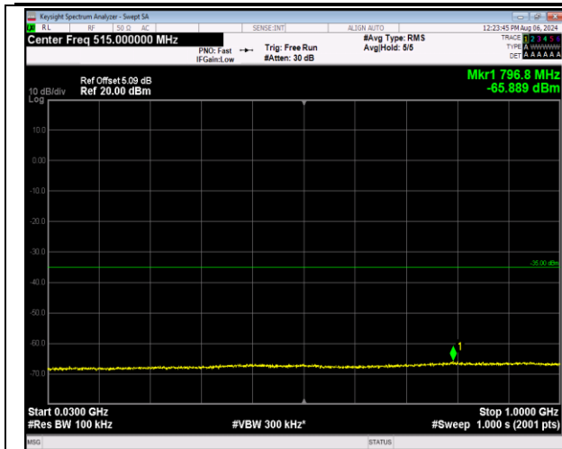
7-7-10MHz-20MHz-16QAM-16QAM-21006-21150-1RB#0 -1RB#99-30~1000MHz-PASS
