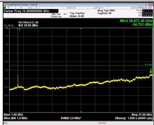
7-7-10MHz-20MHz-QPSK-QPSK-21206-21350-1RB#49-0R B#0-1000~27000MHz-PASS
