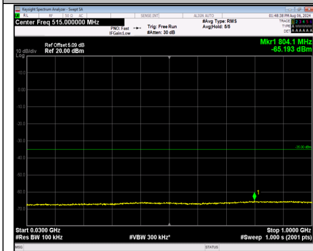
7-7-20MHz-10MHz-16QAM-16QAM-21051-21195-100RB #0-50RB#0-30~1000MHz-PASS
