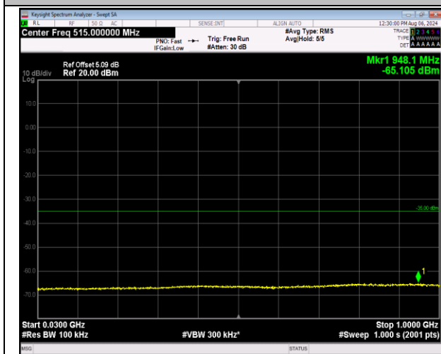
7-7-10MHz-20MHz-16QAM-16QAM-21206-21350-50RB#0-100RB#0-30~1000MHz-PASS
