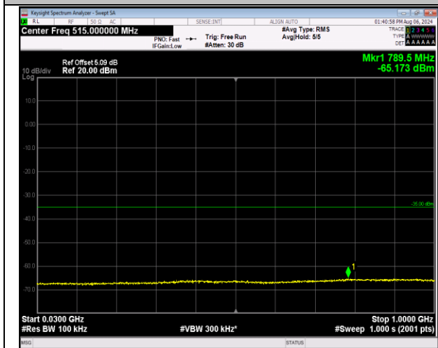
7-7-20MHz-10MHz-16QAM-16QAM-20850-20994-1RB#9 9-ORB#0-30~1000MHz-PASS
