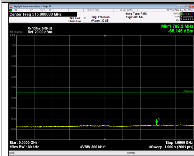
7-7-20MHz-10MHz-16QAM-16QAM-21251-21395-100RB#0-50RB#0-30~1000MHz-PASS
