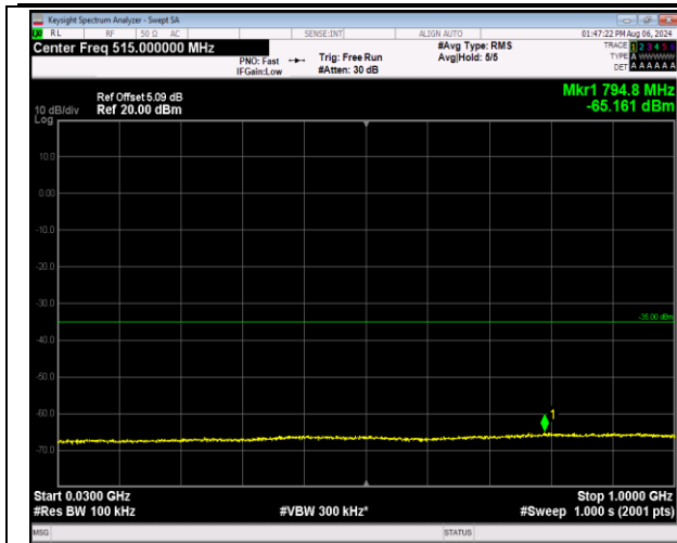
7-7-20MHz-10MHz-16QAM-16QAM-21051-21195-1RB#0 -1RB#49-30~1000MHz-PASS
