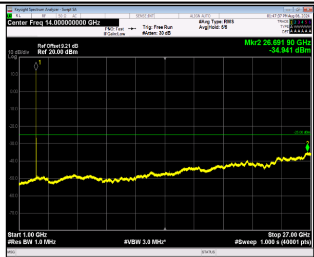
7-7-20MHz-10MHz-16QAM-16QAM-21051-21195-1RB#0-1 RB#49-1000~27000MHz-PASS
