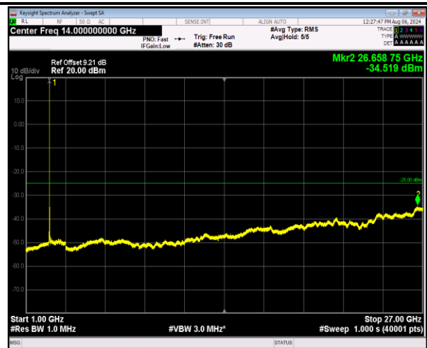
7-7-10MHz-20MHz-16QAM-16QAM-21206-21350-1RB#49- ORB#0-1000~27000MHz-PASS
