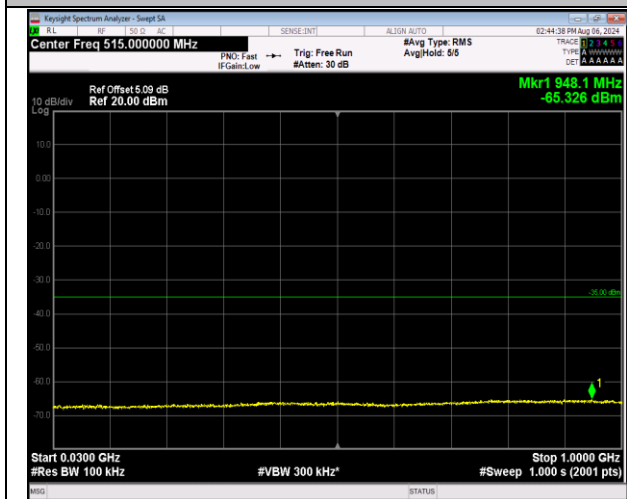
7-7-20MHz-20MHz-QPSK-QPSK-20850-21048-100RB#0-100RB#0-30~1000MHz-PASS
