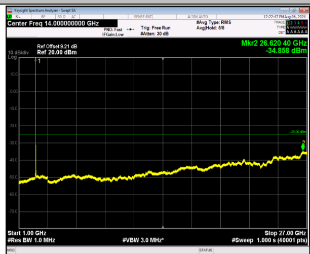
7-7-10MHz-20MHz-16QAM-16QAM-21006-21150-1RB#49-ORB#0-1000~27000MHz-PASS
