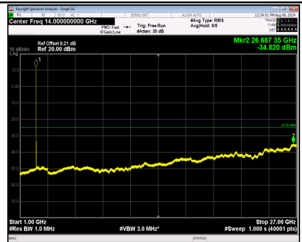
7-7-10MHz-20MHz-16QAM-16QAM-21006-21150-1RB#0-1 RB#99-1000~27000MHz-PASS
