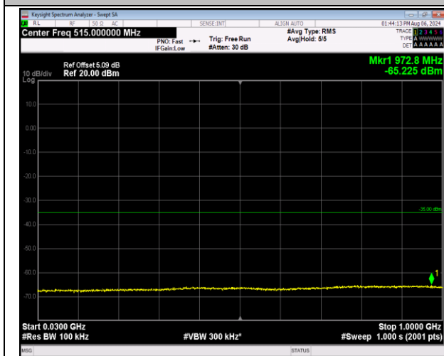
7-7-20MHz-10MHz-QPSK-QPSK-21051-21195-1RB#0-0 RB#0-30~1000MHz-PASS
