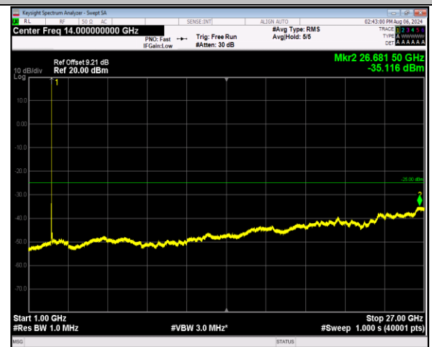
7-7-20MHz-20MHz-16QAM-16QAM-20850-21048-1RB#99-0 ORB#0-1000~27000MHz-PASS
