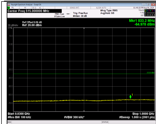
7-7-20MHz-10MHz-QPSK-QPSK-21251-21395-1RB#0-0 RB#0-30~1000MHz-PASS
