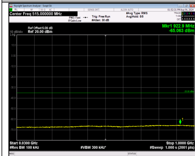
7-7-20MHz-10MHz-16QAM-16QAM-21251-21395-1RB#0 -1RB#49-30~1000MHz-PASS
