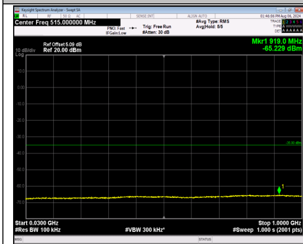
7-7-20MHz-10MHz-16QAM-16QAM-21051-21195-1RB#99-ORB#0-30~1000MHz-PASS
