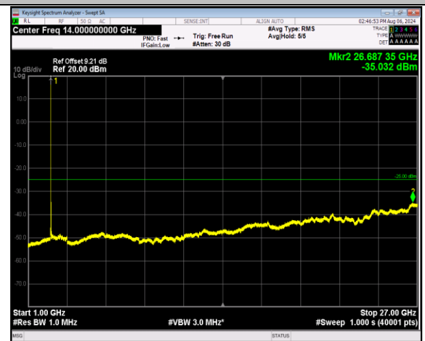
7-7-20MHz-20MHz-16QAM-16QAM-21001-21199-1RB#0-0 RB#0-1000~27000MHz-PASS
