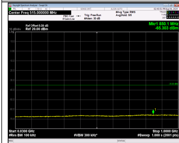
7-7-20MHz-20MHz-QPSK-QPSK-20850-21048-1RB#0-0RB#0-30~1000MHz-PASS
