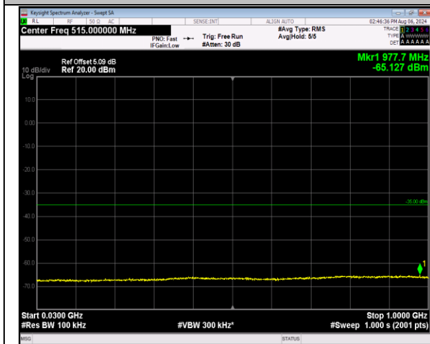
7-7-20MHz-20MHz-16QAM-16QAM-21001-21199-1RB#0 -0RB#0-30~1000MHz-PASS
