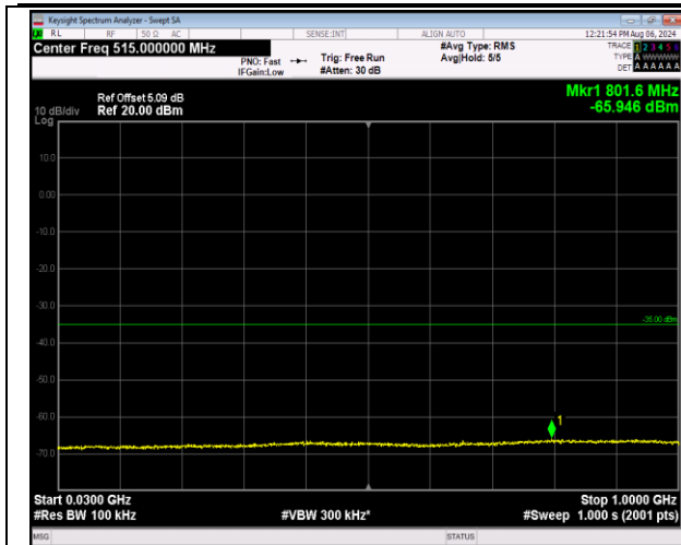
7-7-10MHz-20MHz-QPSK-QPSK-21006-21150-1RB#49-ORB#0-30~1000MHz-PASS
