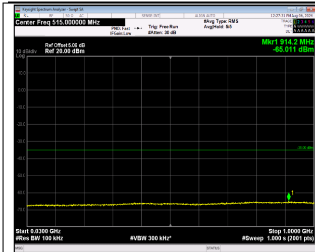
7-7-10MHz-20MHz-16QAM-16QAM-21206-21350-1RB#4 9-ORB#0-30~1000MHz-PASS
