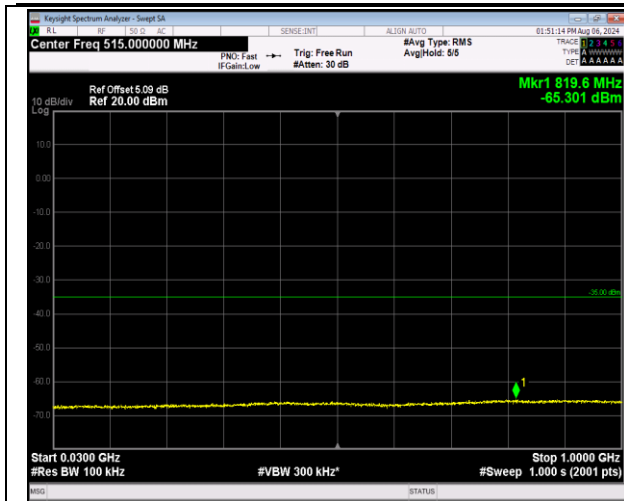
7-7-20MHz-10MHz-16QAM-16QAM-21251-21395-1RB#9 9-ORB#0-30~1000MHz-PASS
