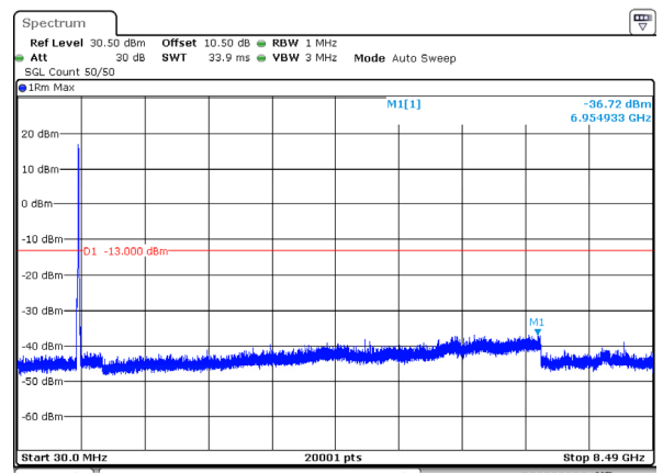
n5_20MHz_15kHz_839MHz_DFT-s-OFDM QPSK_RB100@0 -36.72dBm
