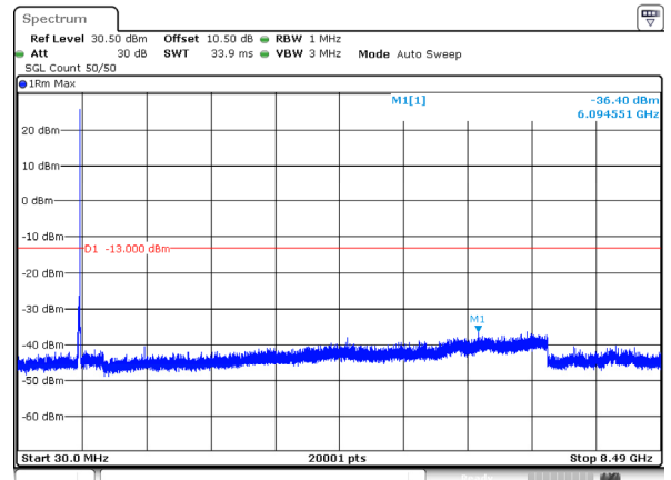
n5_20MHz_15kHz_836.5MHz_DFT-s-OFDM QPSK_RB1@105 -36.40dBm
