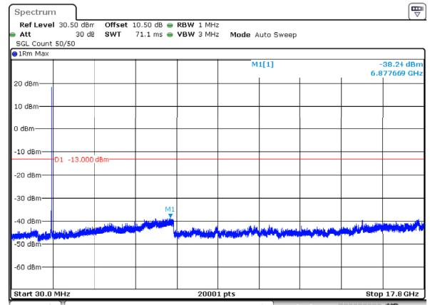
n66_25MHz_15kHz_1722.5MHz_DFT-s-OFDM QPSK_RB1@132 -38.24dBm
