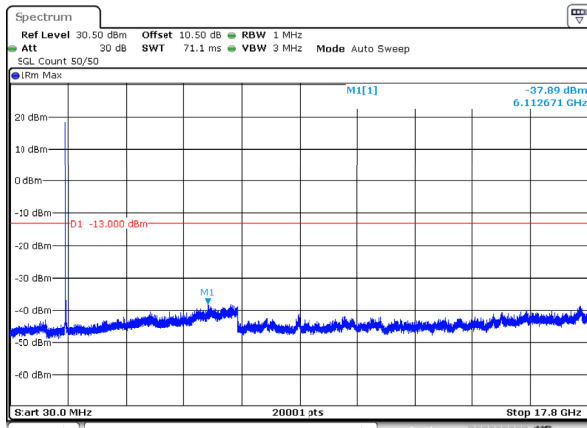
n66_25MHz_15kHz_1722.5MHz_DFT-s-OFDM QPSK_RB1@0 -37.89dBm
