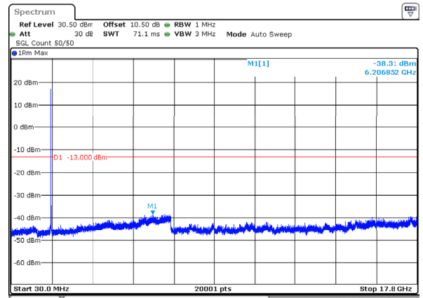
n66_25MHz_15kHz_1745MHz_DFT-s-OFDM QPSK_RB1@0 -38.31dBm
