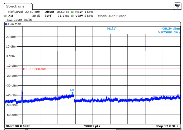
n66_25MHz_15kHz_1745MHz_DFT-s-OFDM QPSK_RB128@0 -38.29dBm
