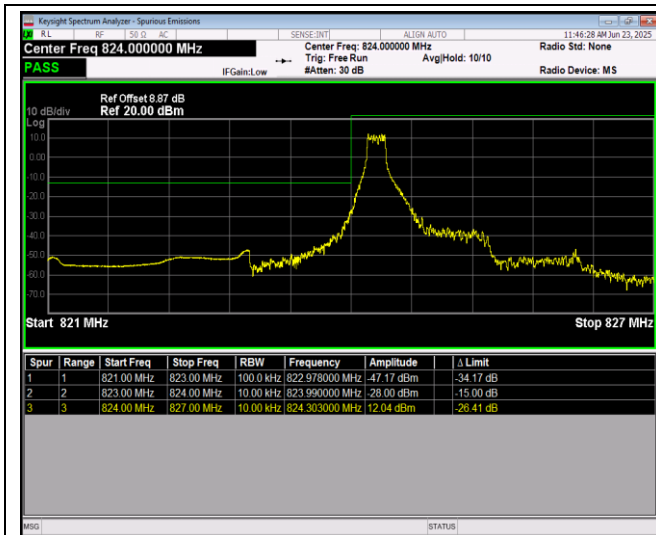
Band5-1.4MHz-64QAM-20407-6RB#0
