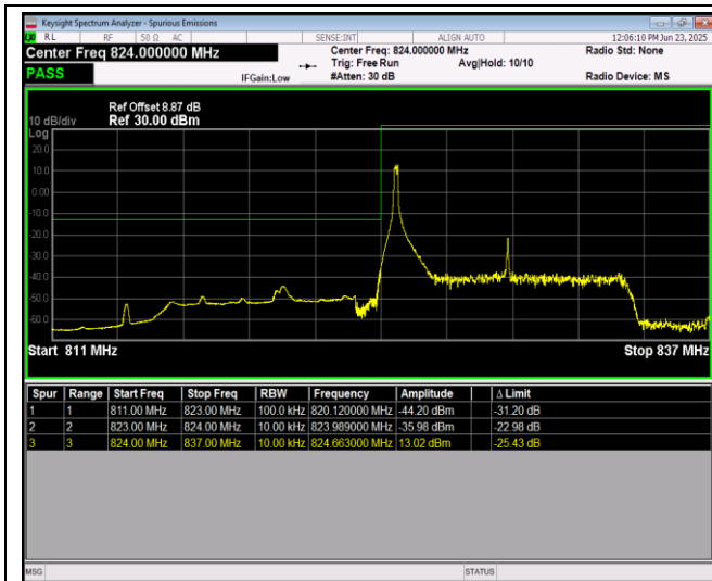
Band5-10MHz-QPSK-20450-50RB#0
