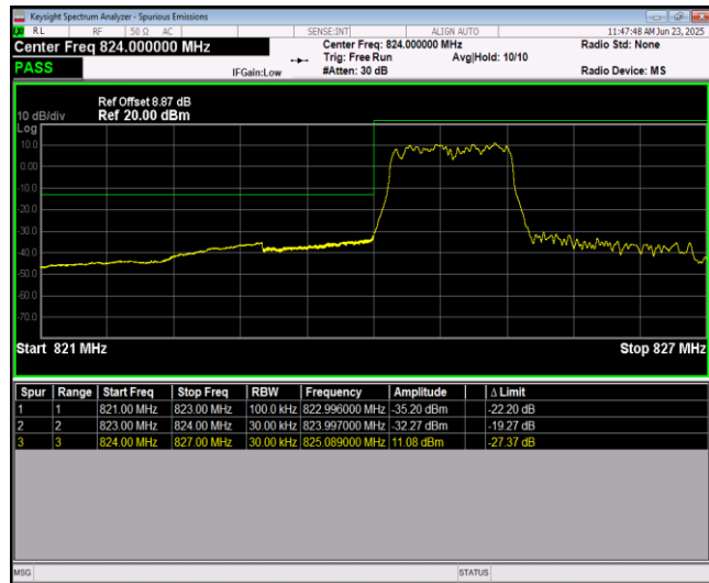
Band5-1.4MHz-QPSK-20643-1RB#5
