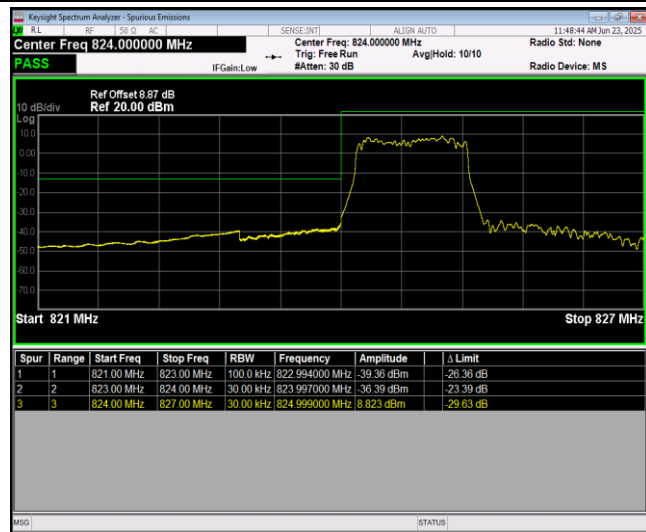
Band5-1.4MHz-64QAM-20643-1RB#5
