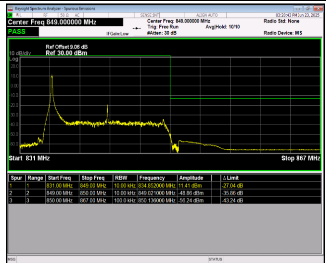
Band26-15MHz-16QAM-26965-75RB#0
