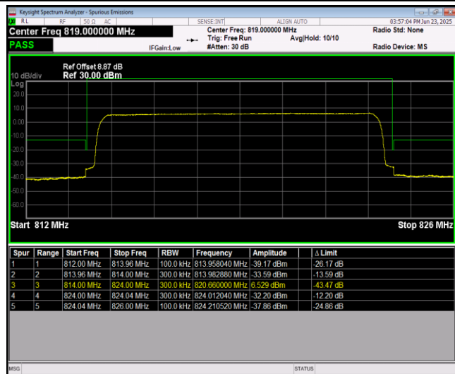
Band26-10MHz-64QAM-26740-1RB#49
