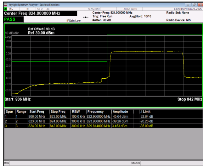
Band26-15MHz-64QAM-26965-1RB#74
