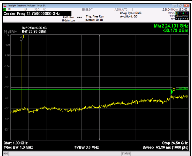
Band7-5MHz-64QAM-21425-1RB#0-Range2:1000~2 6500MHz
