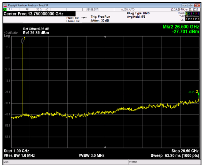
Band7-5MHz-64QAM-21100-1RB#0-Range2:1000~2 6500MHz
