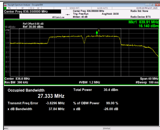
5-5-10MHz-10MHz-16QAM-16QAM-20501-20600-50RB#0-5 50RB#0-PASS
