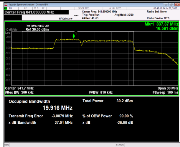
5-5-10MHz-5MHz-16QAM-16QAM-20450-20522-50RB#0-2 5RB#0-PASS
