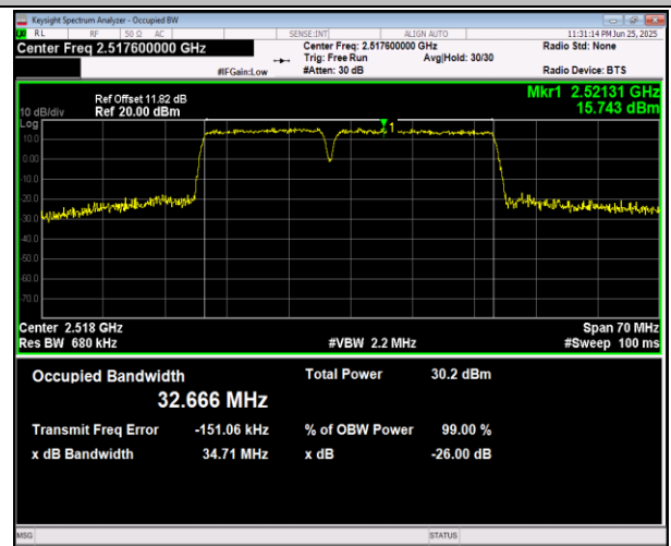
7-7-15MHz-20MHz-16QAM-16QAM-21003-21174-75RB#0- 100RB#0-PASS
