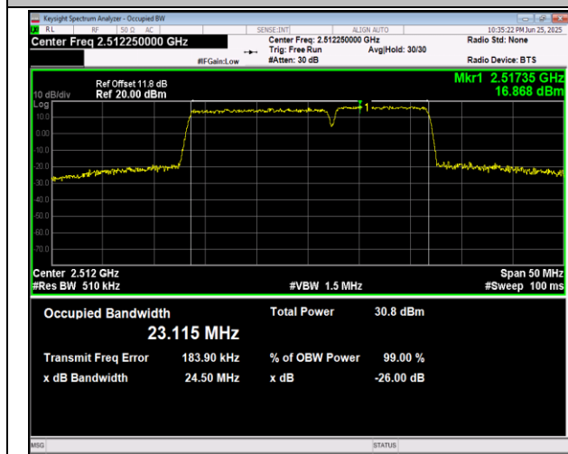
7-7-15MHz-10MHz-QPSK-QPSK-21051-21171-75RB#0-5 ORB#0-PASS
