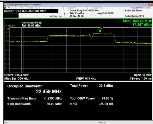
5-5-10MHz-5MHz-16QAM-16QAM-20550-20622-50RB#0-2 5RB#0-PASS
