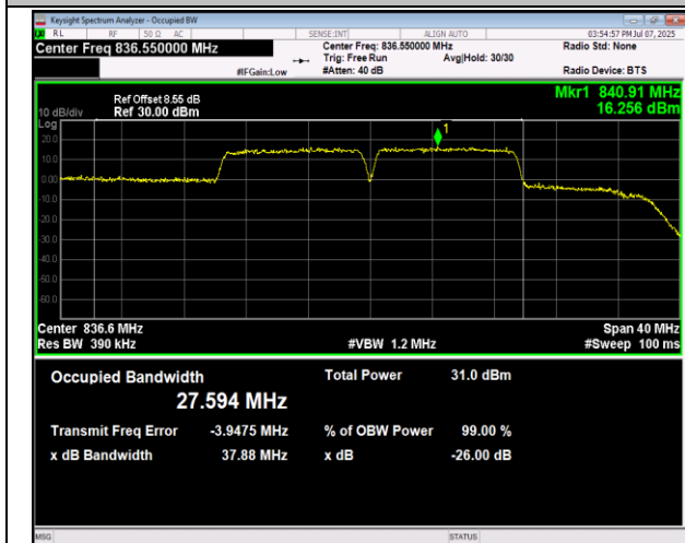
5-5-10MHz-10MHz-QPSK-QPSK-20501-20600-50RB#0-5 ORB#0-PASS
