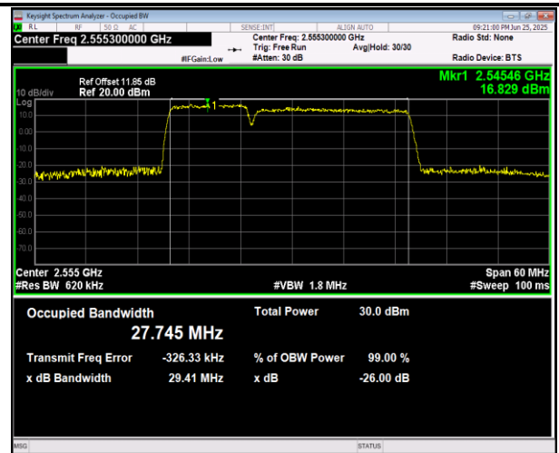
7-7-15MHz-10MHz-16QAM-16QAM-20825-20945-75RB#0-50RB#0-PASS
