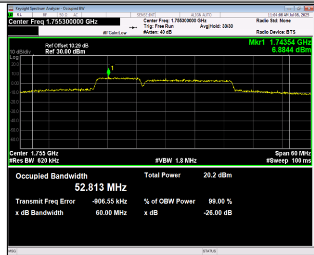
66-66-10MHz-20MHz-16QAM-16QAM-132428-132572-50R B#0-100RB#0-PASS
