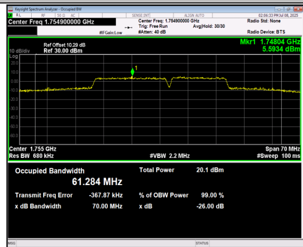
66-66-20MHz-15MHz-16QAM-16QAM-132423-132594-100 RB#0-75RB#0-PASS
