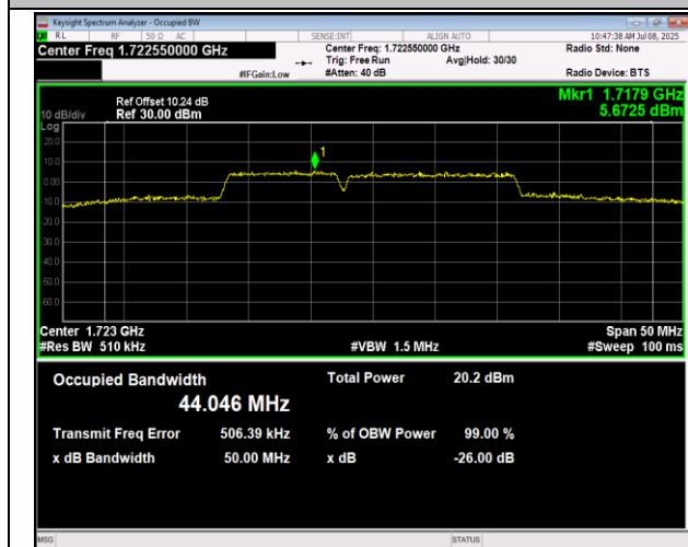
66-66-10MHz-15MHz-QPSK-QPSK-132351-132471-50R B#0-75RB#0-PASS
