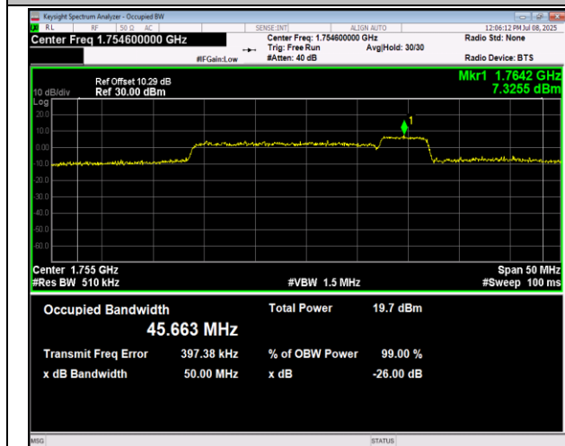
66-66-20MHz-5MHz-QPSK-QPSK-132522-132639-100R B#0-25RB#0-PASS
