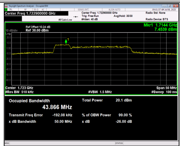
66-66-5MHz-20MHz-16QAM-16QAM-132330-132447-25R B#0-100RB#0-PASS
