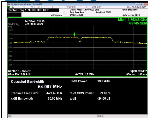
66-66-15MHz-20MHz-QPSK-QPSK-132050-132221-75R B#0-100RB#0-PASS
