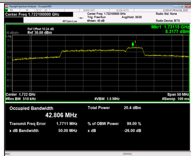
66-66-20MHz-5MHz-16QAM-16QAM-132397-132514-100R B#0-25RB#0-PASS
