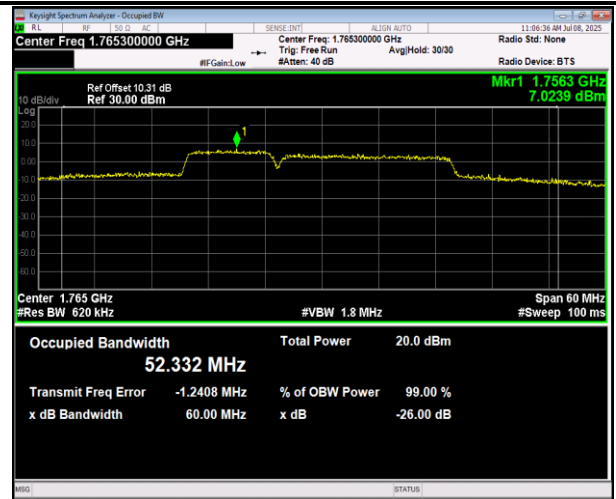
66-66-15MHz-10MHz-16QAM-16QAM-132047-132167-75R B#0-50RB#0-PASS
