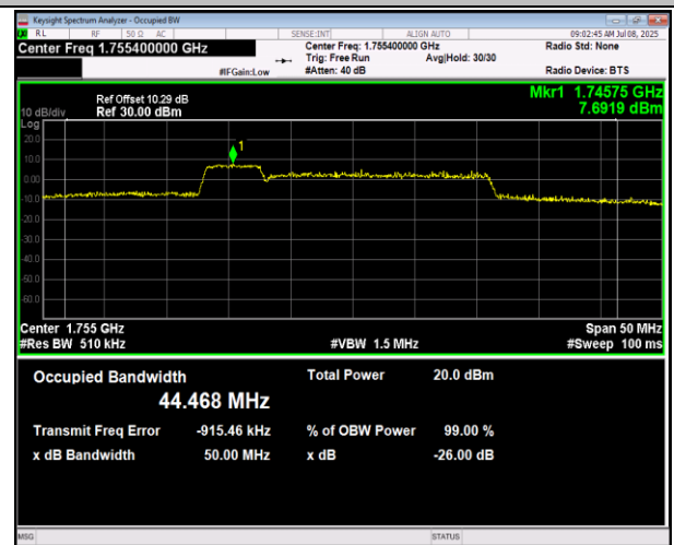
66-66-5MHz-20MHz-16QAM-16QAM-132455-132572-25R B#0-100RB#0-PASS
