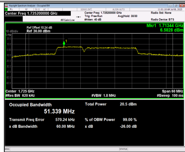
66-66-10MHz-20MHz-16QAM-16QAM-132328-132472-50R B#0-100RB#0-PASS
