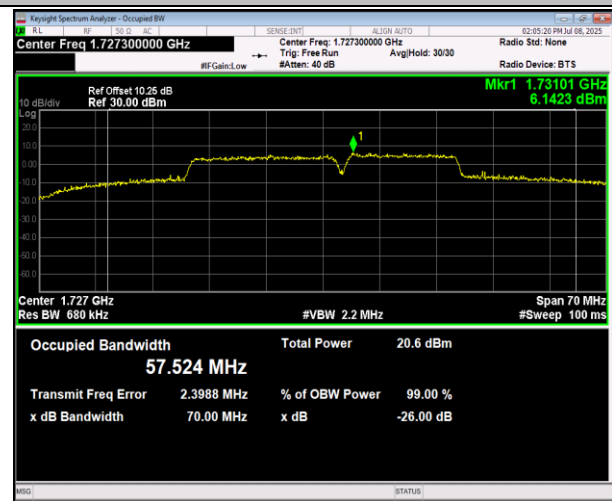
66-66-20MHz-15MHz-16QAM-16QAM-132348-132519-100 RB#0-75RB#0-PASS
