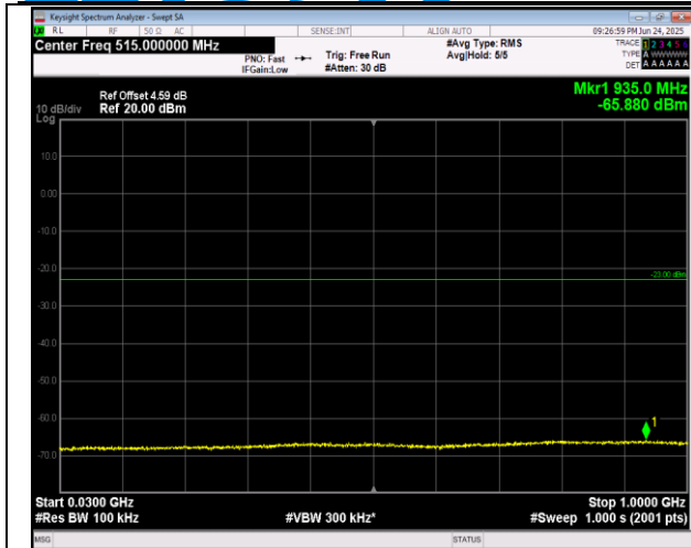
2-2-5MHz-20MHz-QPSK-QPSK-18983-19100-1RB#24-0 RB#0-30~1000MHz-PASS
