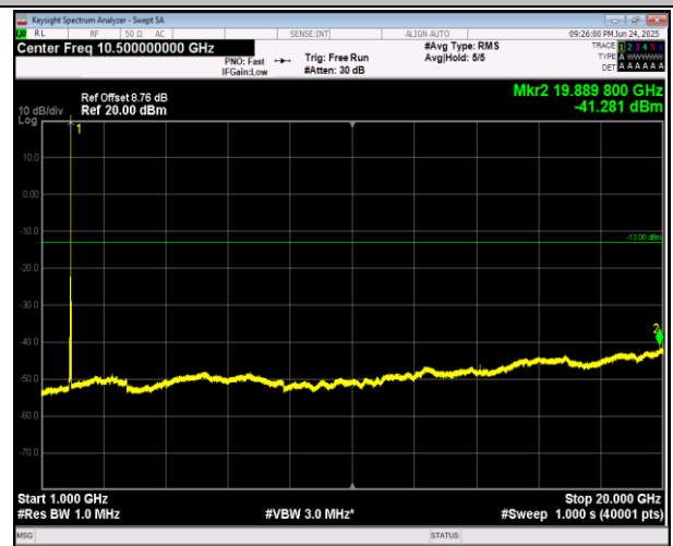
2-2-5MHz-20MHz-QPSK-QPSK-18983-19100-25RB#0-100 RB#0-1000~20000MHz-PASS
