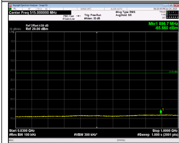
2-2-5MHz-20MHz-QPSK-QPSK-18983-19100-25RB#0-10 ORB#0-30~1000MHz-PASS
