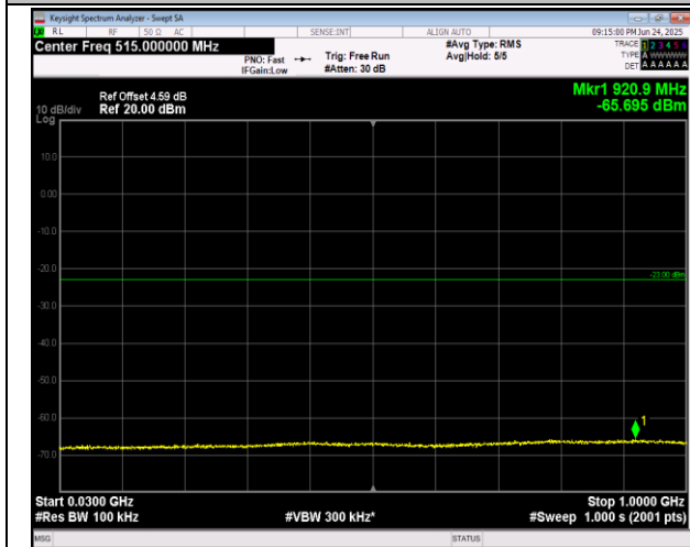
2-2-5MHz-20MHz-16QAM-16QAM-18633-18750-1RB#0- 1RB#99-30~1000MHz-PASS
