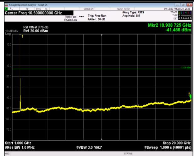
2-2-5MHz-20MHz-QPSK-QPSK-18633-18750-25RB#0-100 RB#0-1000~20000MHz-PASS
