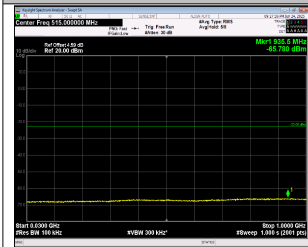
2-2-5MHz-20MHz-16QAM-16QAM-18983-19100-1RB#24-0RB#0-30~1000MHz-PASS
