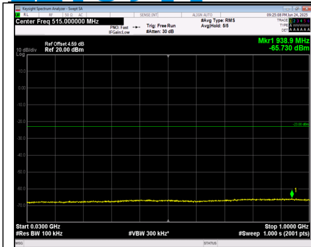
2-2-5MHz-20MHz-16QAM-16QAM-18983-19100-1RB#0-1RB#99-30~1000MHz-PASS
