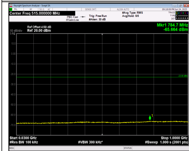
2-2-5MHz-20MHz-16QAM-16QAM-18633-18750-1RB#0- ORB#0-30~1000MHz-PASS
