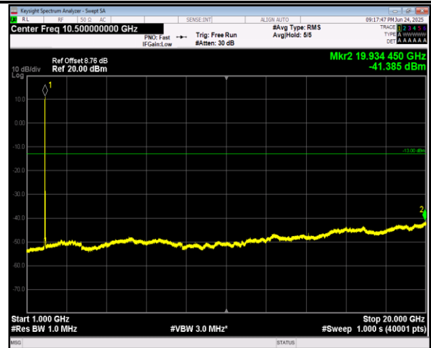
2-2-5MHz-20MHz-16QAM-16QAM-18633-18750-1RB#24-0 RB#0-1000~20000MHz-PASS
