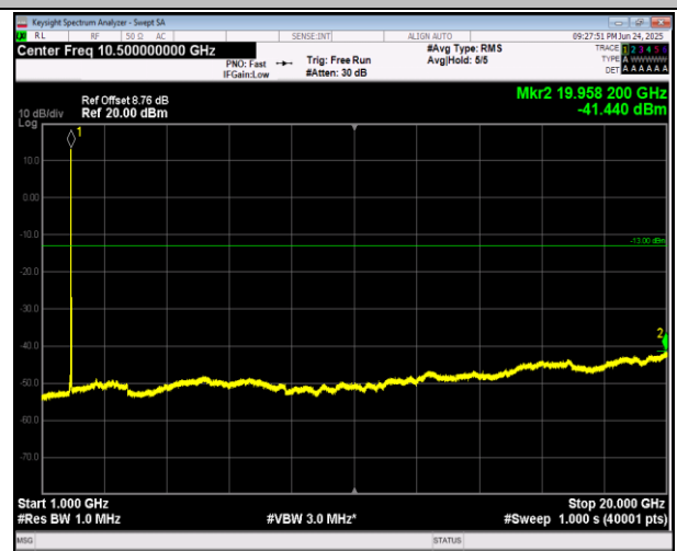
2-2-5MHz-20MHz-16QAM-16QAM-18983-19100-1RB#24-0RB#0-1000~20000MHz-PASS
