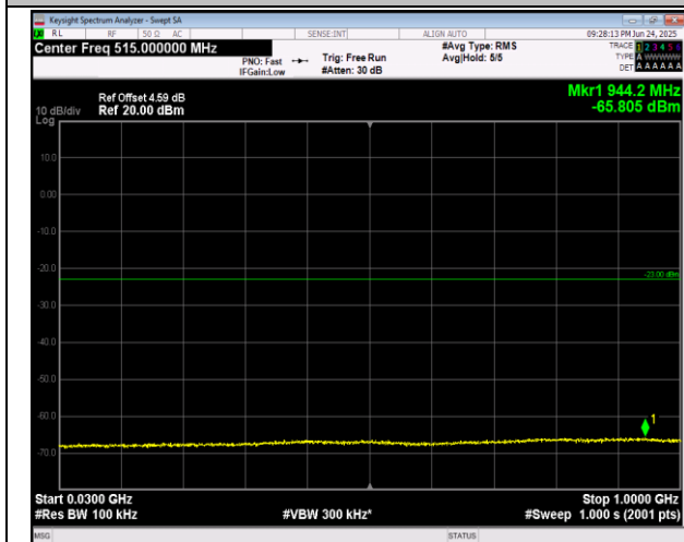
2-2-5MHz-20MHz-16QAM-16QAM-18983-19100-1RB#0- ORB#0-30~1000MHz-PASS
