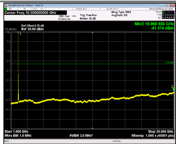
2-2-5MHz-20MHz-16QAM-16QAM-18633-18750-25RB#0-1 00RB#0-1000~20000MHz-PASS
