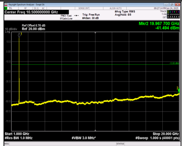
2-2-5MHz-20MHz-QPSK-QPSK-18983-19100-1RB#24-0RB #0-1000~20000MHz-PASS
