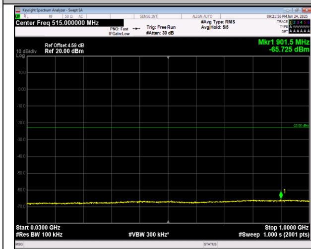
2-2-5MHz-20MHz-QPSK-QPSK-18808-18925-1RB#24-0 RB#0-30~1000MHz-PASS
