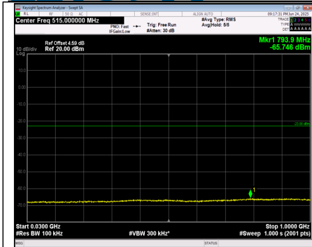
2-2-5MHz-20MHz-16QAM-16QAM-18633-18750-1RB#24 -0RB#0-30~1000MHz-PASS
