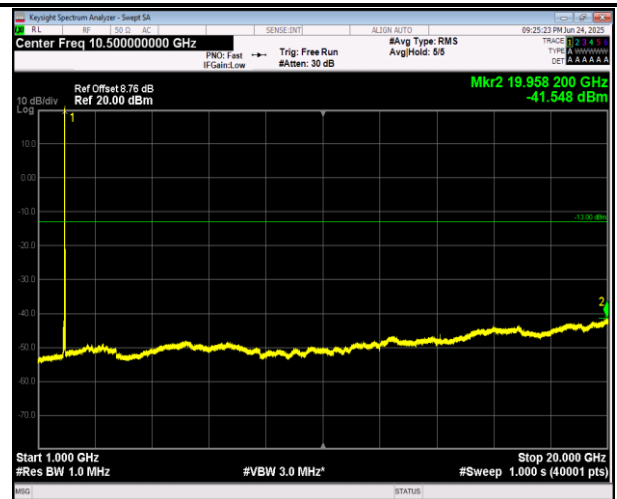
2-2-5MHz-20MHz-16QAM-16QAM-18983-19100-1RB#0-1RB#99-1000~20000MHz-PASS
