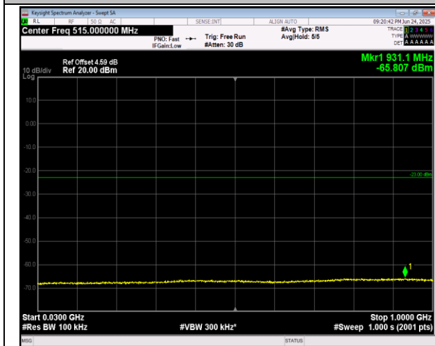
2-2-5MHz-20MHz-QPSK-QPSK-18808-18925-25RB#0-10 ORB#0-30~1000MHz-PASS
