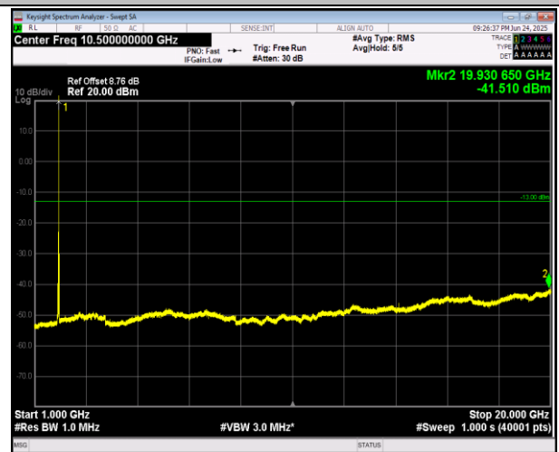
2-2-5MHz-20MHz-16QAM-16QAM-18983-19100-25RB#0-100RB#0-1000~20000MHz-PASS
