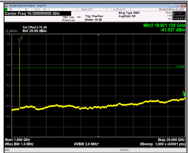
2-2-5MHz-20MHz-16QAM-16QAM-18633-18750-1RB#0-OR B#0-1000~20000MHz-PASS
