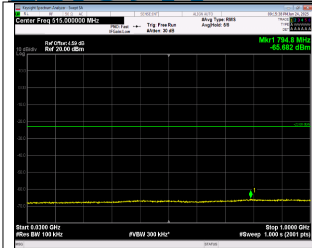
2-2-5MHz-20MHz-QPSK-QPSK-18633-18750-25RB#0-10 ORB#0-30~1000MHz-PASS
