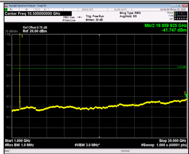
2-2-20MHz-20MHz-16QAM-16QAM-18700-18898-100RB# 0-100RB#0-1000~20000MHz-PASS
