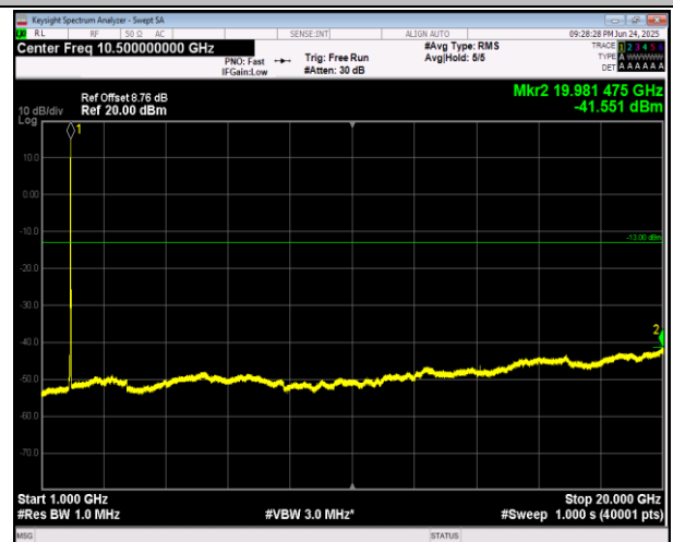
2-2-5MHz-20MHz-16QAM-16QAM-18983-19100-1RB#0-0RB B#0-1000~20000MHz-PASS
