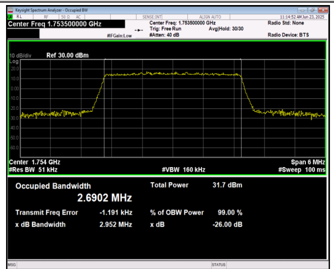
Band4-3MHz-16QAM-20175-15RB#0
