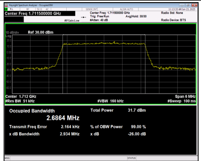
Band4-3MHz-QPSK-20385-15RB#0
