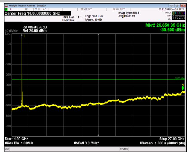
7-7-20MHz-20MHz-16QAM-16QAM-21001-21199-1RB#0-1 RB#99-1000~27000MHz-PASS
