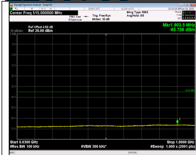
7-7-20MHz-10MHz-16QAM-16QAM-21051-21195-100RB #0-50RB#0-30~1000MHz-PASS
