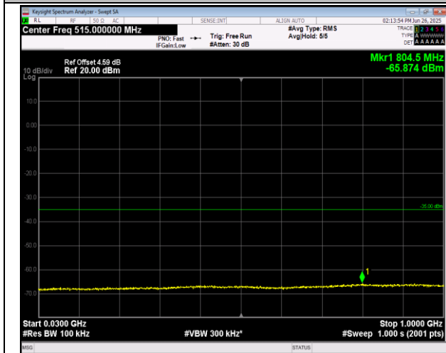
7-7-20MHz-20MHz-16QAM-16QAM-21001-21199-1RB#9 9-0RB#0-30~1000MHz-PASS
