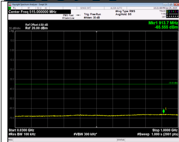
7-7-20MHz-10MHz-QPSK-QPSK-20850-20994-1RB#0-0 RB#0-30~1000MHz-PASS
