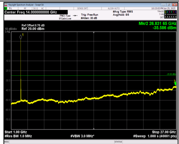
7-7-10MHz-20MHz-16QAM-16QAM-21006-21150-1RB#49- 0RB#0-1000~27000MHz-PASS
