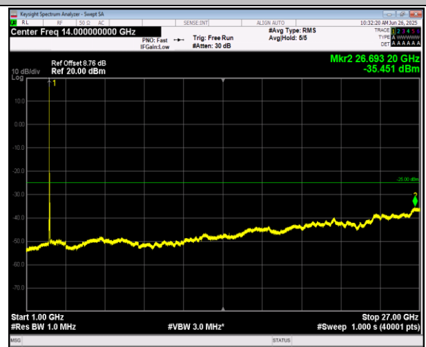
7-7-20MHz-10MHz-16QAM-16QAM-21051-21195-1RB#0-1 RB#49-1000~27000MHz-PASS
