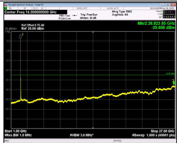
7-7-20MHz-20MHz-16QAM-16QAM-21001-21199-1RB#99- 0RB#0-1000~27000MHz-PASS
