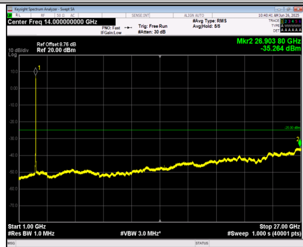
7-7-20MHz-10MHz-16QAM-16QAM-21251-21395-1RB#0-0RB#0-30~1000MHz-PASS RB#0-1000~27000MHz-PASS
