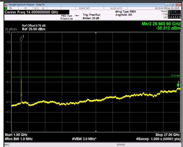
7-7-10MHz-20MHz-16QAM-16QAM-21006-21150-1RB#0-0 RB#0-1000~27000MHz-PASS
