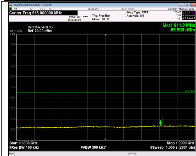
7-7-20MHz-20MHz-QPSK-QPSK-20850-21048-100RB#0-100RB#0-30~1000MHz-PASS
