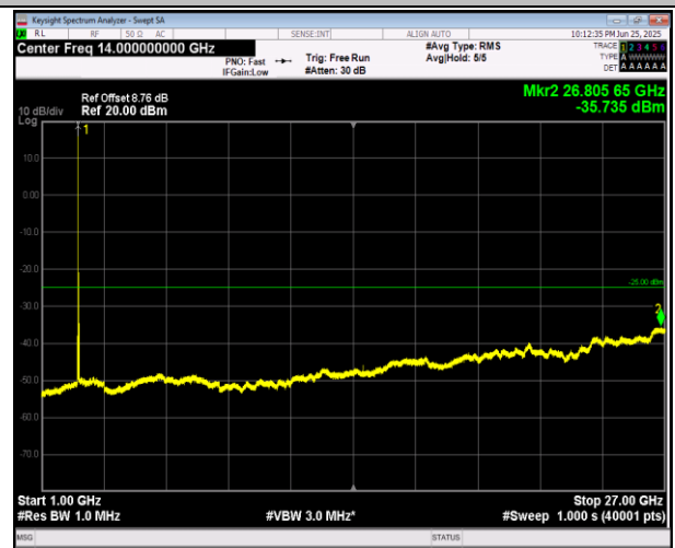
7-7-10MHz-20MHz-16QAM-16QAM-21006-21150-1RB#0-1 RB#99-1000~27000MHz-PASS
