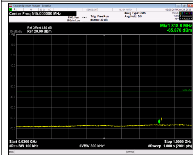
7-7-20MHz-20MHz-16QAM-16QAM-20850-21048-1RB#0-0RB#0-0-30~1000MHz-PASS
