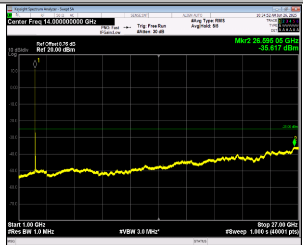
7-7-20MHz-10MHz-16QAM-16QAM-21051-21195-1RB#99- 0RB#0-1000~27000MHz-PASS
