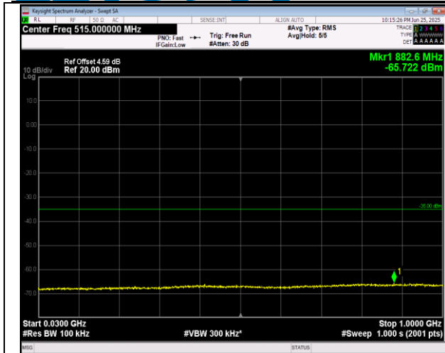
7-7-10MHz-20MHz-16QAM-16QAM-21006-21150-1RB#0 -0RB#0-30~1000MHz-PASS
