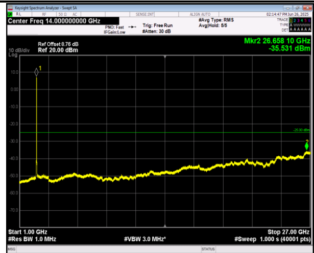
7-7-20MHz-20MHz-16QAM-16QAM-21001-21199-1RB#0-0 RB#0-1000~27000MHz-PASS
