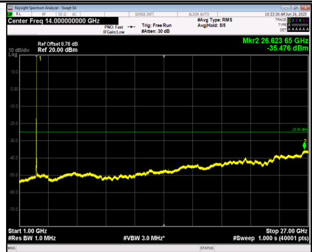
7-7-20MHz-10MHz-16QAM-16QAM-21051-21195-100RB#0 -50RB#0-1000~27000MHz-PASS
