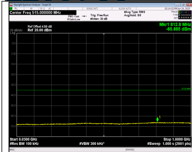
7-7-20MHz-20MHz-16QAM-16QAM-21001-21199-1RB#0 -0RB#0-30~1000MHz-PASS
