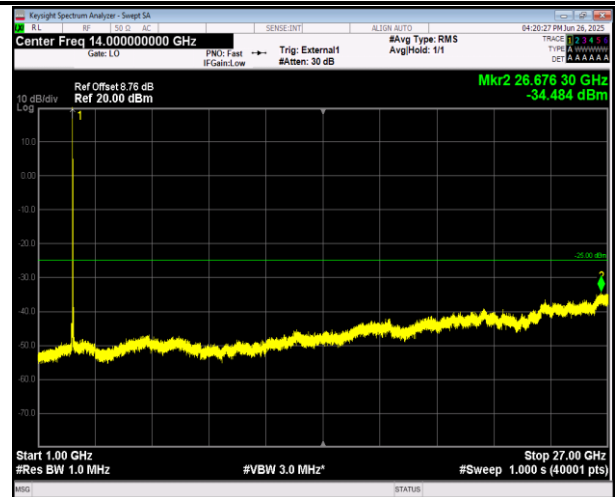
38-38-15MHz-15MHz-QPSK-QPSK-37825-37975-75RB#0- 75RB#0-1000~27000MHz-PASS
