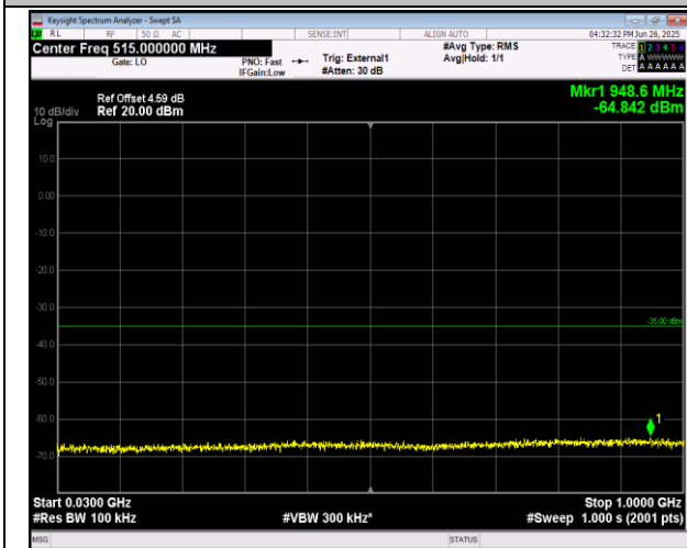
38-38-15MHz-15MHz-QPSK-QPSK-38025-38175-1RB#0- 1RB#74-30~1000MHz-PASS
