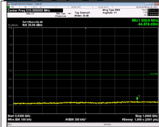
38-38-20MHz-20MHz-16QAM-16QAM-37901-38099-1RB #0-ORB#0-30~1000MHz-PASS
