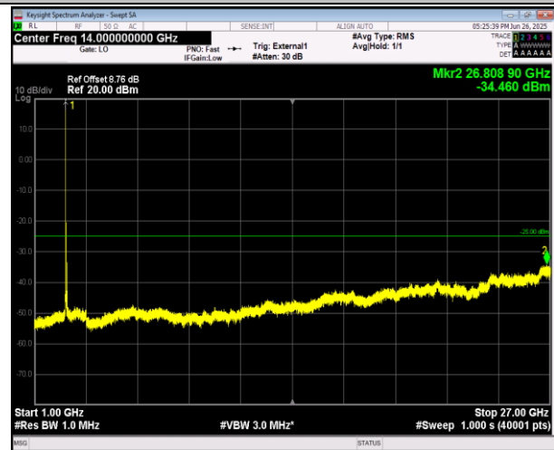
38-38-20MHz-20MHz-16QAM-16QAM-37850-38048-1RB#0-1RB#99-1000~27000MHz-PASS
