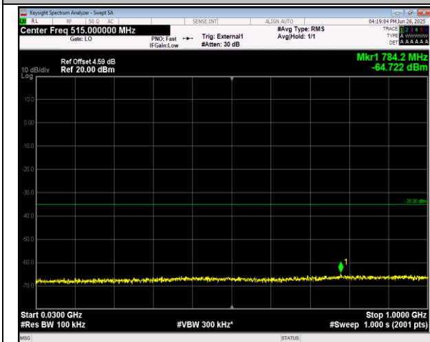
38-38-15MHz-15MHz-16QAM-16QAM-37825-37975-1RB #0-1RB#74-30~1000MHz-PASS
