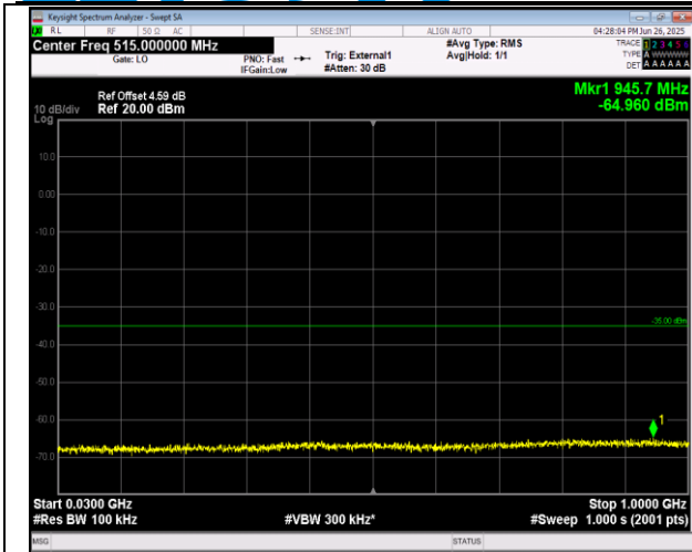
38-38-15MHz-15MHz-16QAM-16QAM-37925-38075-75R B#0-75RB#0-30~1000MHz-PASS
