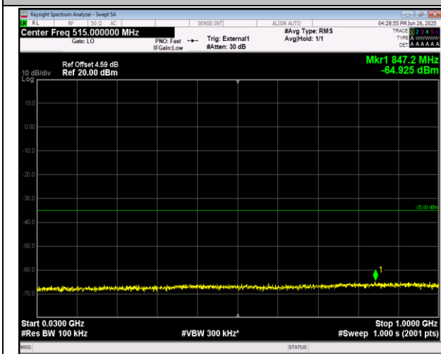
38-38-15MHz-15MHz-QPSK-QPSK-37925-38075-1RB#7-4-0RB#0-30~1000MHz-PASS
