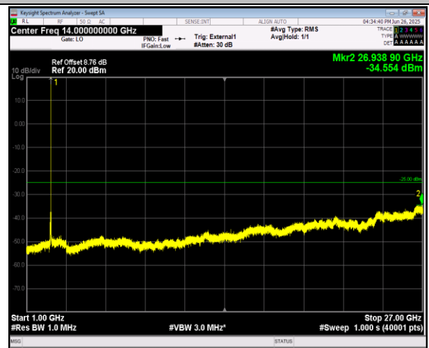
38-38-15MHz-15MHz-QPSK-QPSK-38025-38175-75RB#0- 75RB#0-1000~27000MHz-PASS
