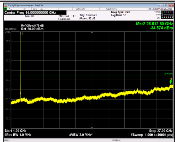
38-38-15MHz-15MHz-16QAM-16QAM-37825-37975-1RB# 0-1RB#74-1000~27000MHz-PASS
