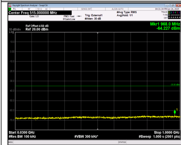
38-38-15MHz-15MHz-QPSK-QPSK-38025-38175-1RB#0- ORB#0-30~1000MHz-PASS
