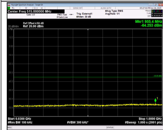
38-38-20MHz-20MHz-16QAM-16QAM-37850-38048-100 RB#0-100RB#0-30~1000MHz-PASS
