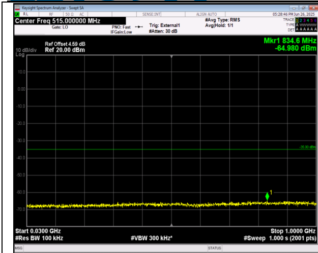
38-38-20MHz-20MHz-16QAM-16QAM-37850-38048-1RB #99-ORB#0-30~1000MHz-PASS
